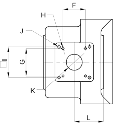
下料口铸件安装尺寸 Installation dimension of material inlet casting
