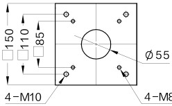
移位料斗安装尺寸 Installation dimension of hopper slider
