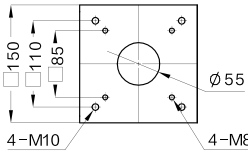
移料料斗安装尺寸 Installation dimension of hopper slider
