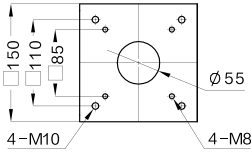
移料斗安装尺寸 Installation dimension of hopper slider
