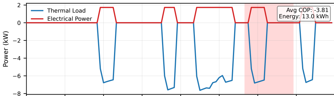
(b) HVAC Performance
