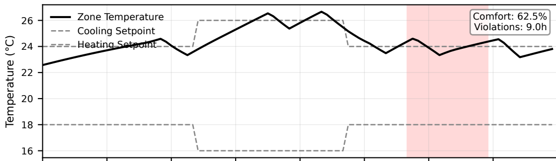
(a) Zone Temperature Control
