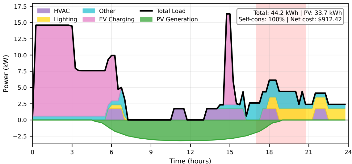
(d) Disaggregated Load Profile
