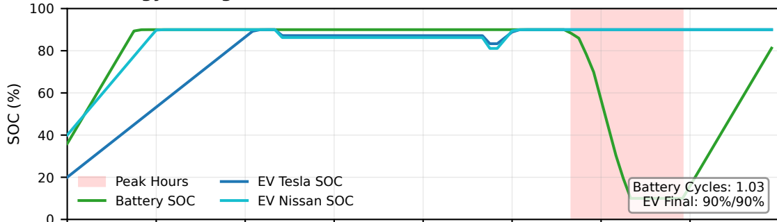
(c) Energy Storage SOC
