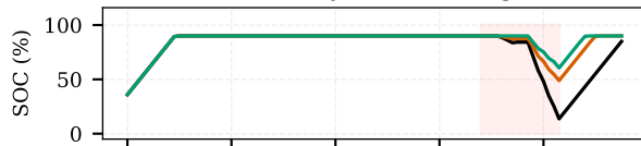
(f) Battery State of Charge
