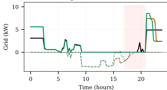
(g) Net Grid Power
