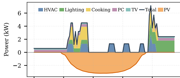
(e) Demand & Generation
