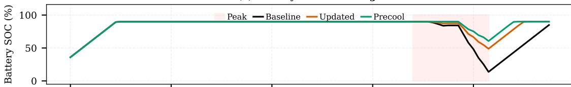
(b) Battery State of Charge
