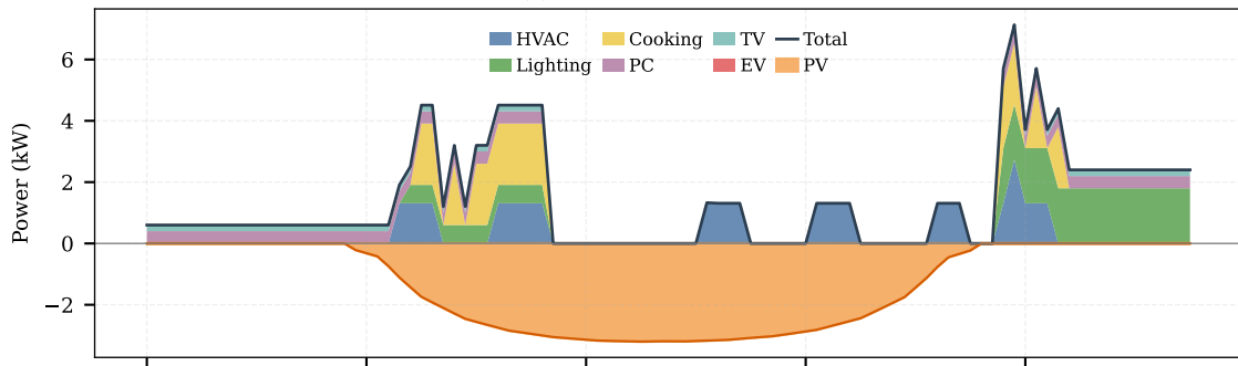
(a) Demand & Generation
