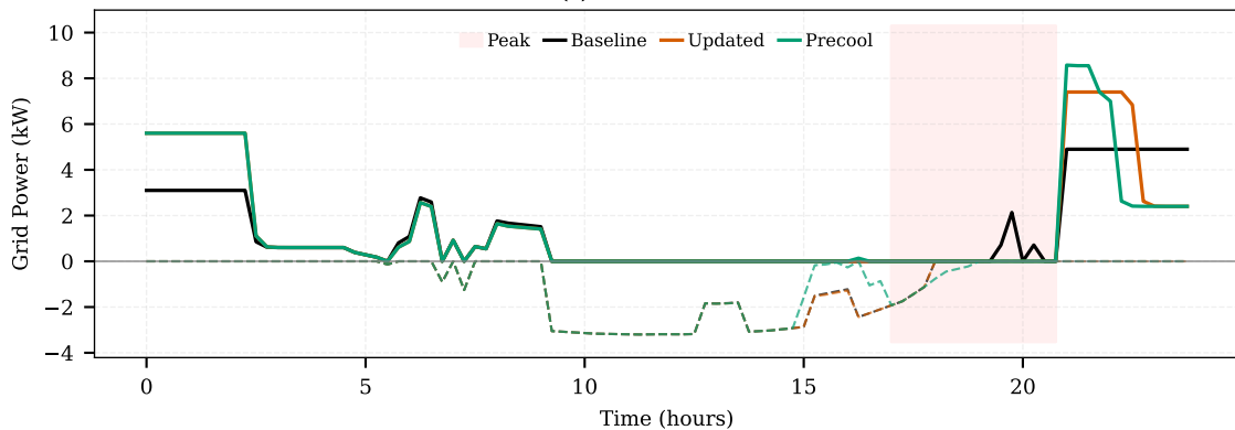
(c) Net Grid Power
