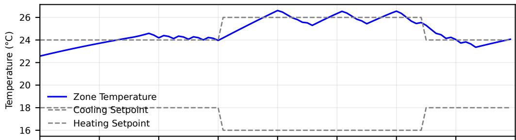
(a) Zone Temperature Control
