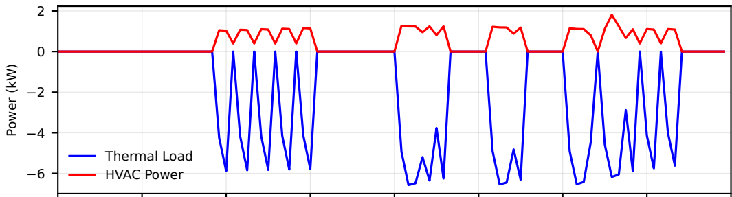
(b) HVAC Performance
