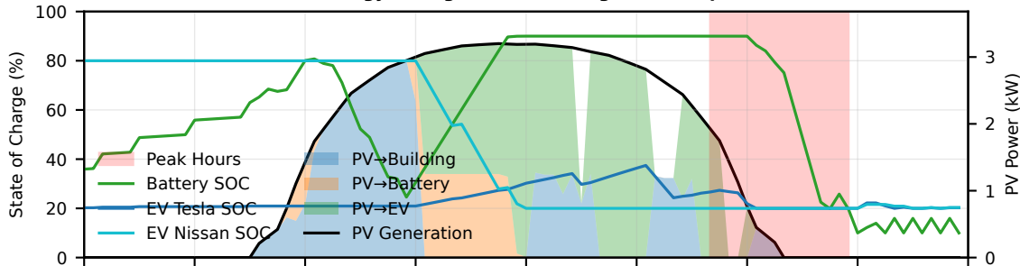
(c) Energy Storage State of Charge & PV Dispatch
