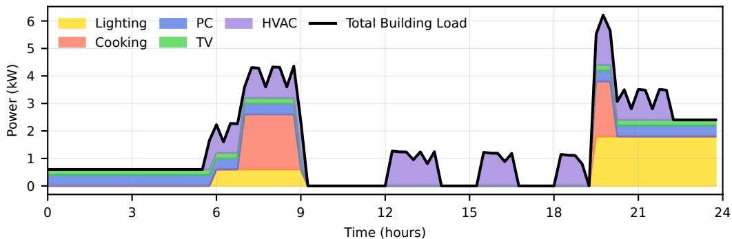
(d) Disaggregated Load Profile
