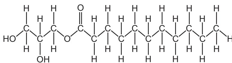
molecule X
