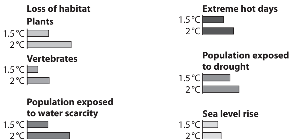
Increasing impacts from 1.5°C to 2°C
