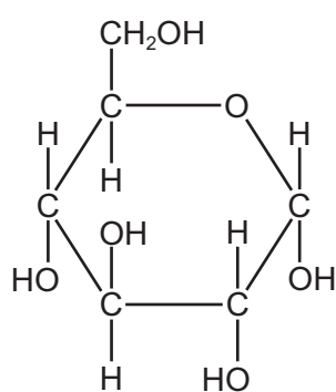
D-glucose
