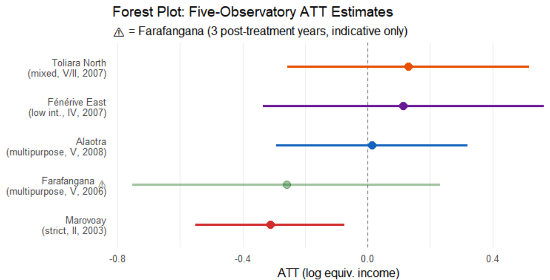
Figure 25.2: Forest plot of average post-treatment ATTs with 95% parametric bootstrap CIs. Farafangana shown at reduced opacity.
