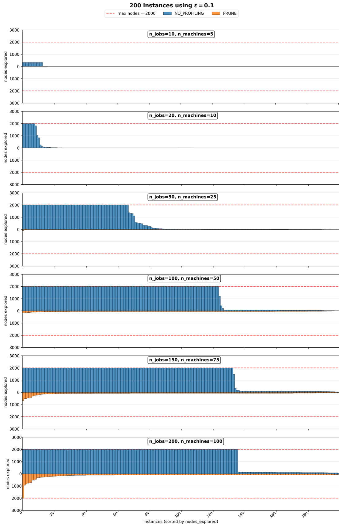
Branch-And-Bound Algorithms as Polynomial-Time Approximation Schemes
