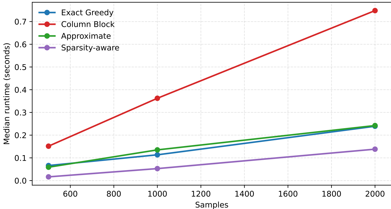
Split-finding runtime on deterministic synthetic data
