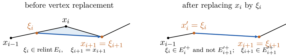
Figure 1: Half-open side membership for the unchanged image vertices in the elementary vertex-replacement pattern. The shaded region is the only part discarded from P ; the blue edge is an actual edge of Q = \lambda P .
