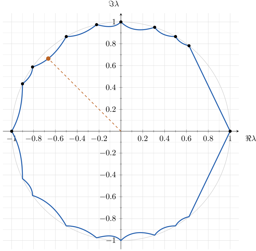
Figure 1: The boundary of \Theta_7 . The thin grey circle is |\lambda| = 1 , and the dashed segment lies on the ray \{te^{3\pi i/4} : t \geq 0\} . Its marked endpoint is \lambda = \rho e^{3\pi i/4} , where \rho is the unique solution of (II.10.2).
