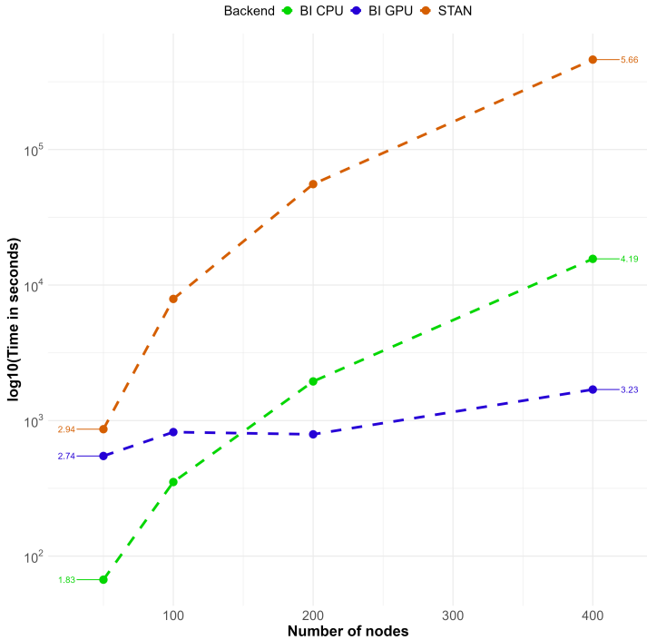
FIGURE 1 (A) Benchmarking runtime performance of STAN and BI (CPU and GPU implementations) for the Social Relations Model (SRM) across networks of varying sizes (50, 100, 200, and 400 nodes). (B) Posterior distributions for model parameters.
