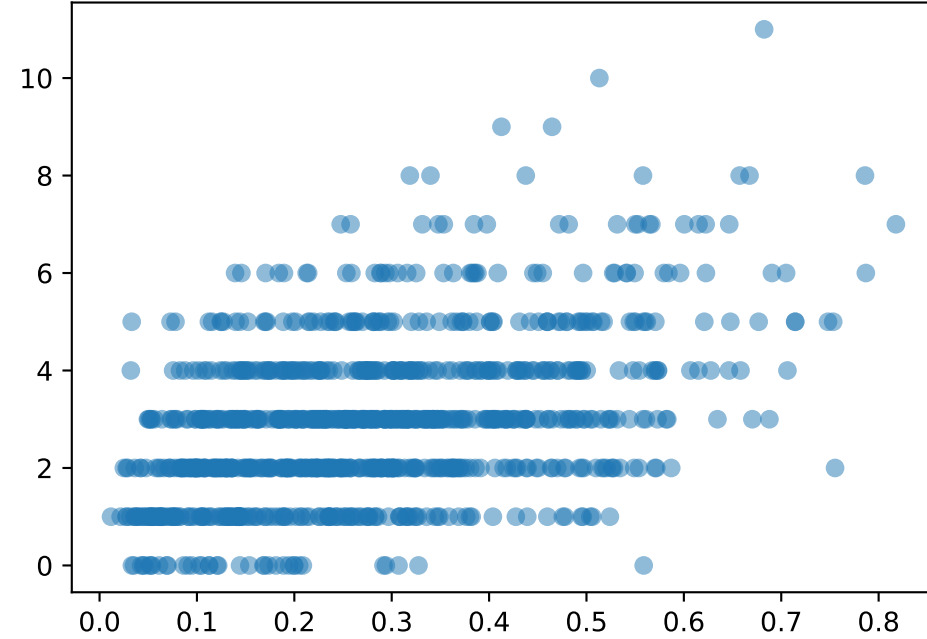
Joint Density Raw Approach Copula (Beta & Poisson)
