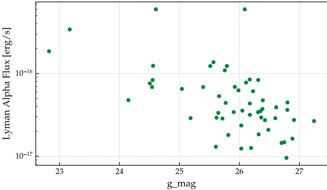
LYA flux vs mag of matched sources
