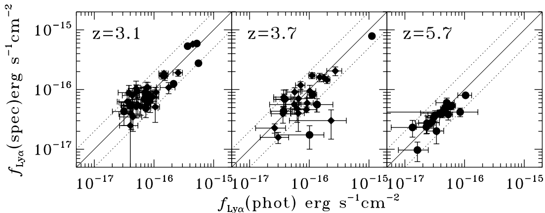
FIG. 15.—Comparison of \text{Ly}\alpha fluxes measured with our images, f_{\text{Ly}\alpha}(\text{phot}) , and spectra, f_{\text{Ly}\alpha}(\text{spec}) , for our LAEs at z = 3.1 (left), 3.7 (middle), and 5.7 (right). The circles and diamonds indicate LAEs with FOCAS and VIMOS spectra, respectively. Since our FOCAS observations used a relatively narrow slit, we apply slit-loss corrections for the \text{Ly}\alpha fluxes of FOCAS. The error bars of circles and diamonds show the ranges of a 95% confidence level. The solid line in each panel presents the equality of f_{\text{Ly}\alpha}(\text{phot}) and f_{\text{Ly}\alpha}(\text{spec}) . We plot dotted lines for the differences from the equality by a factor of 2.
