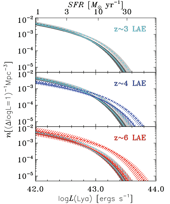
FIG. 21.—Inferred intrinsic Ly \alpha luminosity functions (LFs), together with the best-estimate apparent Ly \alpha LFs. Dashed- and solid-line curves are the intrinsic and apparent Ly \alpha LFs, respectively. Cyan, blue, and red curves denote for LFs at z = 3.1 (top), 3.7 (middle), and 5.7 (bottom), respectively. Cyan lines are repeatedly plotted in each panel for comparison. Light gray and gray shades around cyan lines indicate 1 \sigma errors of intrinsic and apparent Ly \alpha LFs at z = 3.1 . Areas of vertical and hatched lines are the same, but for z = 3.7 (blue) and 5.7 (red) in the middle and bottom panels, respectively.
