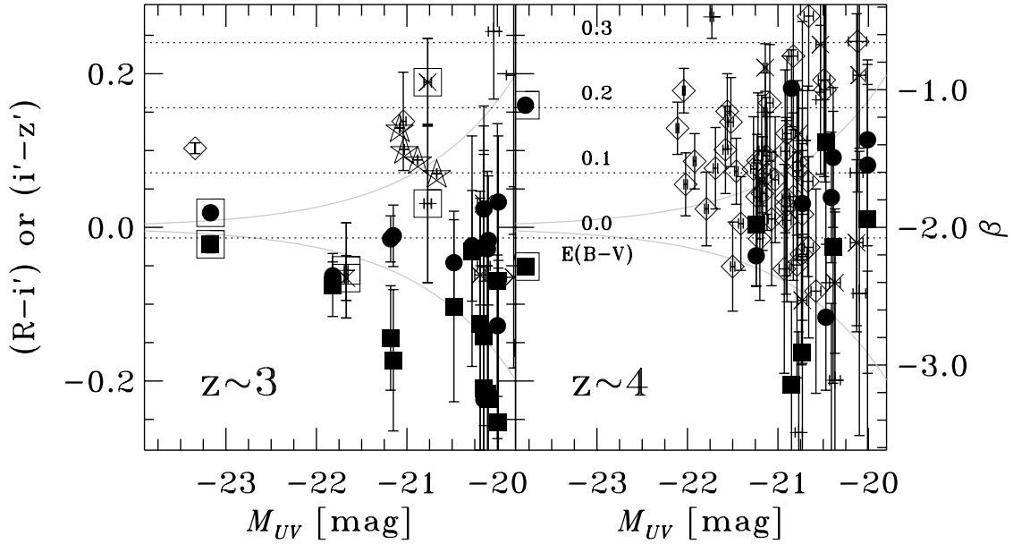
FIG. 26.—UV-continuum color as a function of UV magnitude at z \sim 3 (left) and z \sim 4 (right). The filled squares indicate a i' - z' color of our LAEs at z = 3.1 and 3.7 from our spectroscopic samples. The filled circles are the same, but for a R - i' color. For confused LAEs whose photometry appears to be contaminated by neighboring objects in a broadband image, we use plus signs and crosses instead of filled squares and circles, respectively. We mark LAEs with AGN activities with a large open square. The diamonds plot i' - z' colors of spectroscopically identified LBGs (Yoshida et al. 2006). The star marks in the left panel represent the average colors of LBGs obtained by Shapley et al. (2003). We estimate i' - z' colors of the Shapley et al. data with E(B - V) and eq. (12). The vertical axis on the right side shows the UV-slope index, \beta , that corresponds to i' - z' colors at z \sim 4 . Note that this \beta is based on the original definition (see Calzetti 2001), which is different from \beta_{\text{iz}} defined by Ouchi et al. (2004a). The difference of \beta values between R - i' and i' - z' colors is only \lesssim 7\% in the color range of -0.3 to 0.3 . The E(B - V) values corresponding to the UV colors are indicated with dotted lines. The gray curves represent the size of \pm 1 \sigma error for a continuum-flat ( f_{\nu} = \text{const} ) object.
