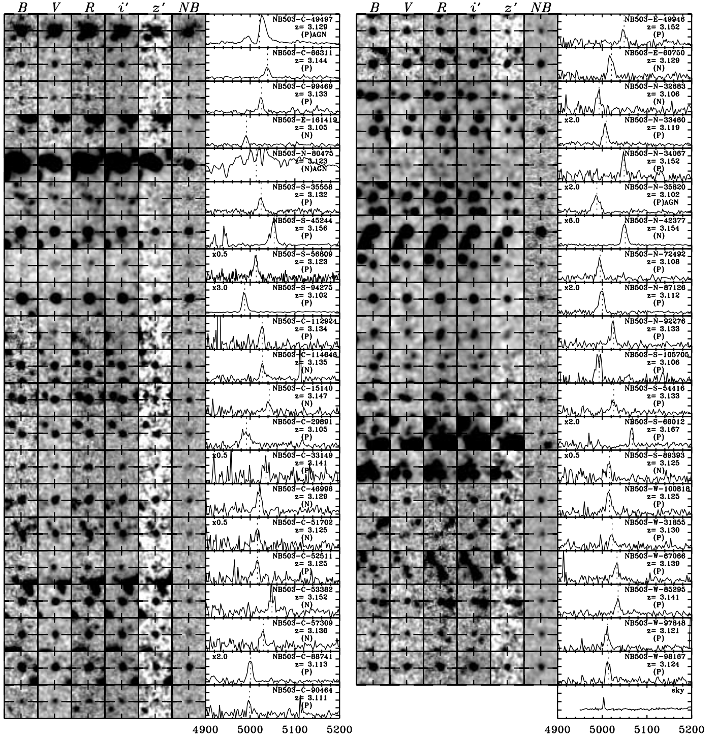
FIG. 3.—Spectra and snapshots of our z = 3.1 LAEs. Each object has a spectrum on the right and snapshots of B , V , R , i' , z' , and NB503 images on the left. Each snapshot is presented in a 6'' \times 6'' box. In the panel of spectrum, the tick of y -axis is marked in 2.5 \times 10^{-18} \text{ ergs s}^{-1} \text{ cm}^{-2} \text{ \AA}^{-1} ; for panels in which a factor is shown in the top left corner, multiply the scale by this factor to obtain a correct scale. The wavelength (in x -axis) is in unit of angstroms. The object name and redshift (+AGN classification, if any) are presented in the right corner of each spectrum panel. “P” (“N”) in parentheses indicates that the object is (or is not) selected with the color criteria and included in our photometric sample (§ 3.1). The vertical dotted lines mean the center of the emission line. The right bottom panel shows a typical spectrum of the sky background with an arbitrary normalization.
