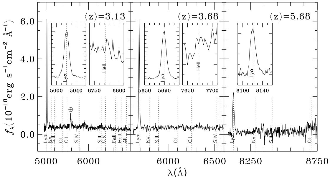
FIG. 27.—Composite spectra of our LAEs at \langle z \rangle = 3.13 (left), 3.68 (middle), and 5.68 (right). The dotted lines indicate the wavelengths of interstellar absorption from star formation or high ionized emission lines from AGN activities. The plots of spectrum are magnified in the inset boxes for wavelength ranges of \text{Ly}\alpha (left) and \text{He II} (right). For the \langle z \rangle = 5.68 LAE, we only show the inset box of \text{Ly}\alpha , since our spectrum does not cover the wavelength of \text{He II} emission for z = 5.7 objects.
