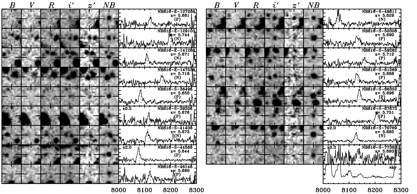
FIG. 5.—Same as Fig. 3, but for our z = 5.7 LAEs. The ticks of the y-axis in a spectrum panel are marked in 0.5 \times 10^{-18} \text{ ergs s}^{-1} \text{ cm}^{-2} \text{ Å}^{-1} .
