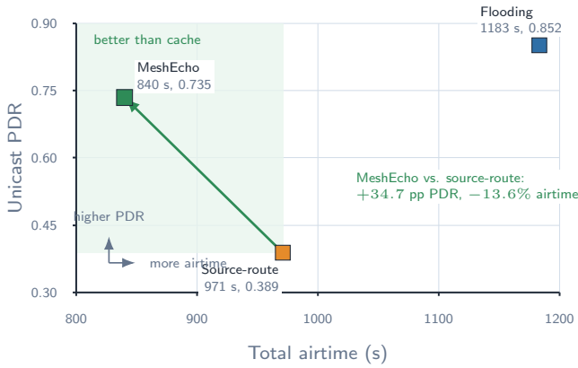
Fig. 4. Mixed-traffic reliability-airtime tradeoff under the evaluated protocol budgets. MeshEcho moves the source-route operating point toward higher delivery with lower airtime, but the end-to-end difference includes bounded recovery not available to the fixed baselines.
