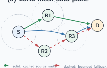
(a) LoRa mesh data plane
