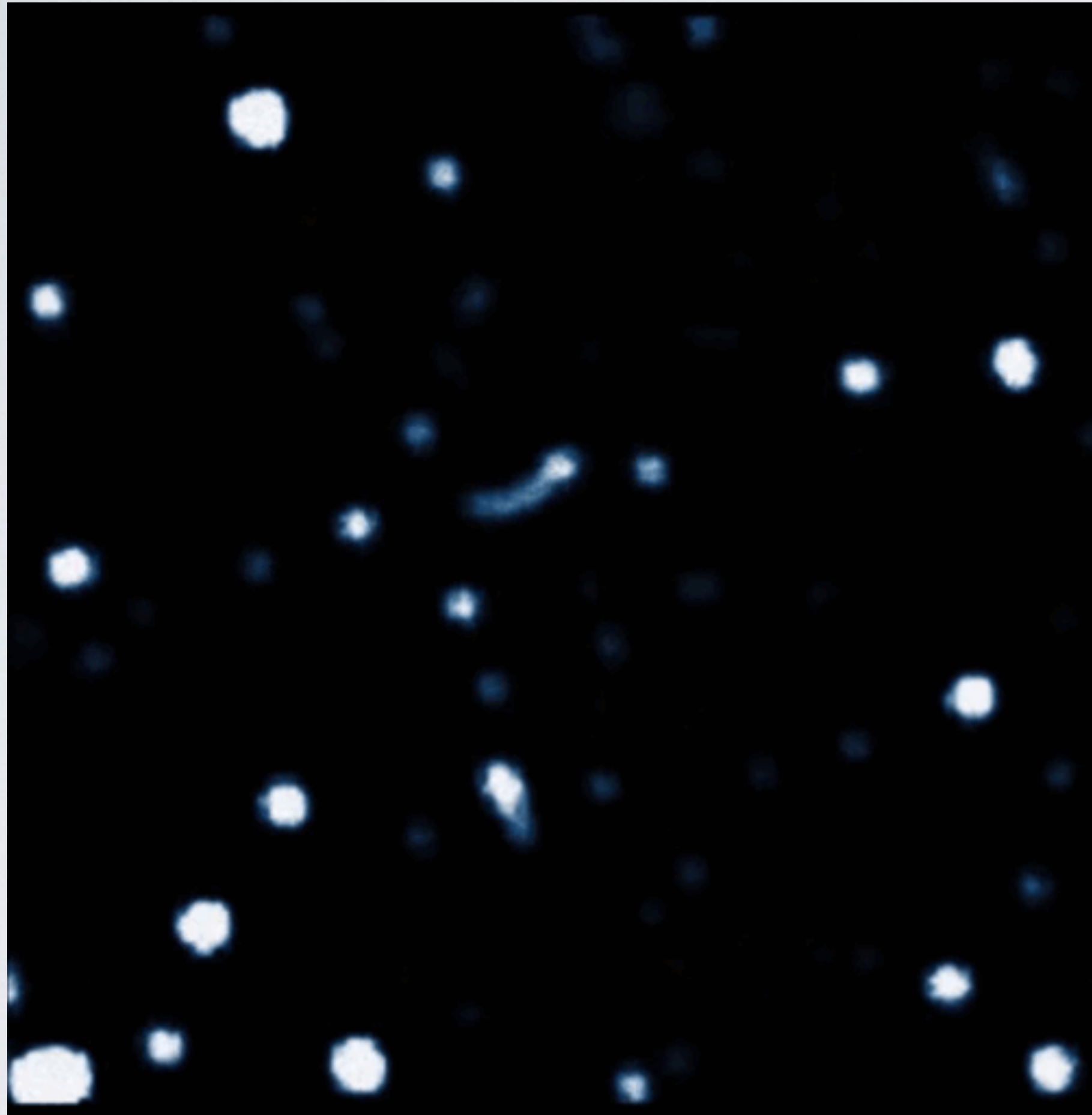
Stars circa 1.19 billion km away from black hole (1700 solar radii)
