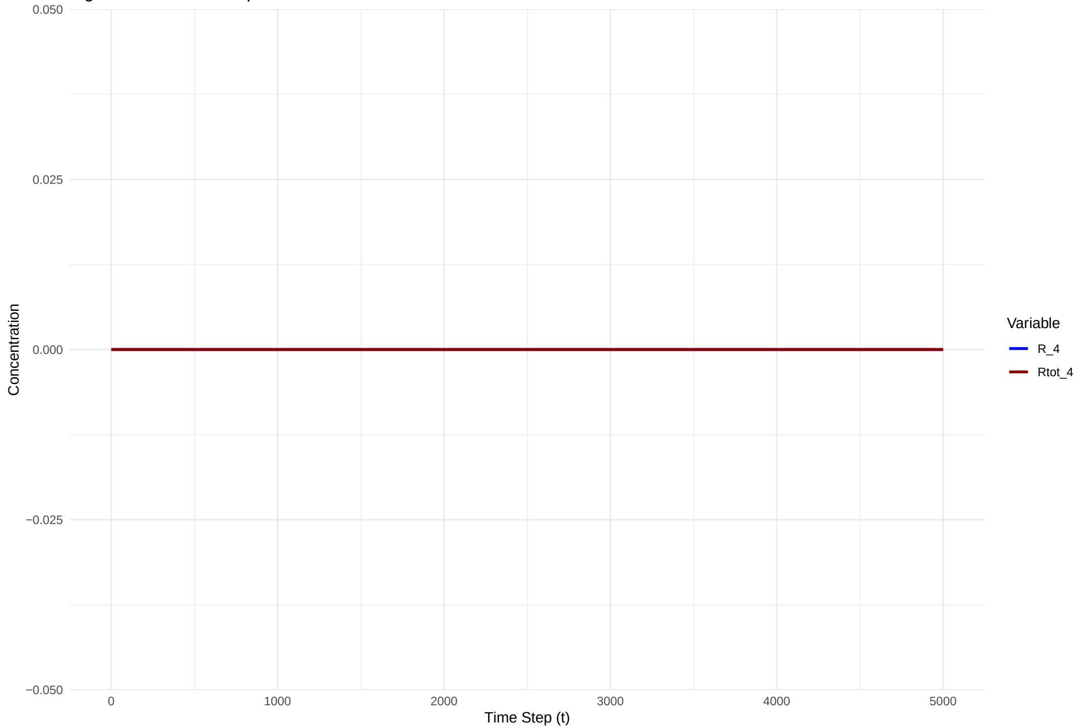
Figure 1 Evolution of Species R 4
