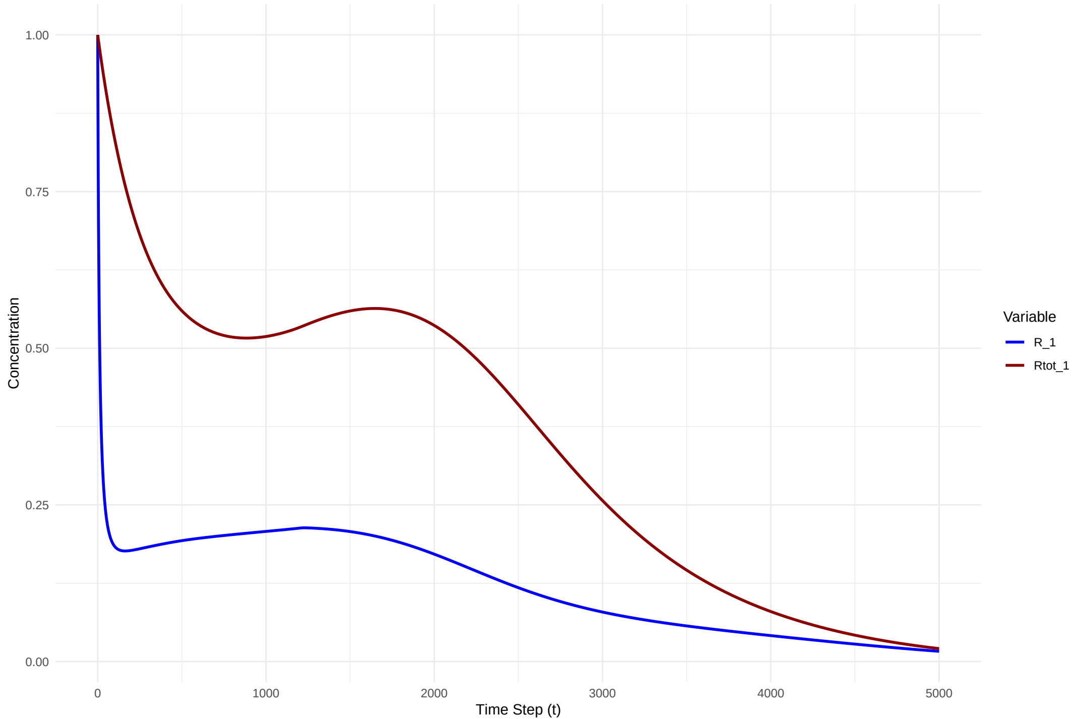
Figure 1 Evolution of Species R 1
