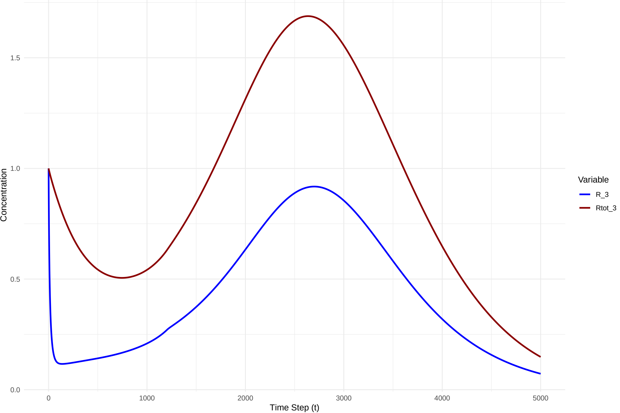
Figure 1 Evolution of Species R 3
