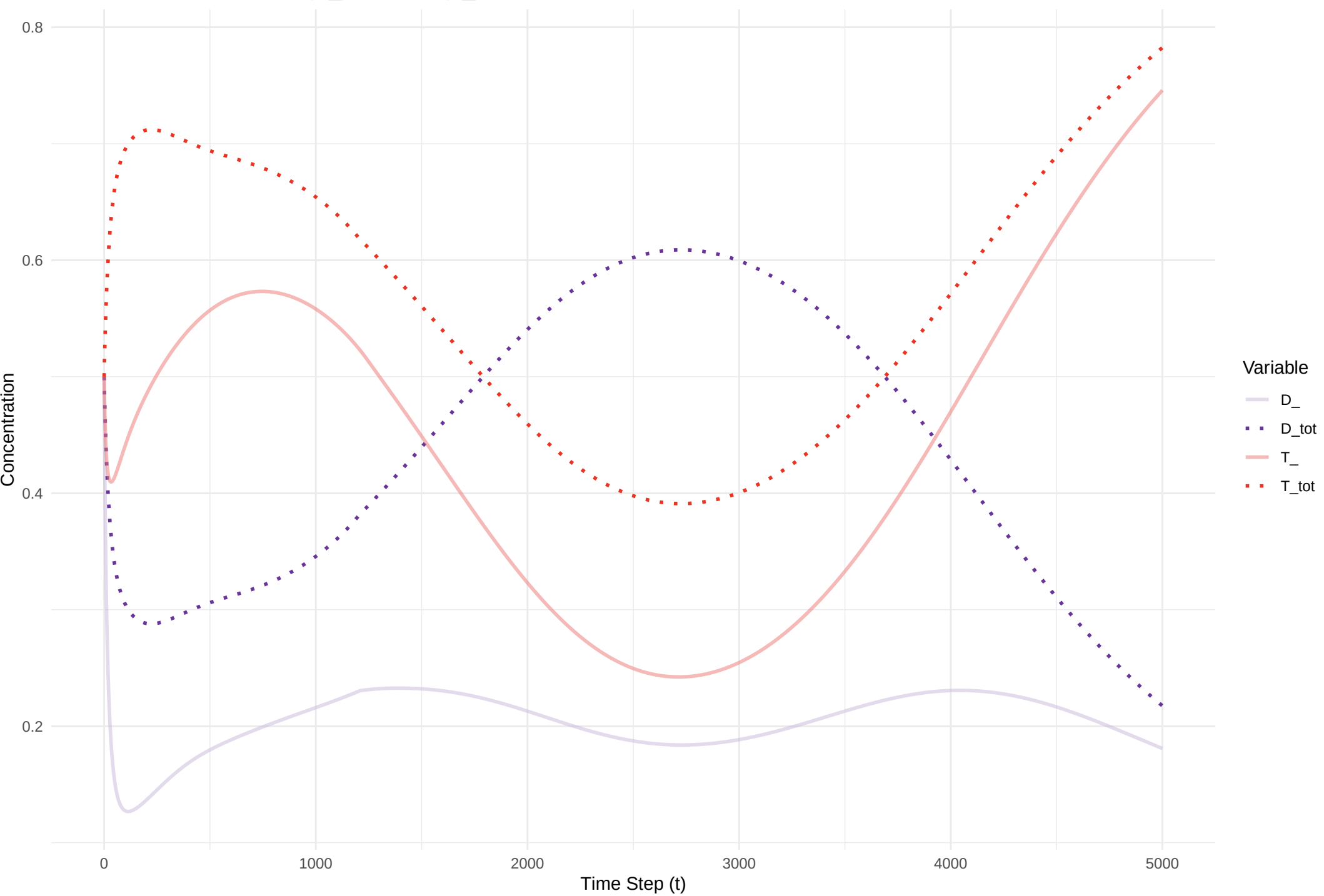
Figure 1 Evolution of ADP (D_) and ATP (T_)
