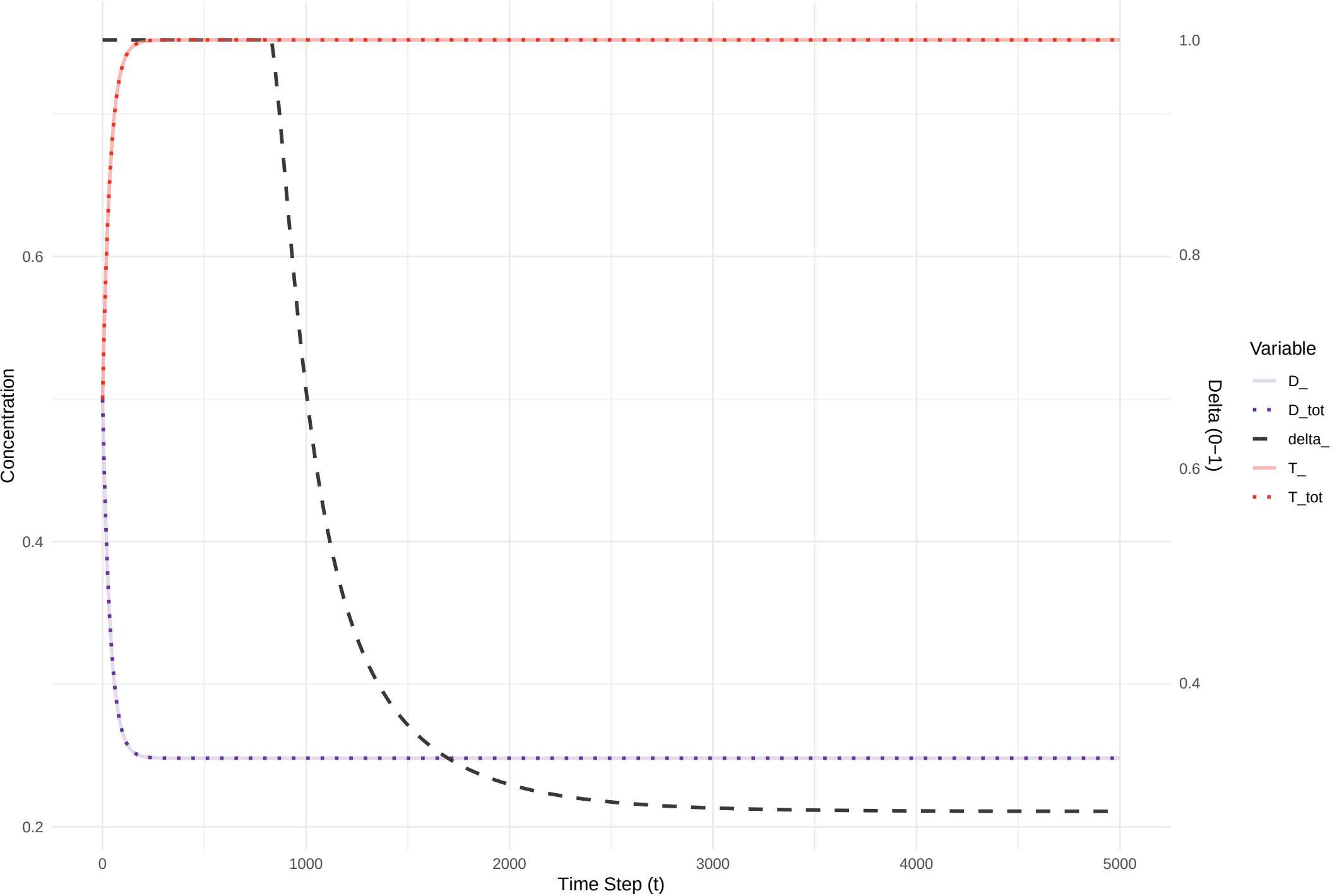
Figure 2 Evolution of ADP ( D_- ), ATP ( T_- ), and \delta (rhs)
