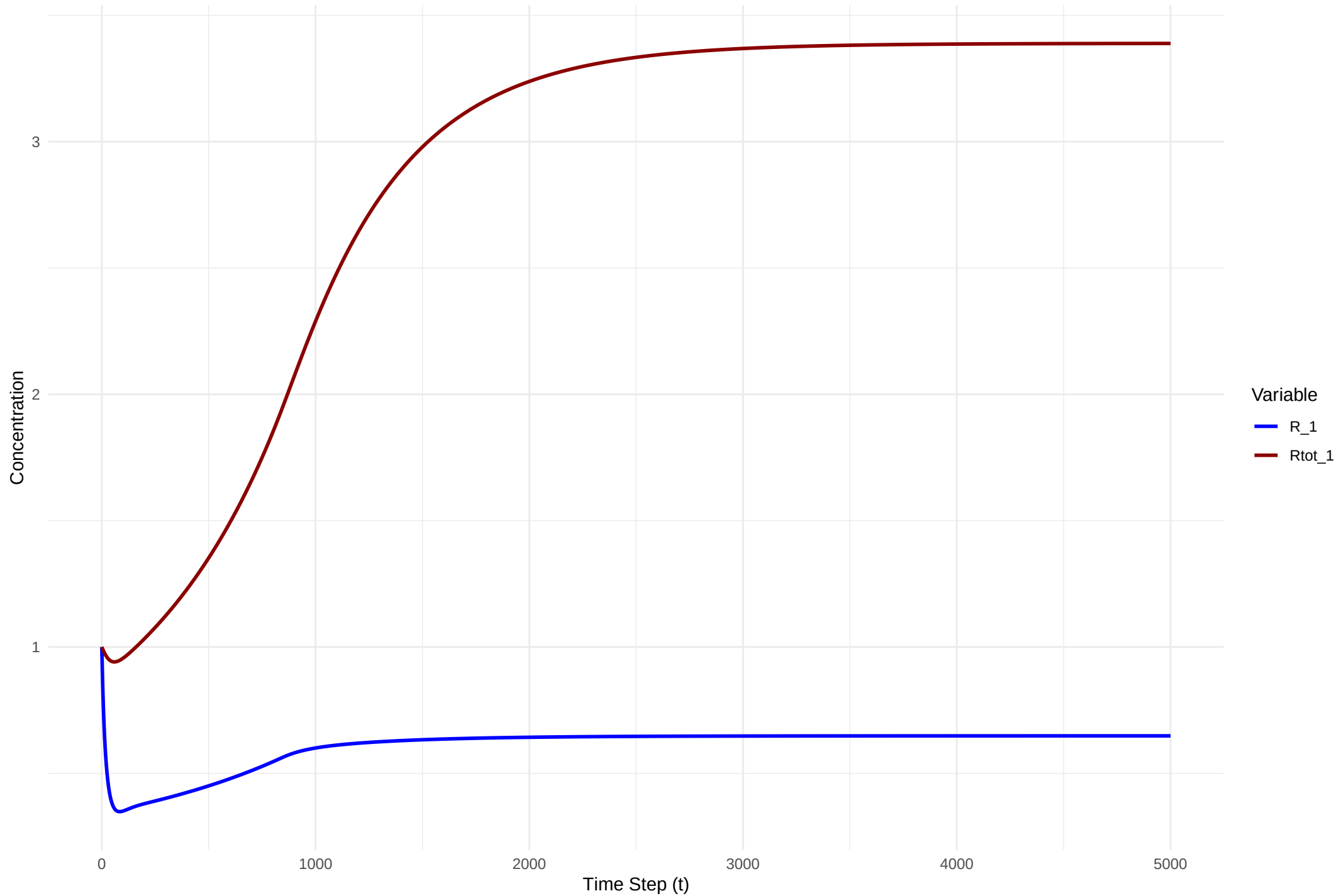
Figure 2 Evolution of Species R 1
