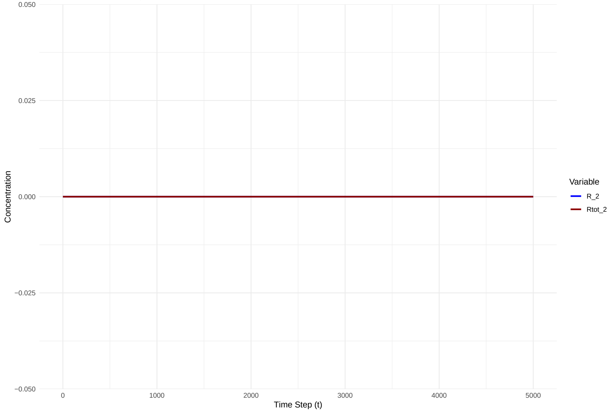
Figure 2 Evolution of Species R 2
