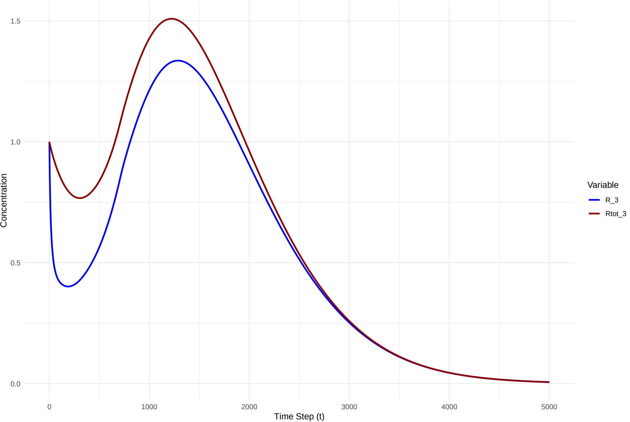
Figure 5 Evolution of Species R 3
