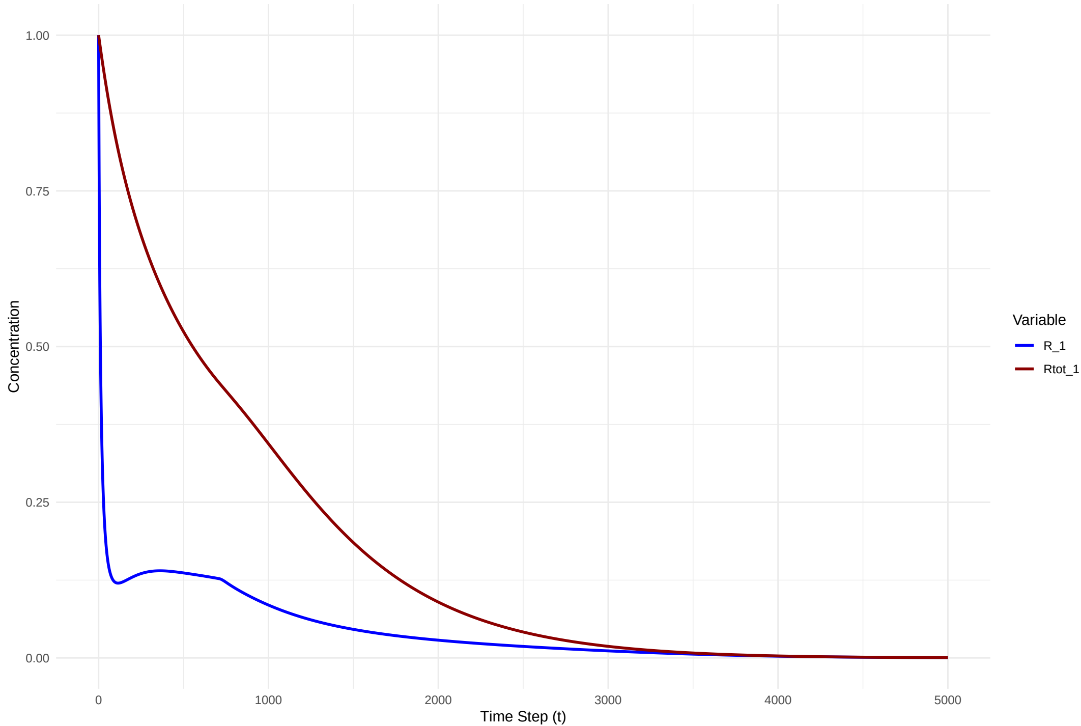
Figure 5 Evolution of Species R 1
