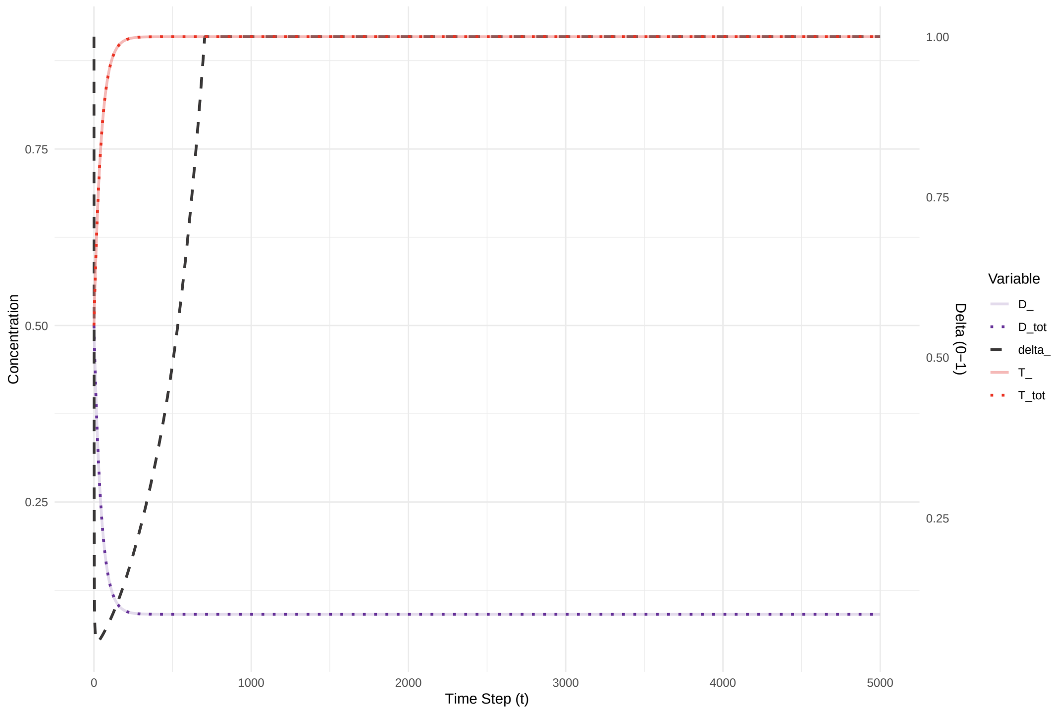
Figure 5 Evolution of ADP ( D_- ), ATP ( T_- ), and \delta_- (rhs)
