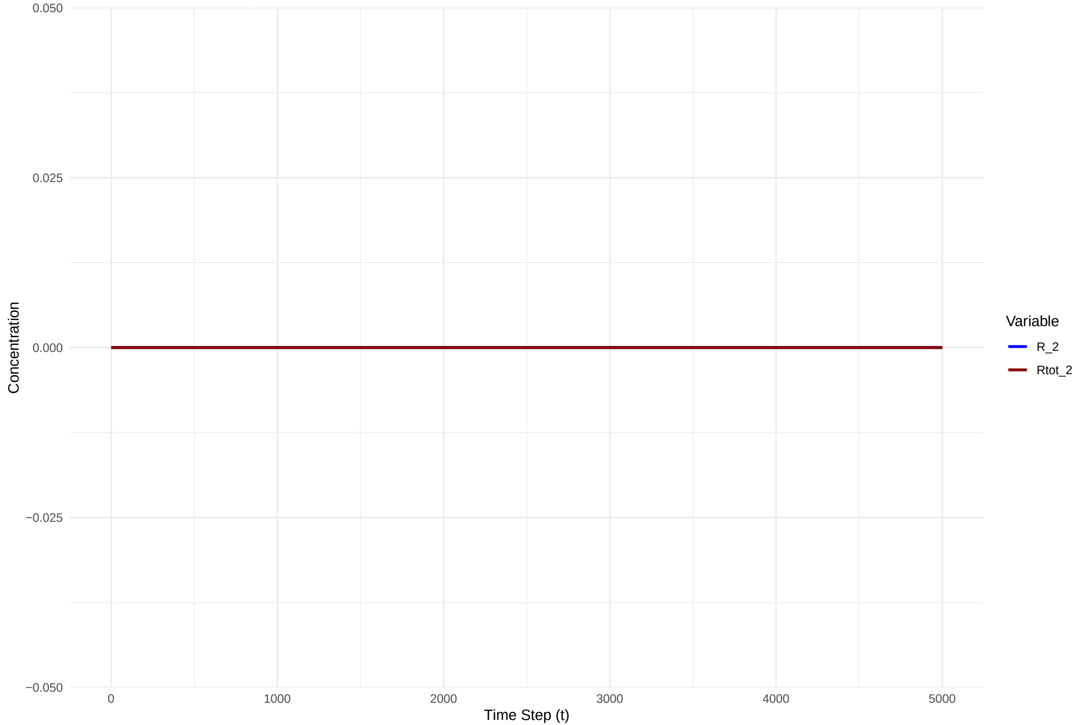
Figure 5 Evolution of Species R 2
