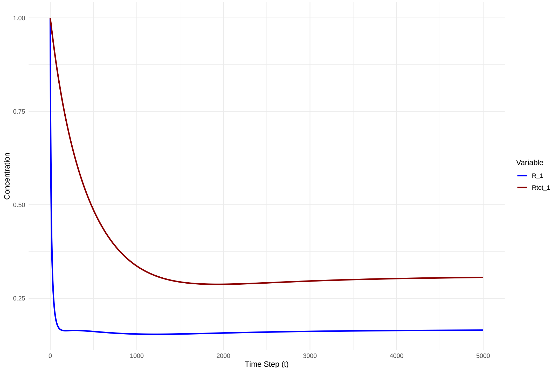
Figure 6 Evolution of Species R 1
