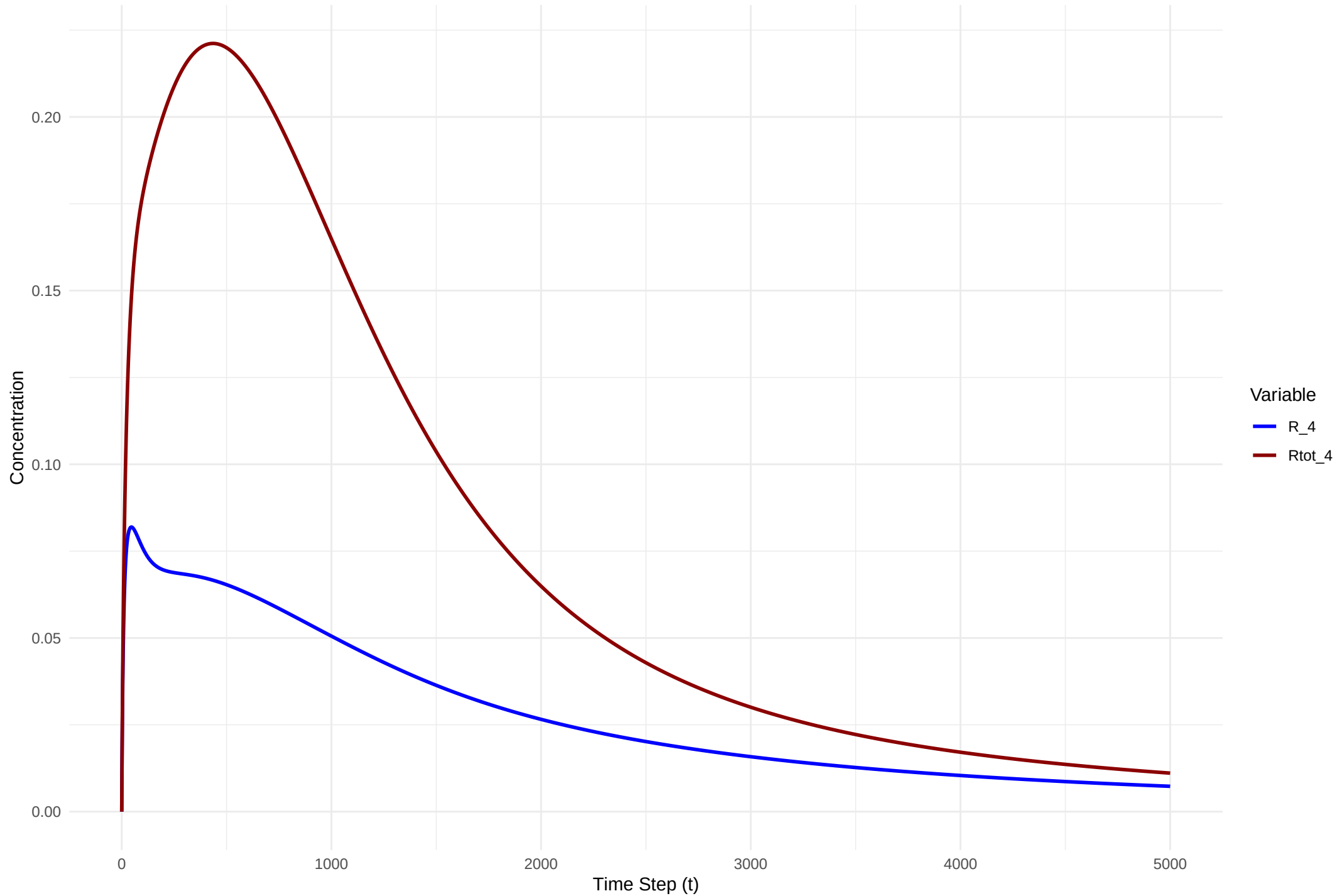
Figure 6 Evolution of Species R 4
