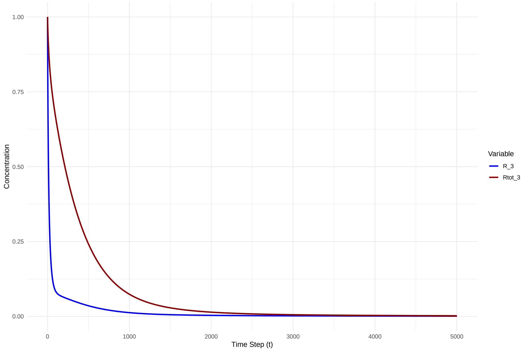
Figure 6 Evolution of Species R 3
