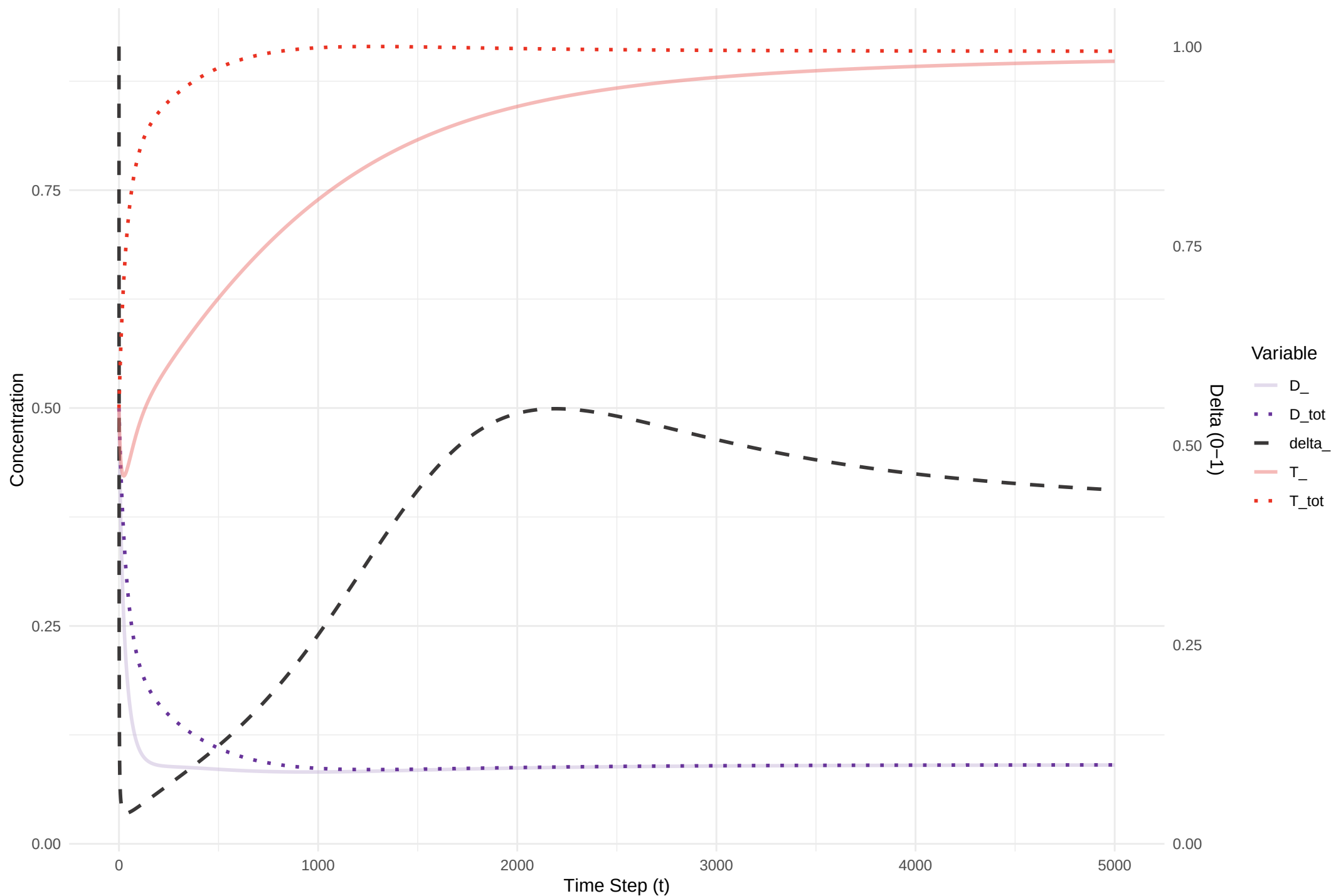
Figure 6 Evolution of ADP ( D_- ), ATP ( T_- ), and \delta_- (rhs)
