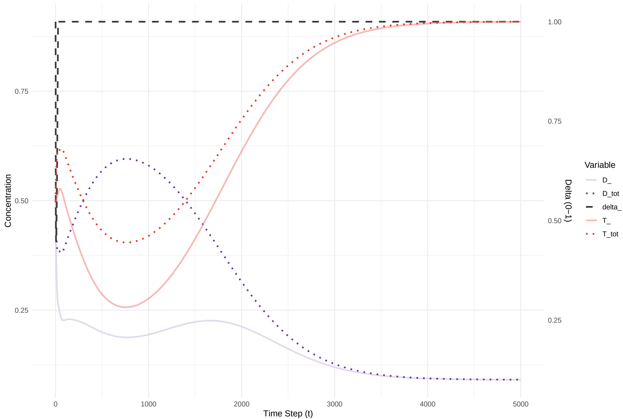
Figure 8 Evolution of ADP ( D_- ), ATP ( T_- ), and \delta_- (rhs)
