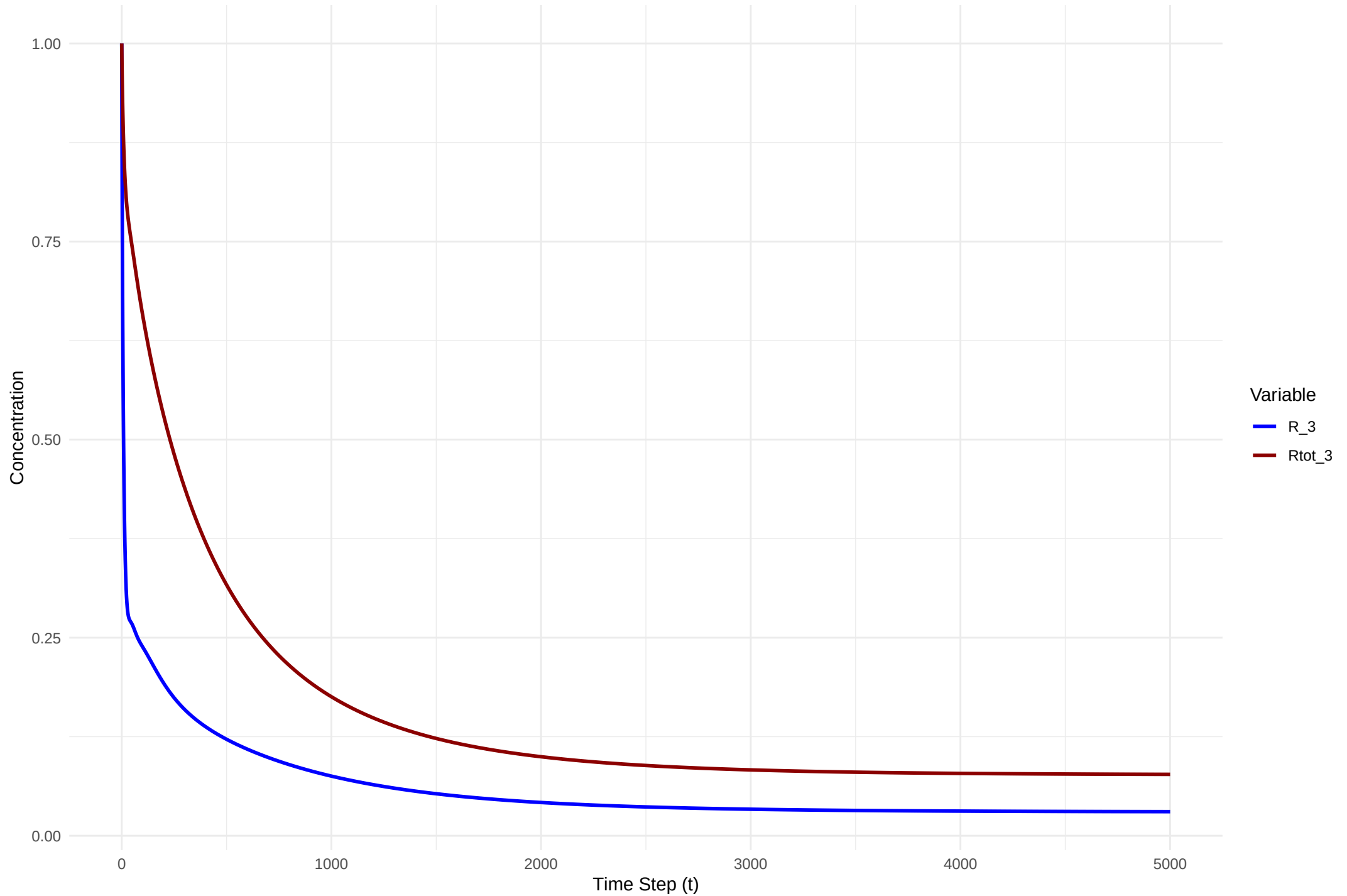
Figure 9 Evolution of Species R 3
