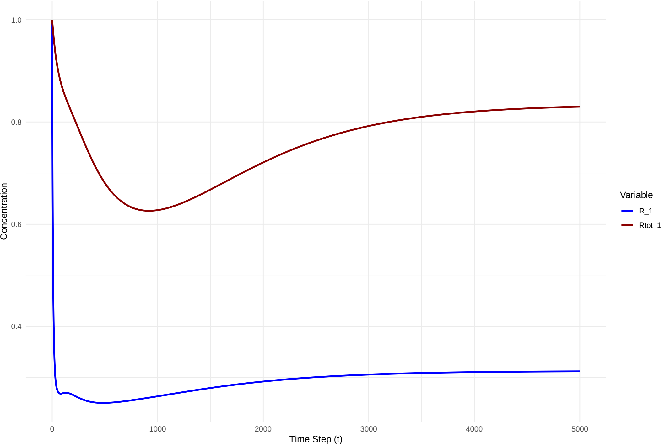
Figure 9 Evolution of Species R 1
