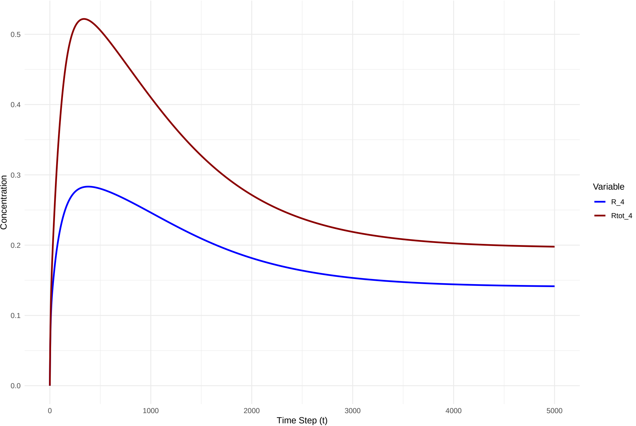
Figure 9 Evolution of Species R 4
