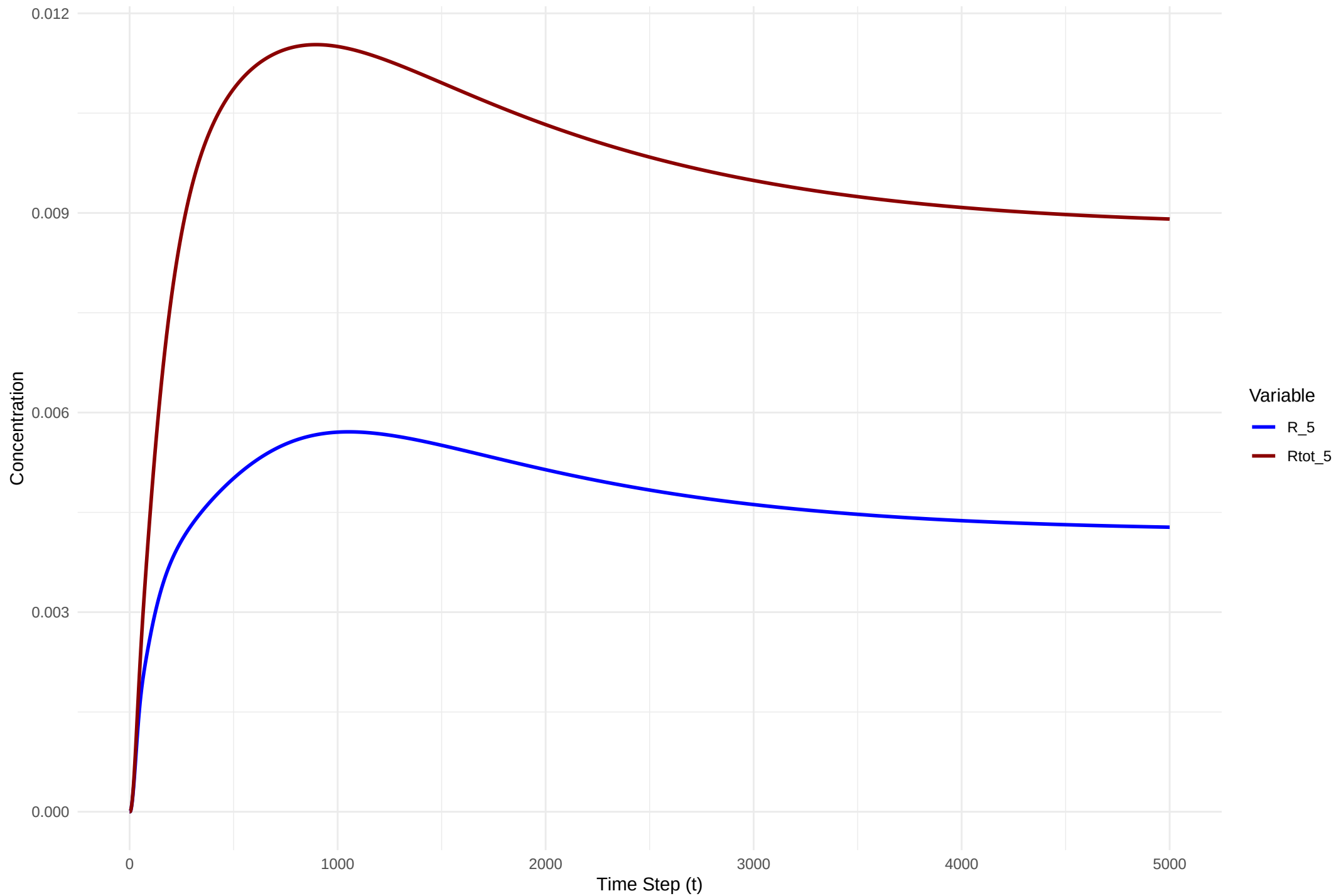
Figure 9 Evolution of Species R 5
