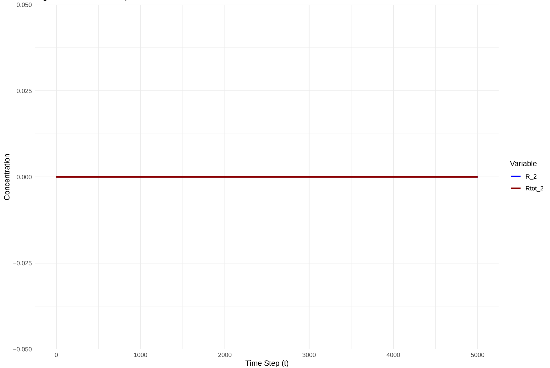
Figure 9 Evolution of Species R 2
