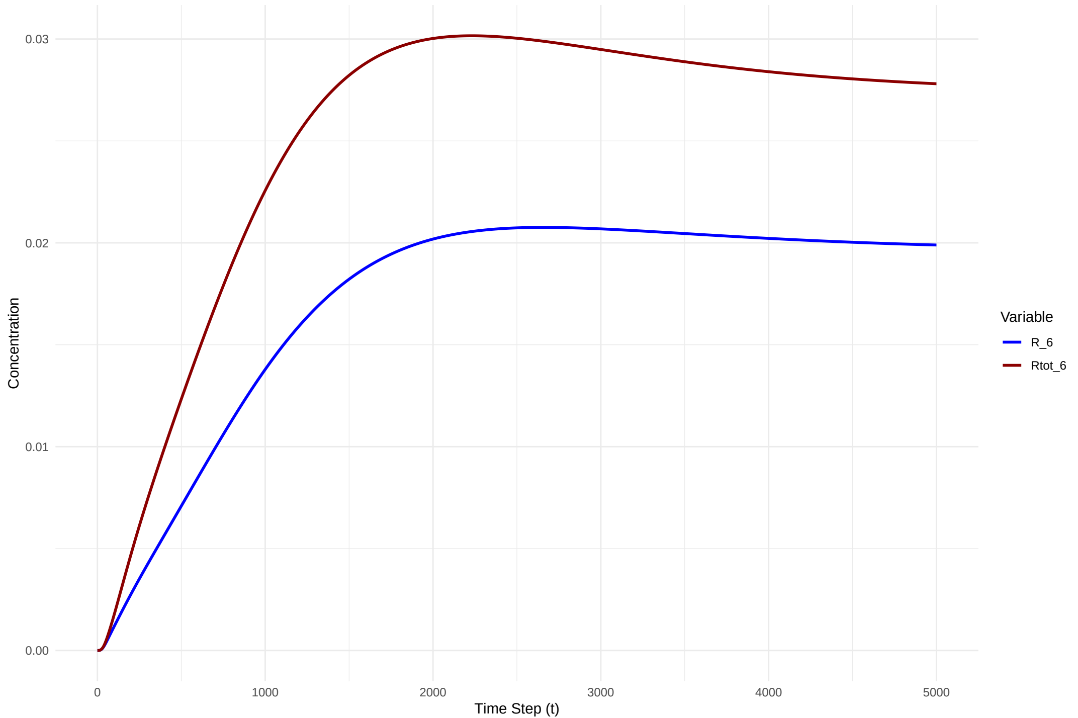
Figure 9 Evolution of Species R 6
