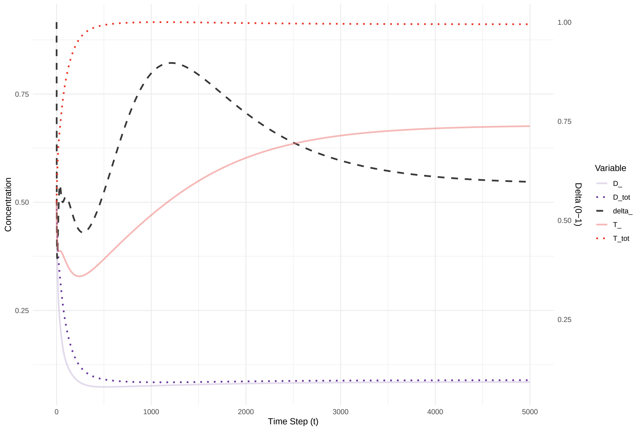
Figure 9 Evolution of ADP ( D_- ), ATP ( T_- ), and \delta_- (rhs)
