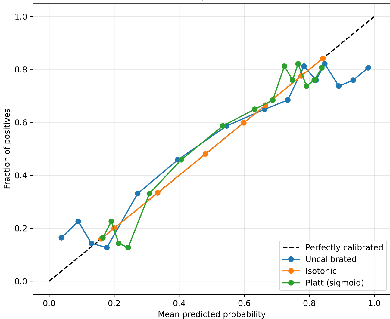
Calibration plot (validation)
