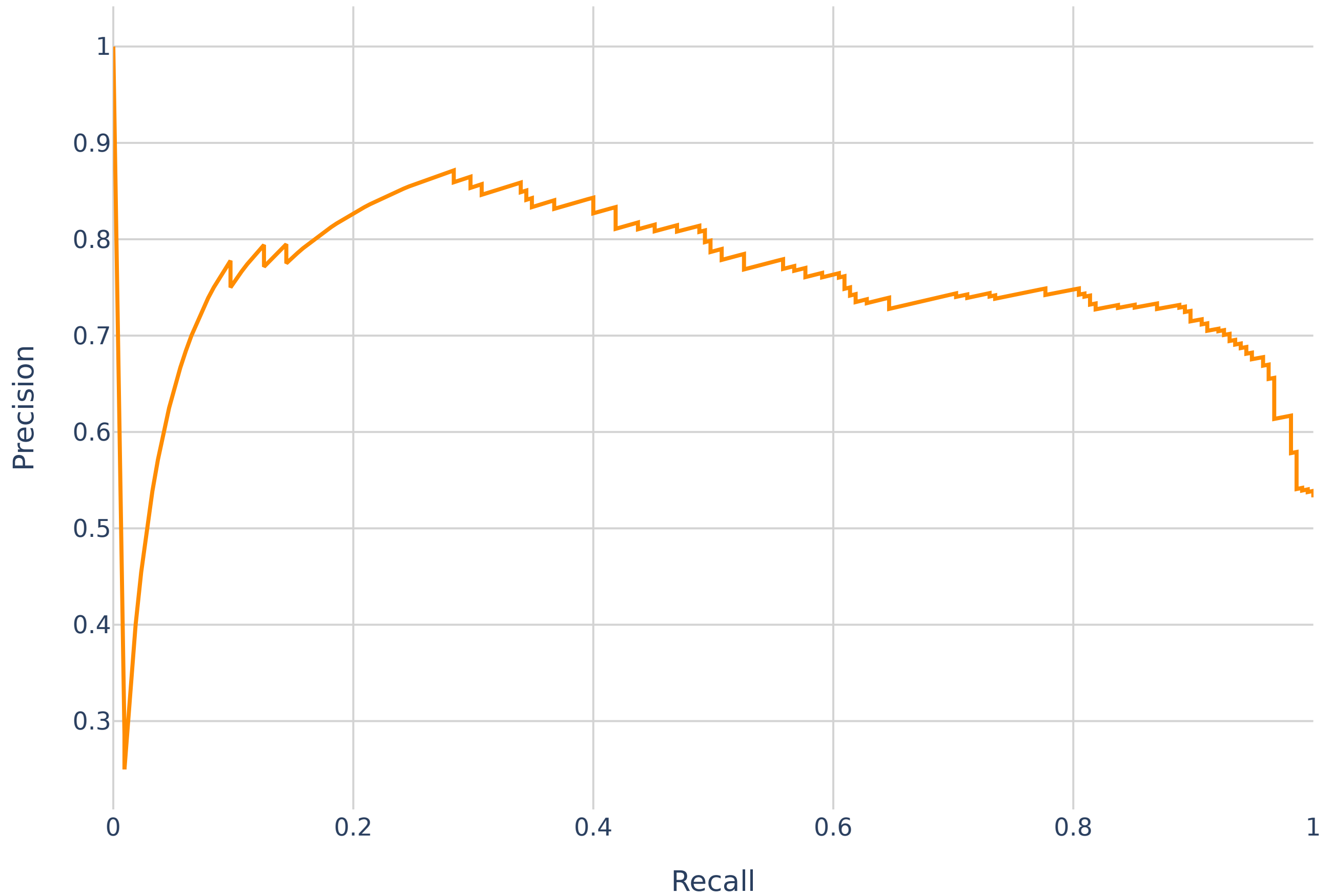
BIMCV Validation - Single model - Precision-Recall Curve
