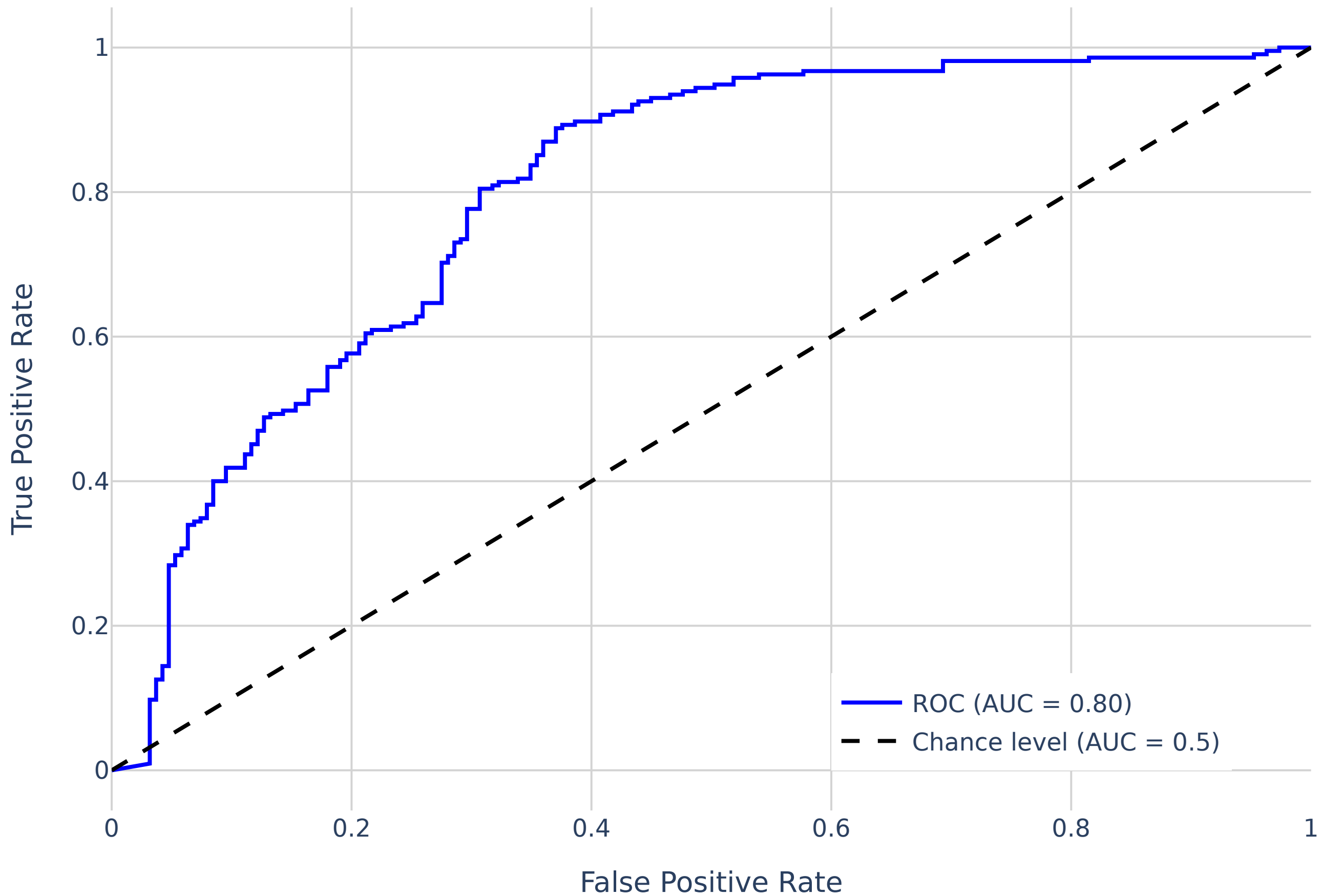
BIMCV Validation - Single model - ROC Curve
