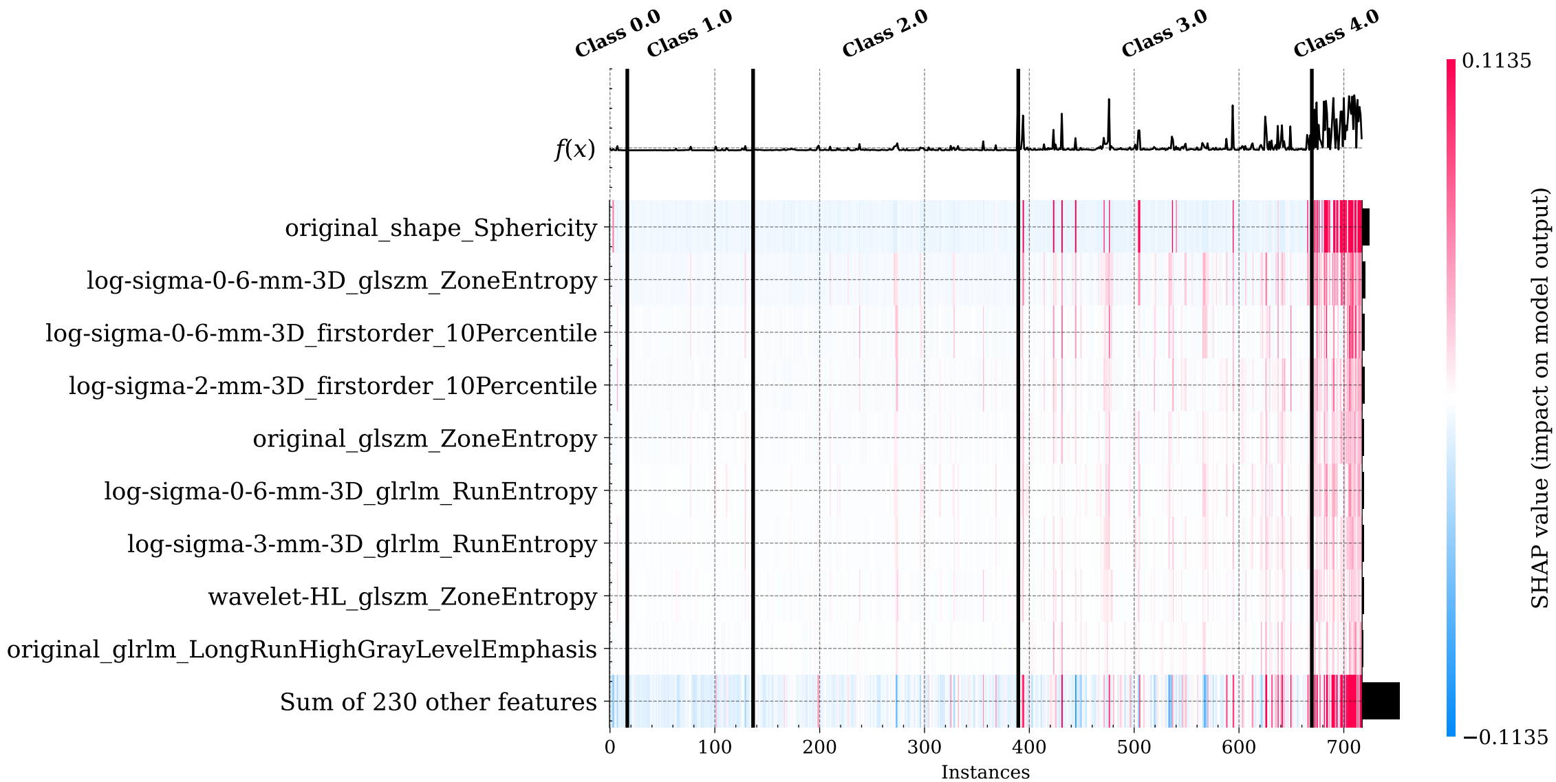
SHAP Heatmap - Class 4 vs All
