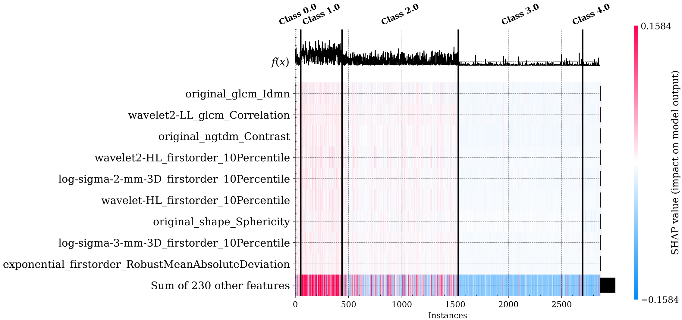
SHAP Heatmap - Class 1 vs All
