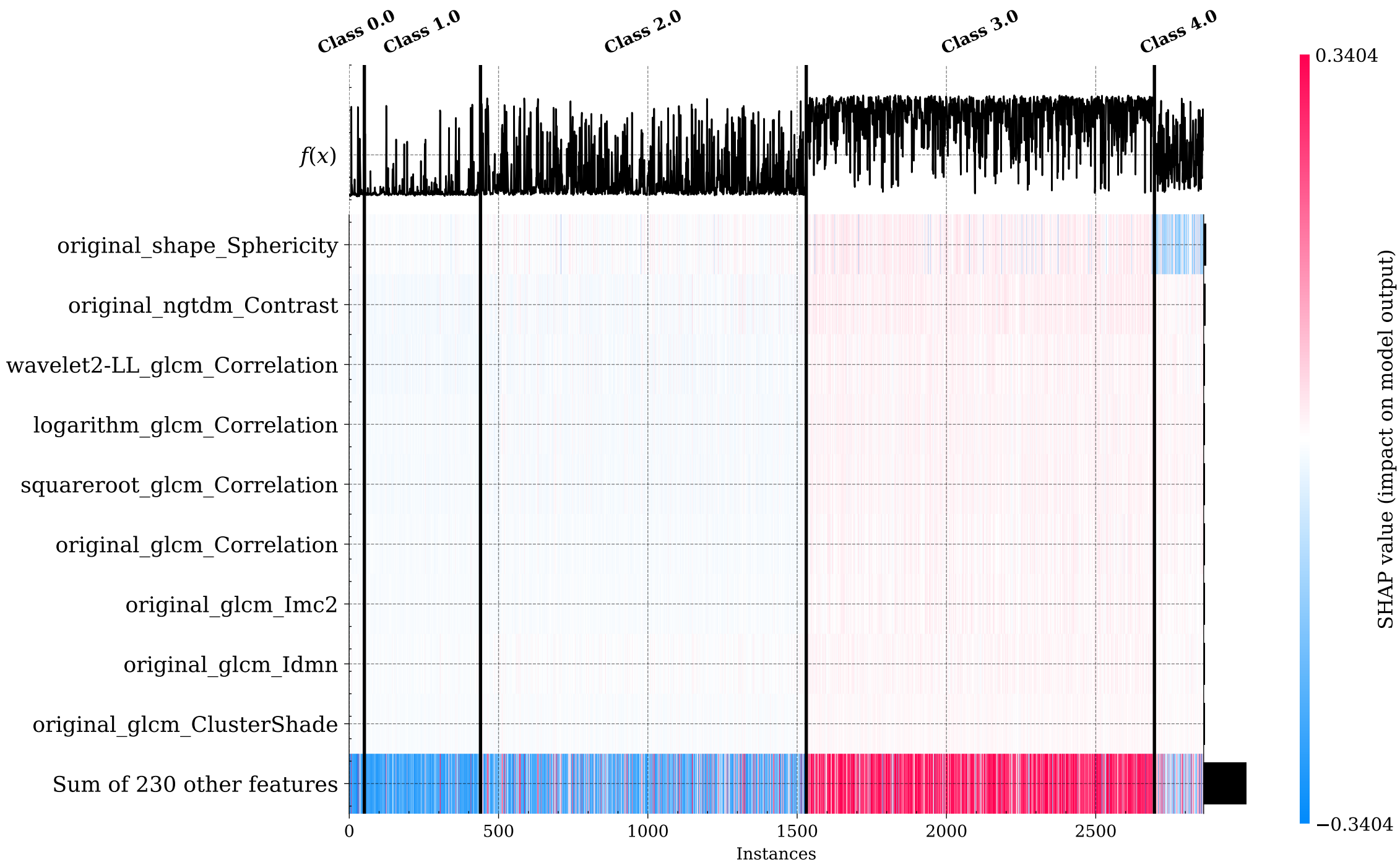
SHAP Heatmap - Class 3 vs All
