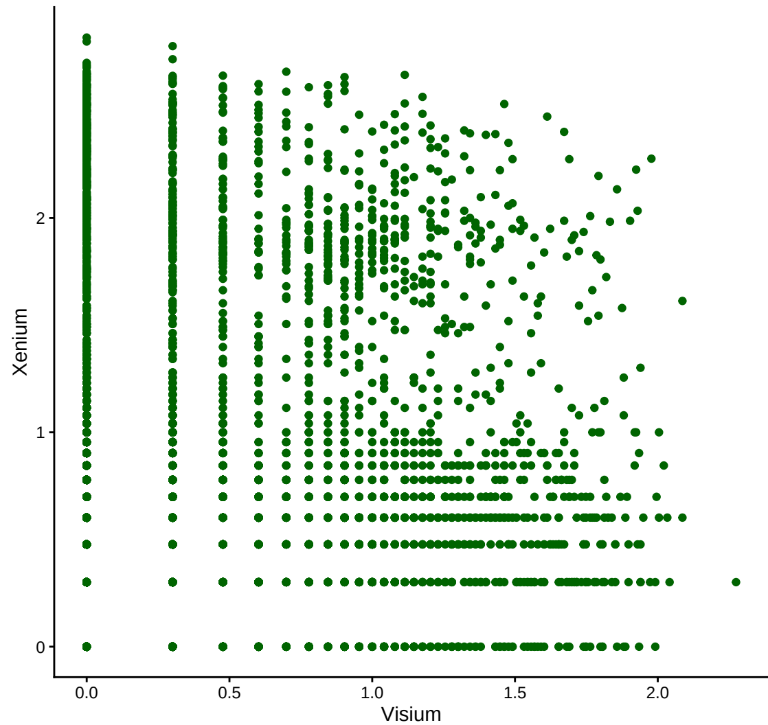
Specificity (TACSTD2)
