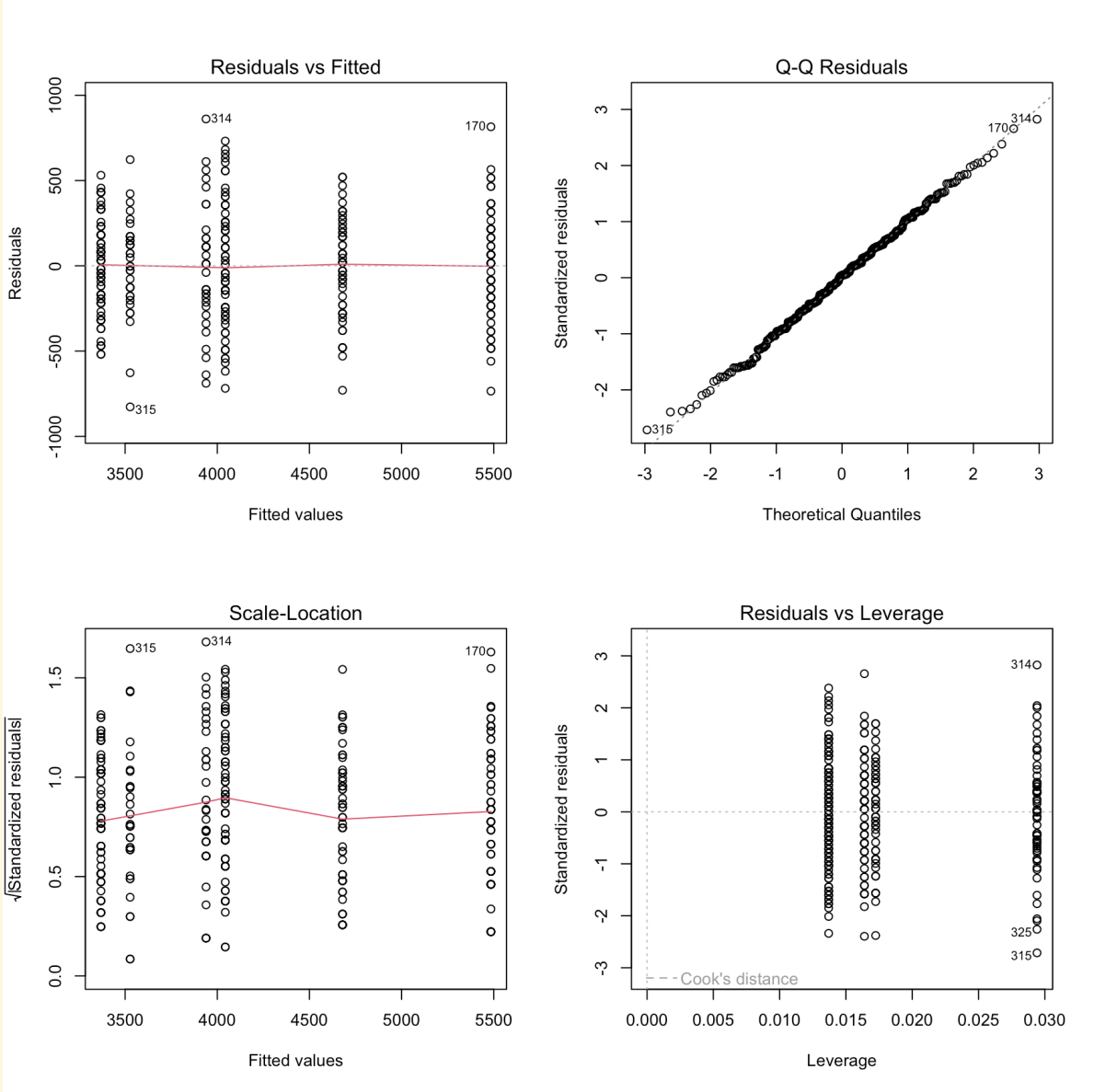
Diagnostic plots for the linear model with species and sex as predictors of body mass.
