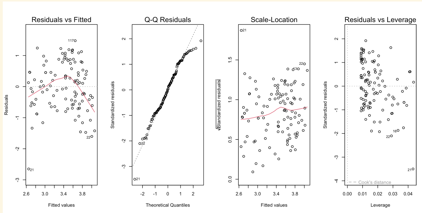
Figure 2: Residual diagnostics of the log-transformed model
