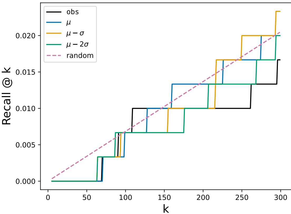
Recall @ k s = 53
