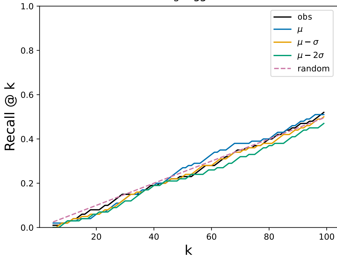
Recall @ k s = 53
