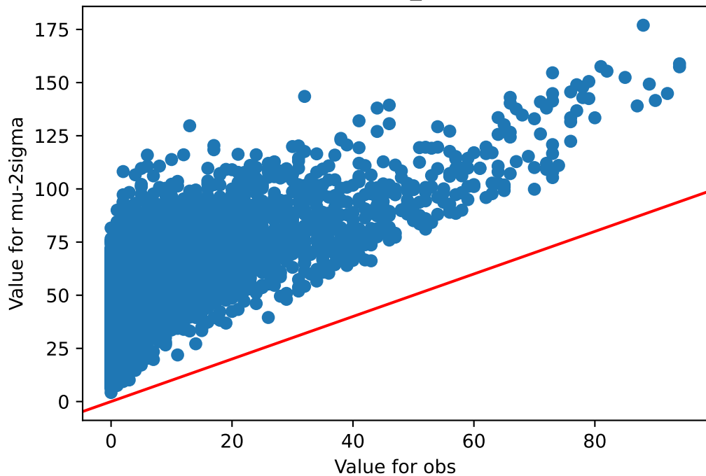
obs v/s mu-2sigma Thyroid_237
