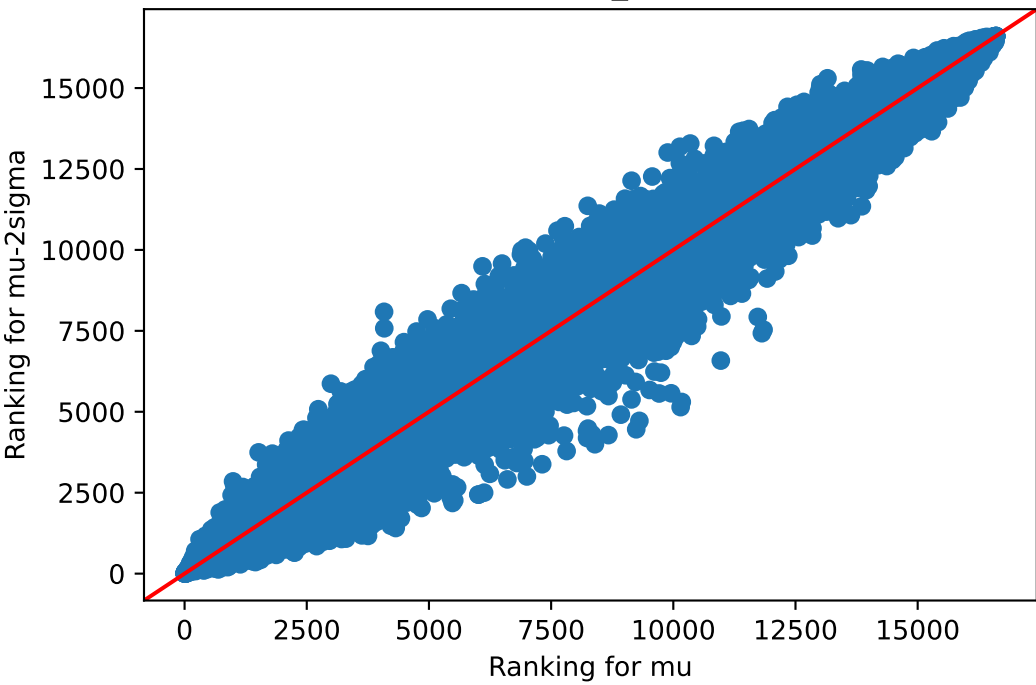
mu v/s mu-2sigma Thyroid_237
