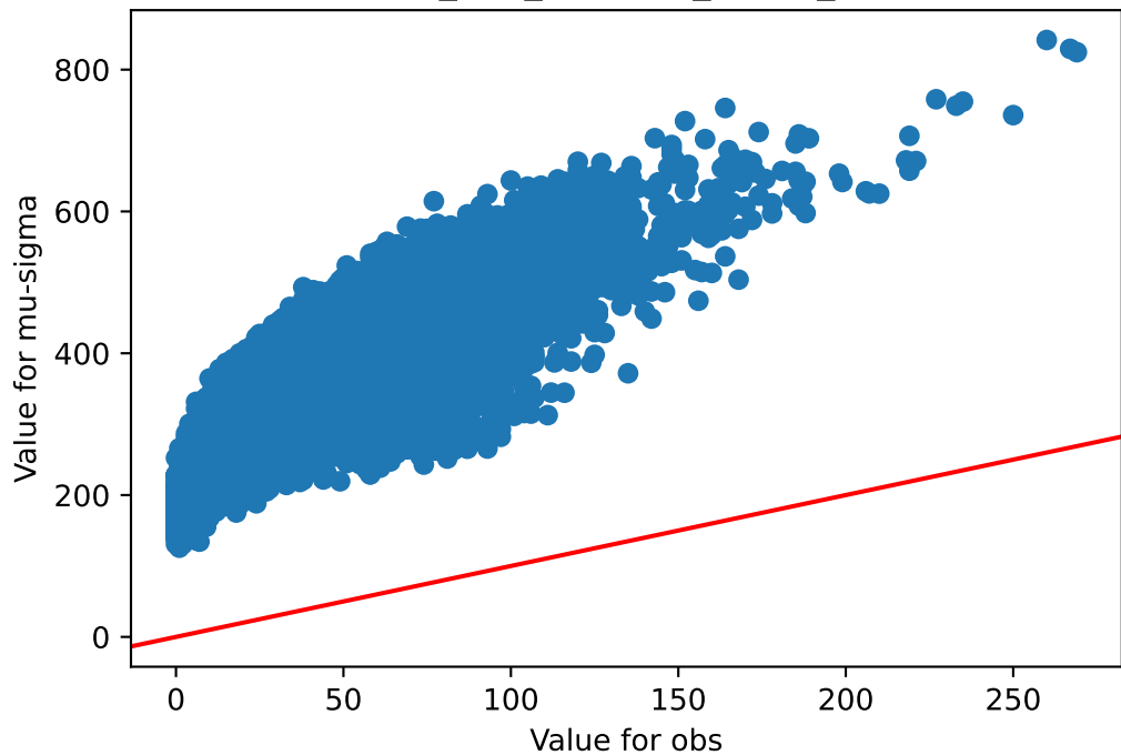
obs v/s mu-sigma Skin_Sun_Exposed_Lower_leg
