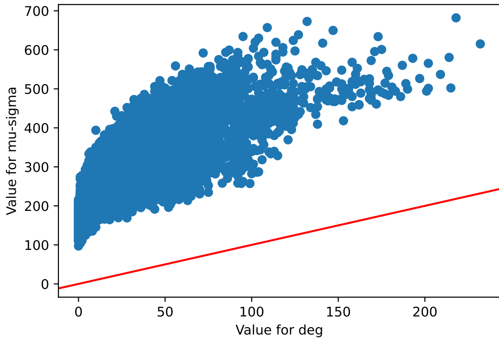
deg v/s mu-sigma Pituitary
