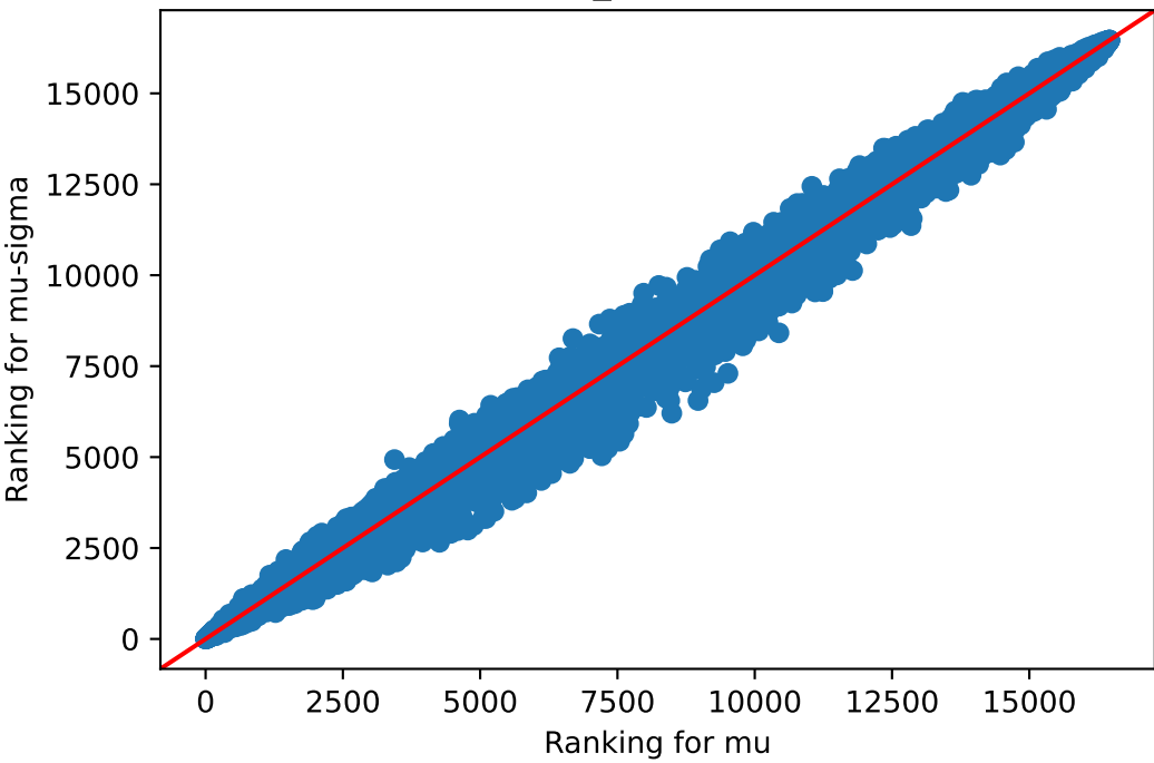
mu v/s mu-sigma Brain_Cerebellum
