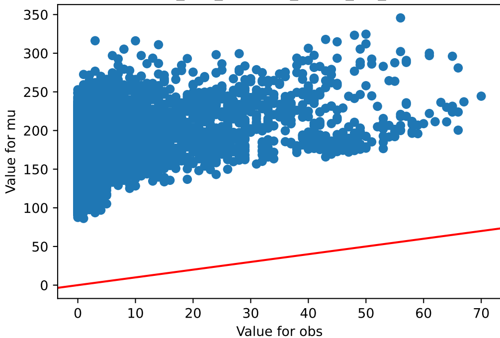
obs v/s mu Skin_Sun_Exposed_Lower_leg_237
