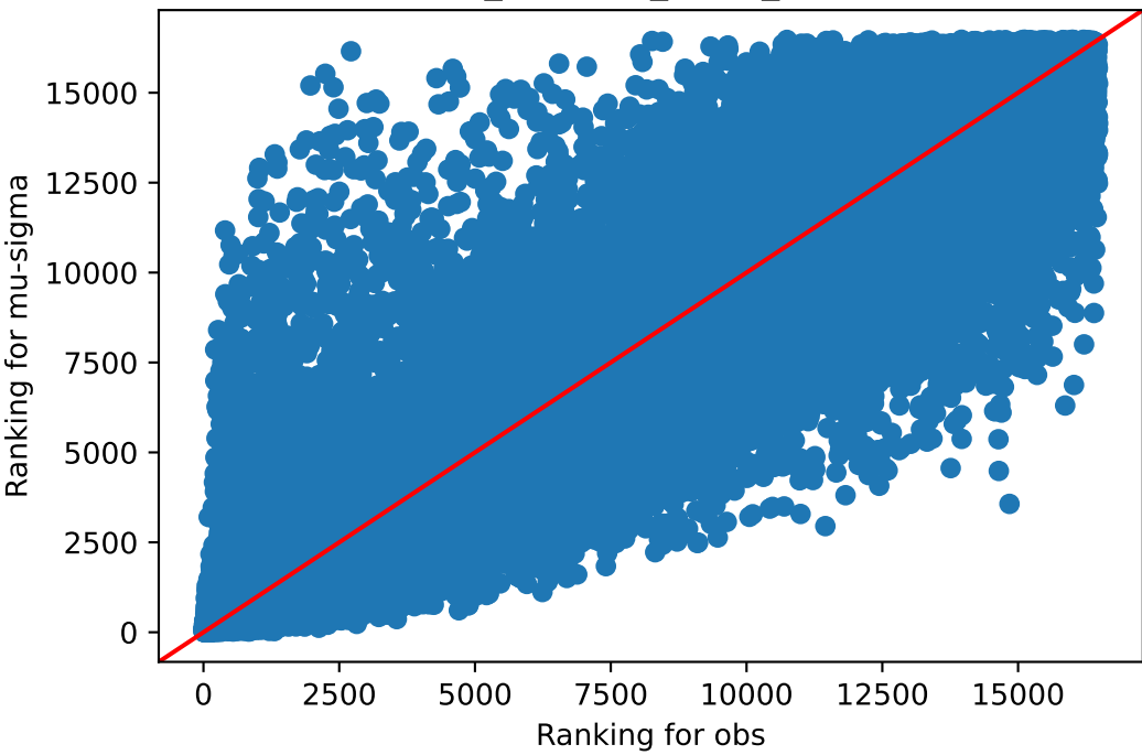
obs v/s mu-sigma Brain_Caudate_basal_ganglia
