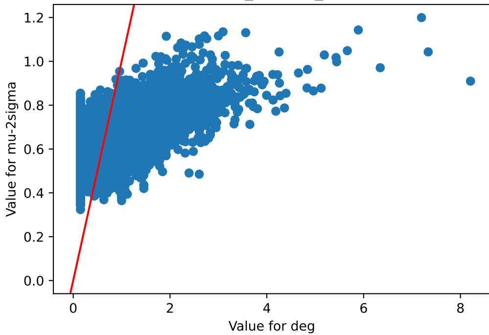
deg v/s mu-2sigma Muscle_Skeletal_237
