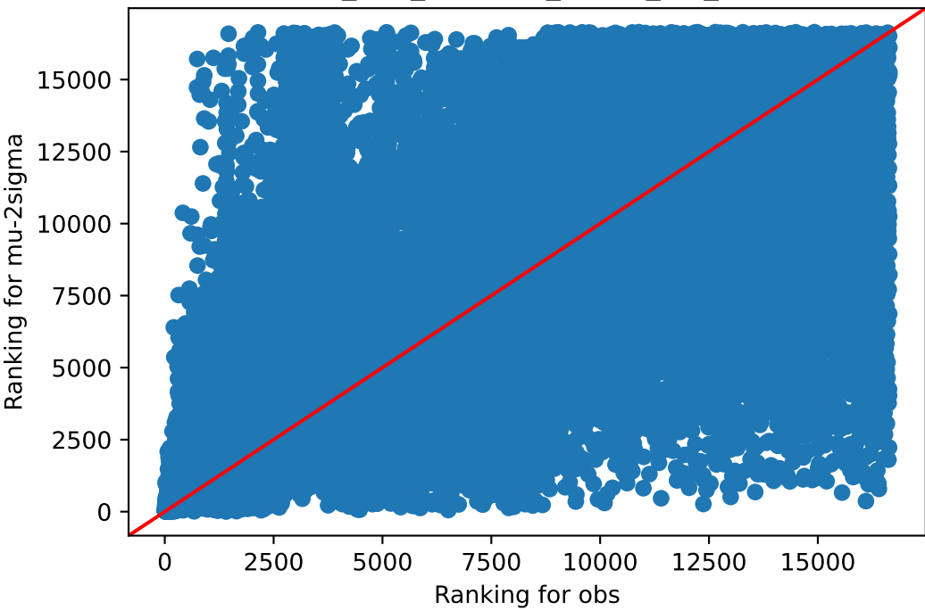
obs v/s mu-2sigma Skin_Sun_Exposed_Lower_leg_237
