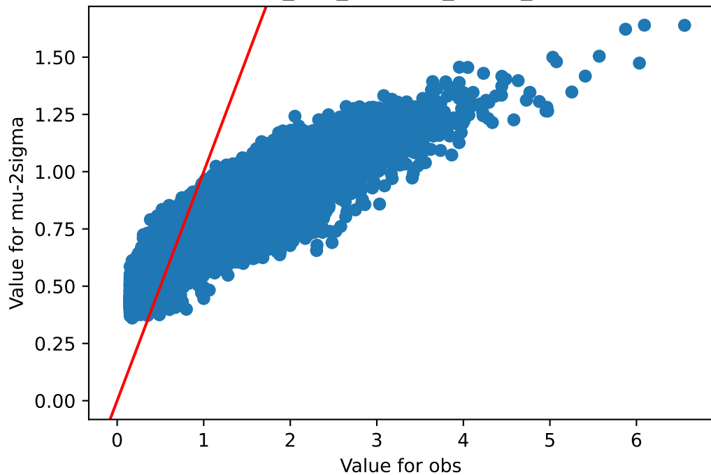
obs v/s mu-2sigma Skin_Sun_Exposed_Lower_leg
