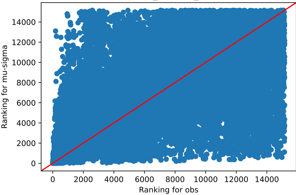
obs v/s mu-sigma Muscle_Skeletal_237
