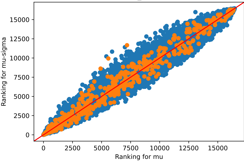
mu v/s mu-sigma Kidney_Cortex
