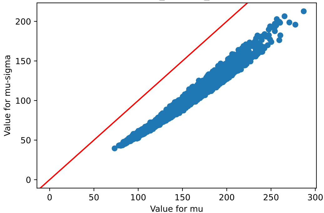
mu v/s mu-sigma Muscle_Skeletal_237
