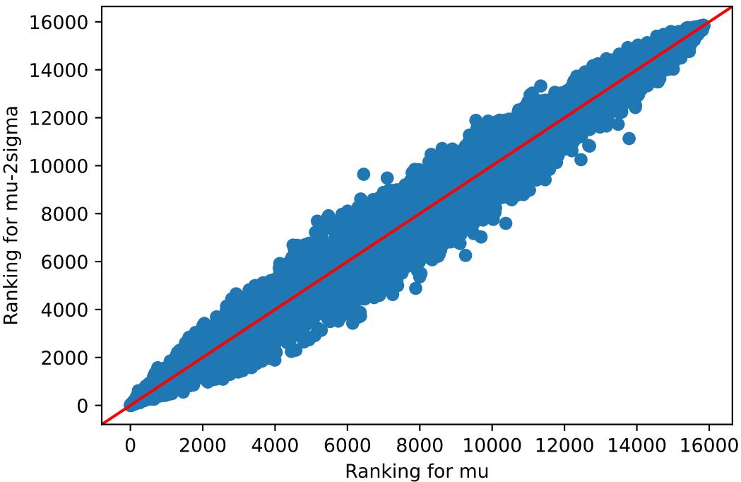
mu v/s mu-2sigma Pancreas
