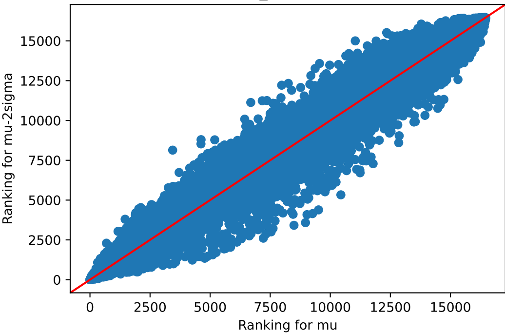
mu v/s mu-2sigma Brain_Cerebellum
