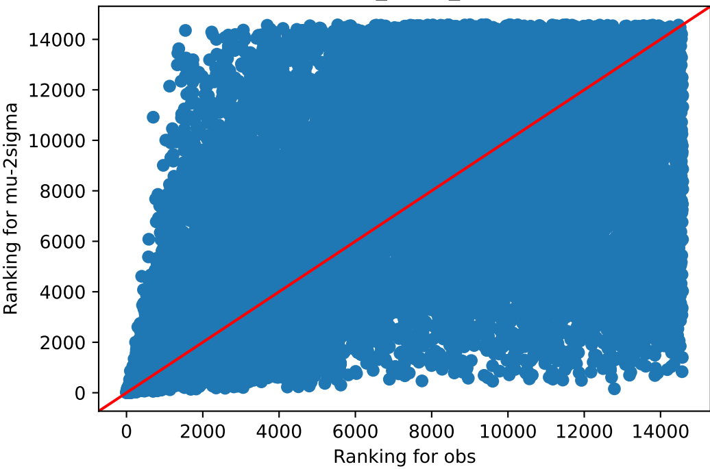
obs v/s mu-2sigma Whole_Blood_237
