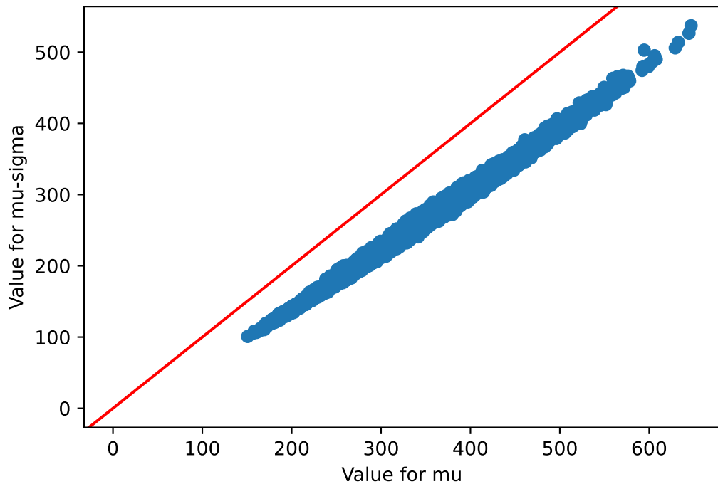
mu v/s mu-sigma Stomach
