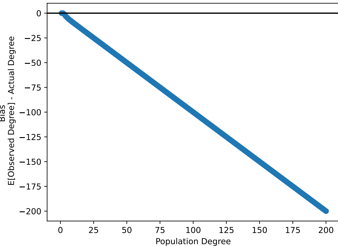
Estimator Bias -- 1% FDR
