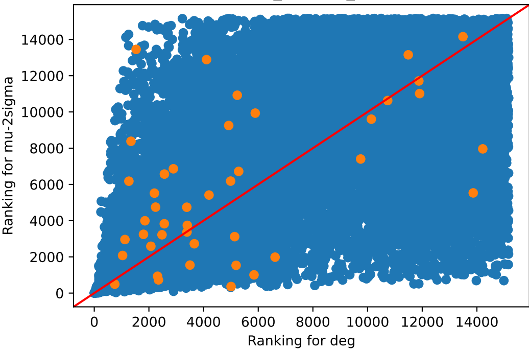
deg v/s \mu -2sigma Muscle_Skeletal_237
