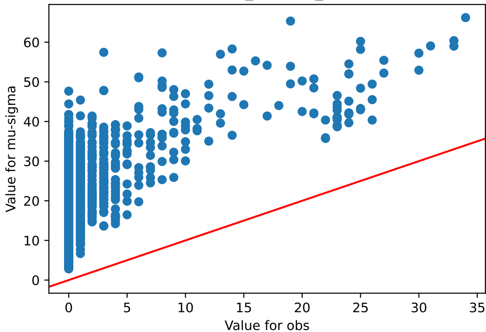
obs v/s mu-sigma Muscle_Skeletal_73
