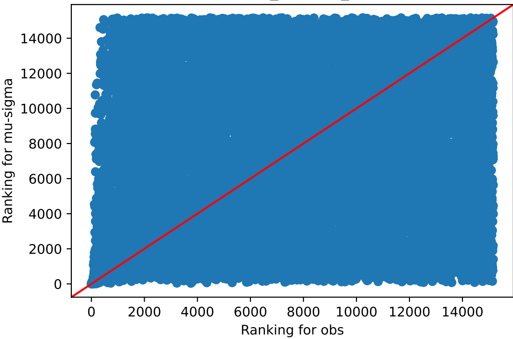
obs v/s mu-sigma Muscle_Skeletal_73
