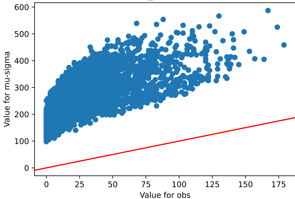
obs v/s mu-sigma Brain_Cerebellum
