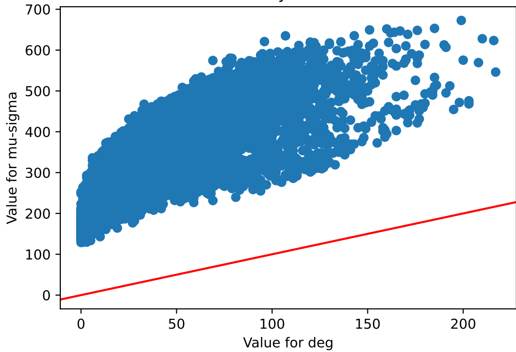
deg v/s mu-sigma Thyroid
