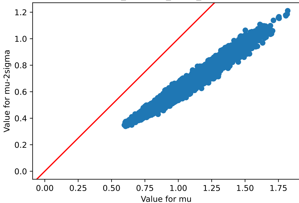
mu v/s mu-2sigma Brain_Caudate_basal_ganglia
