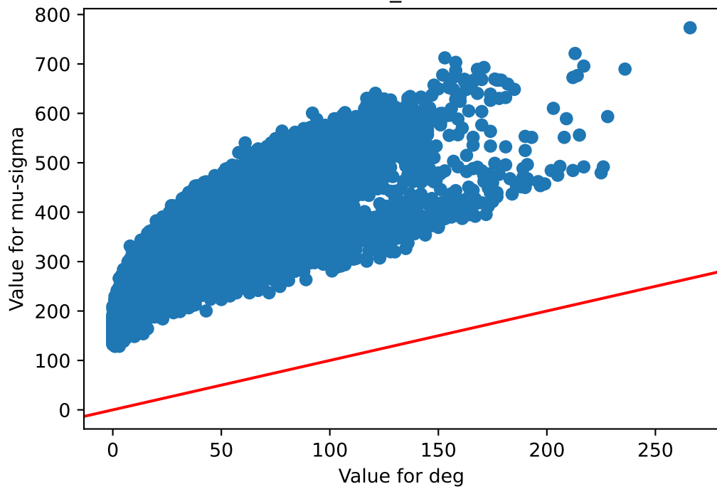
deg v/s mu-sigma Muscle_Skeletal
