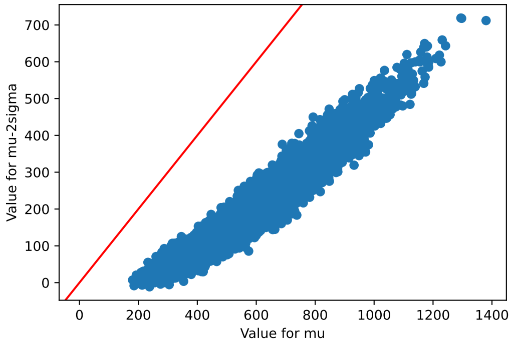
mu v/s mu-2sigma Uterus
