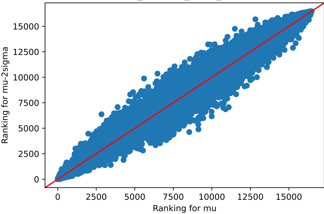
mu v/s mu-2sigma Brain_Caudate_basal_ganglia
