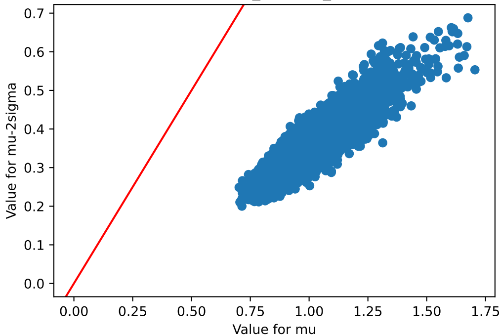
mu v/s mu-2sigma Muscle_Skeletal_73
