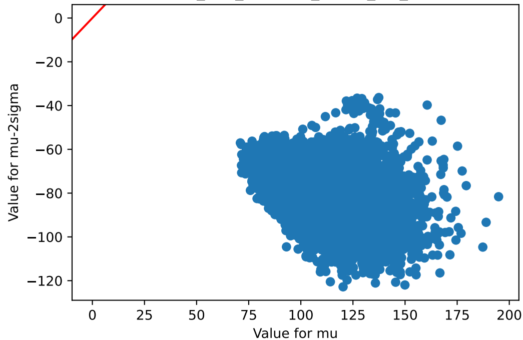
mu v/s mu-2sigma Skin_Sun_Exposed_Lower_leg_73
