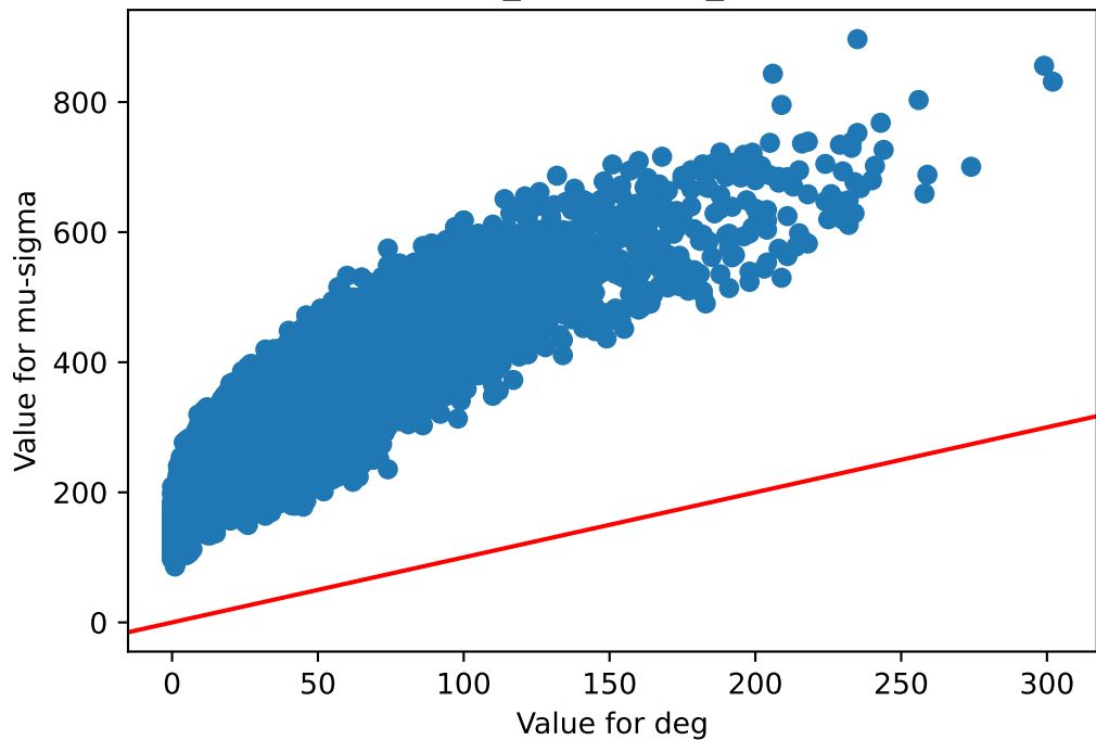
deg v/s mu-sigma Brain_Substantia_nigra
