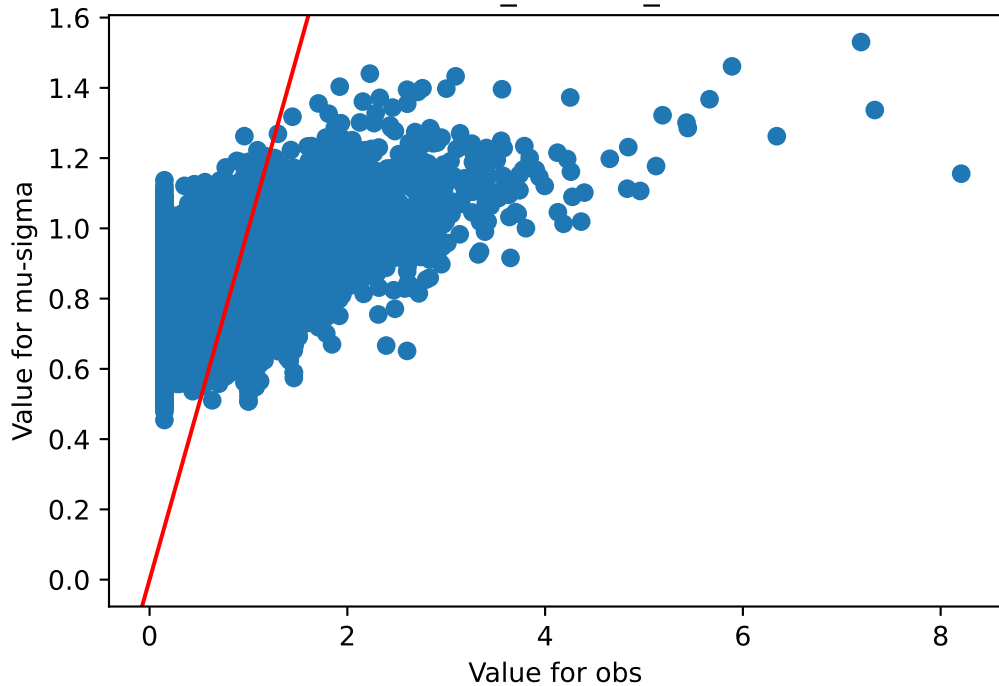
obs v/s mu-sigma Muscle_Skeletal_237
