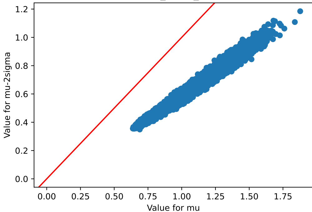
mu v/s mu-2sigma Whole_Blood_237
