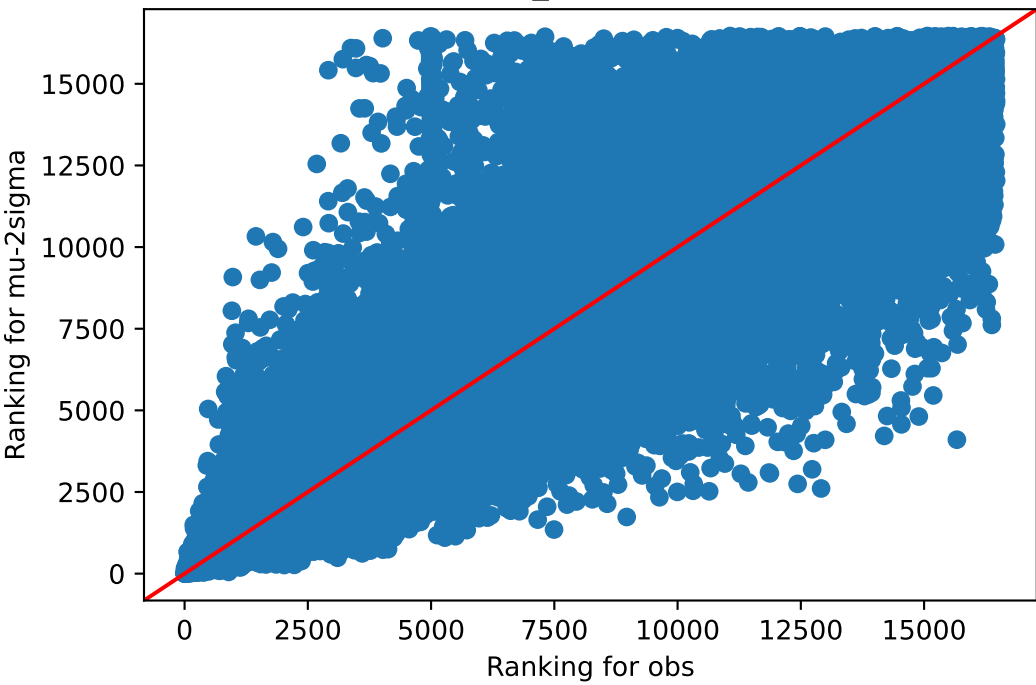
obs v/s mu-2sigma Brain_Cerebellum
