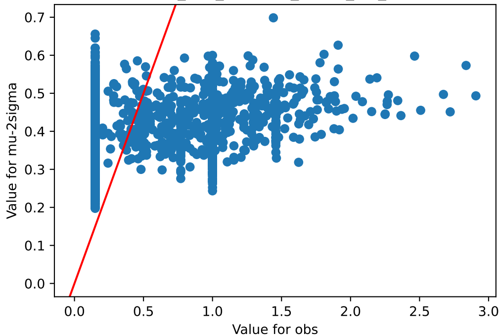
obs v/s mu-2sigma Skin_Sun_Exposed_Lower_leg_73
