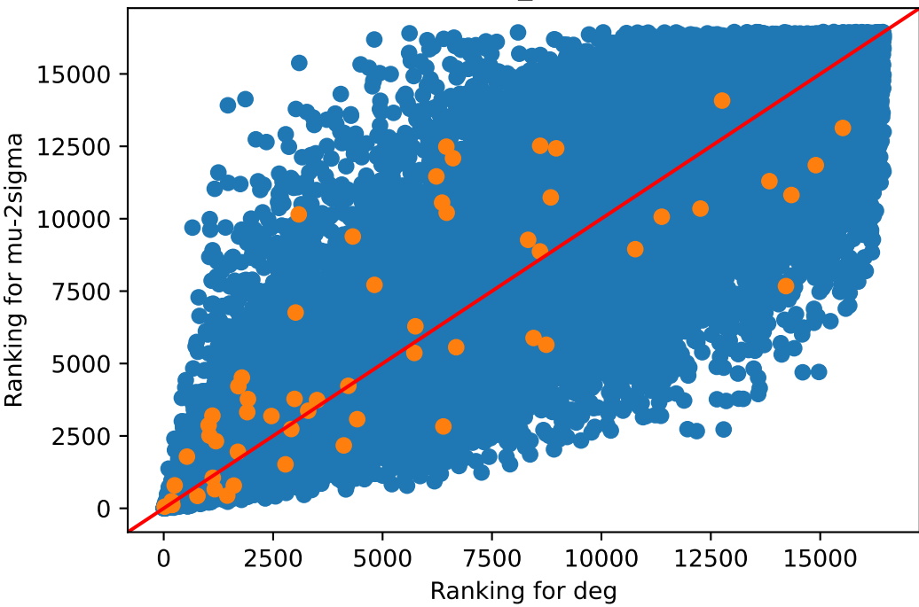
deg v/s \mu -2sigma Kidney_Cortex
