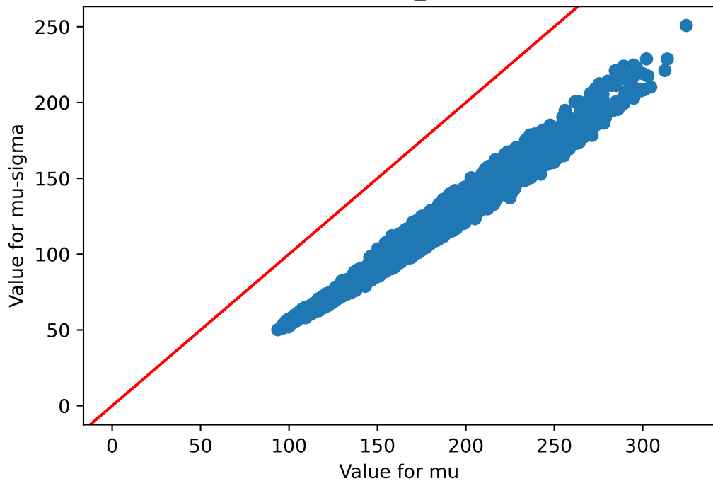
mu v/s mu-sigma Thyroid_237
