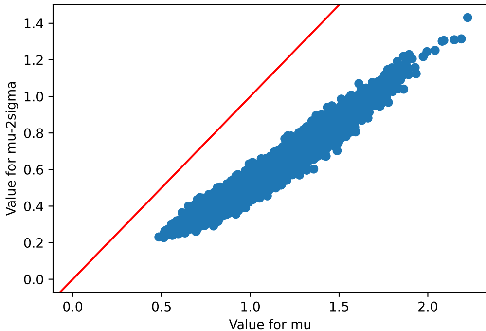
mu v/s mu-2sigma Brain_Substantia_nigra
