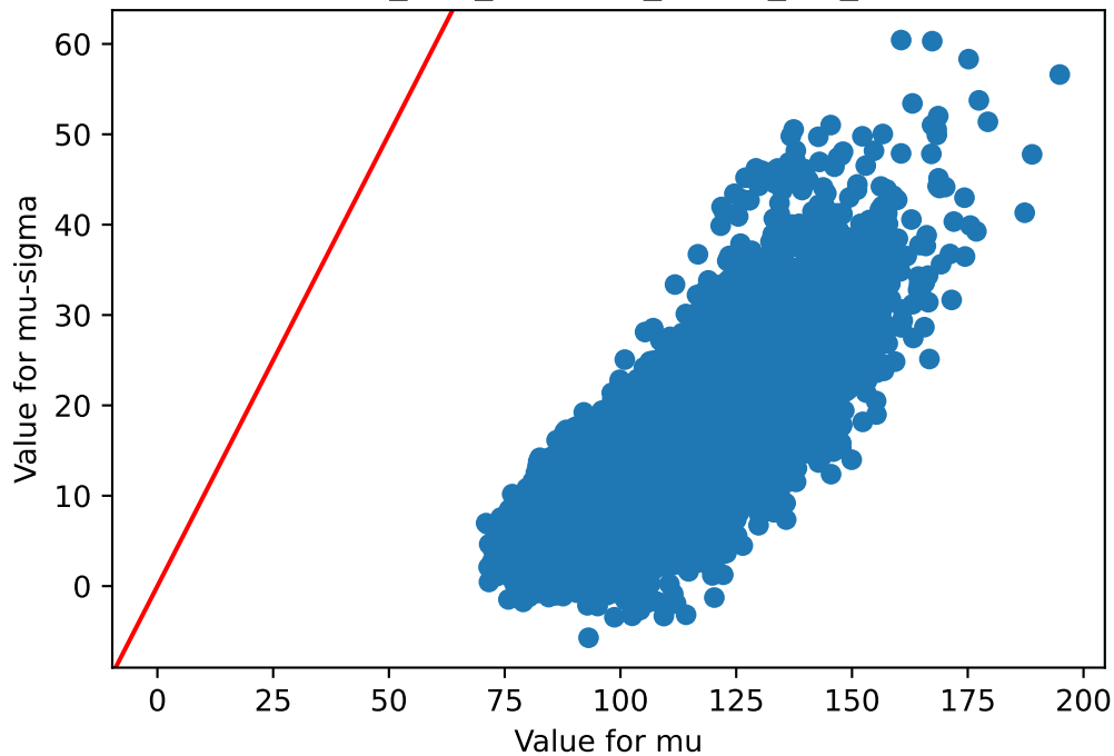
mu v/s mu-sigma Skin_Sun_Exposed_Lower_leg_73
