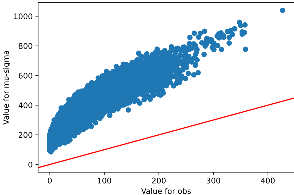
obs v/s mu-sigma Brain_Amygdala
