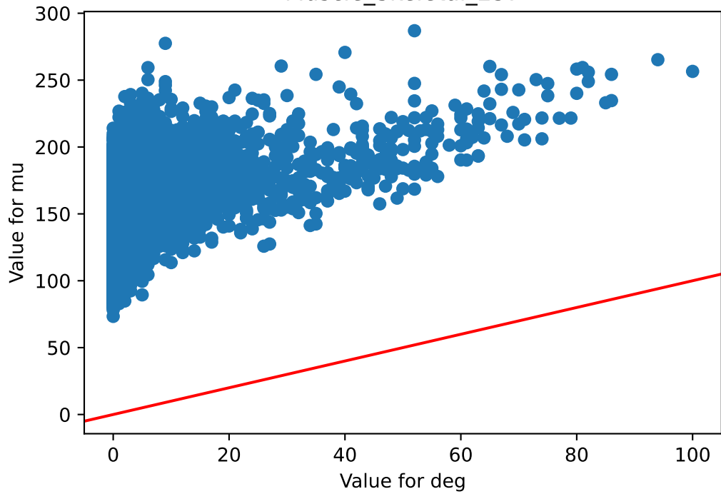
deg v/s mu Muscle_Skeletal_237
