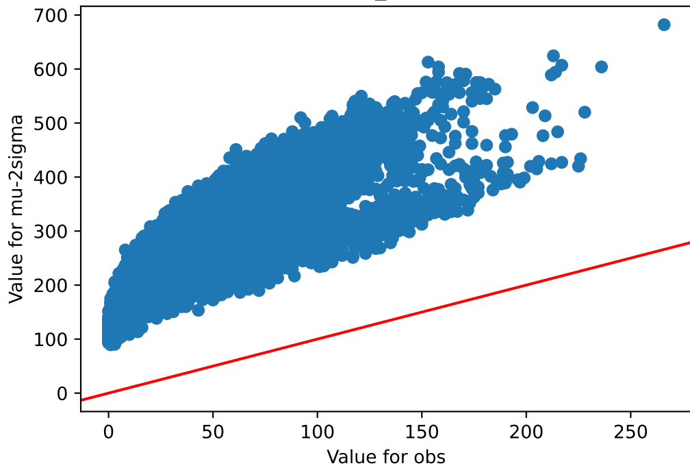
obs v/s mu-2sigma Muscle_Skeletal
