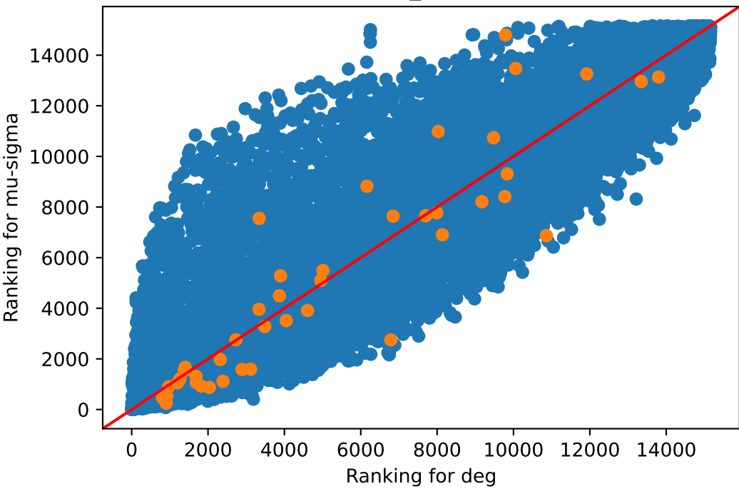
deg v/s mu-sigma Muscle_Skeletal
