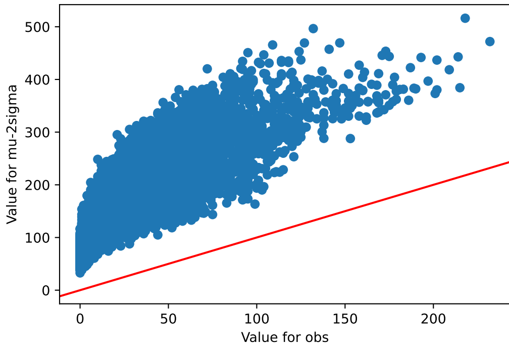
obs v/s mu-2sigma Pituitary
