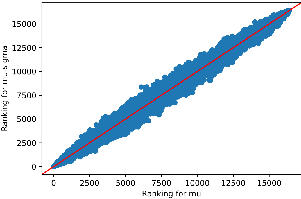
mu v/s mu-sigma Uterus
