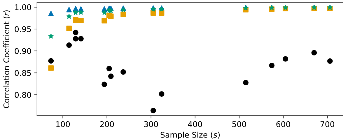
Spearman Correlation among Centrality Metrics (with respect to sample size)
