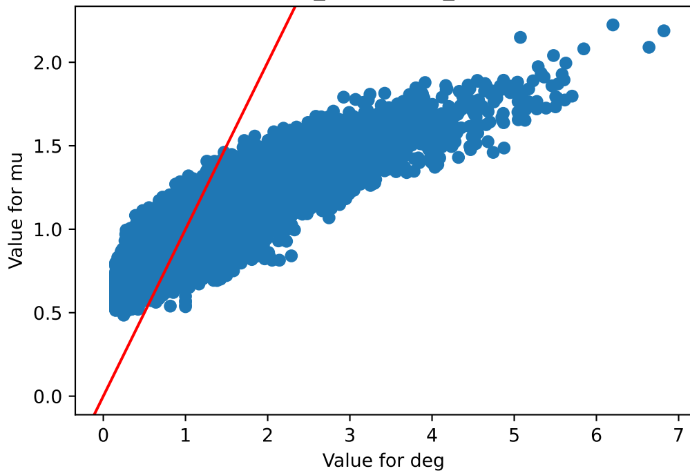
deg v/s mu Brain_Substantia_nigra
