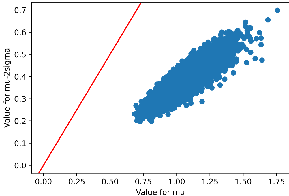
mu v/s mu-2sigma Skin_Sun_Exposed_Lower_leg_73
