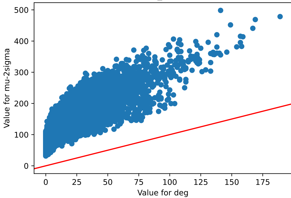
deg v/s \mu -2sigma Brain_Cortex
