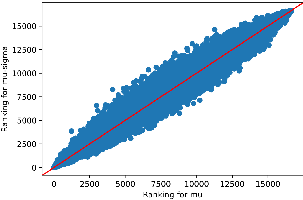
mu v/s mu-sigma Skin_Sun_Exposed_Lower_leg_73
