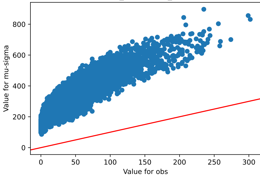
obs v/s mu-sigma Brain_Substantia_nigra
