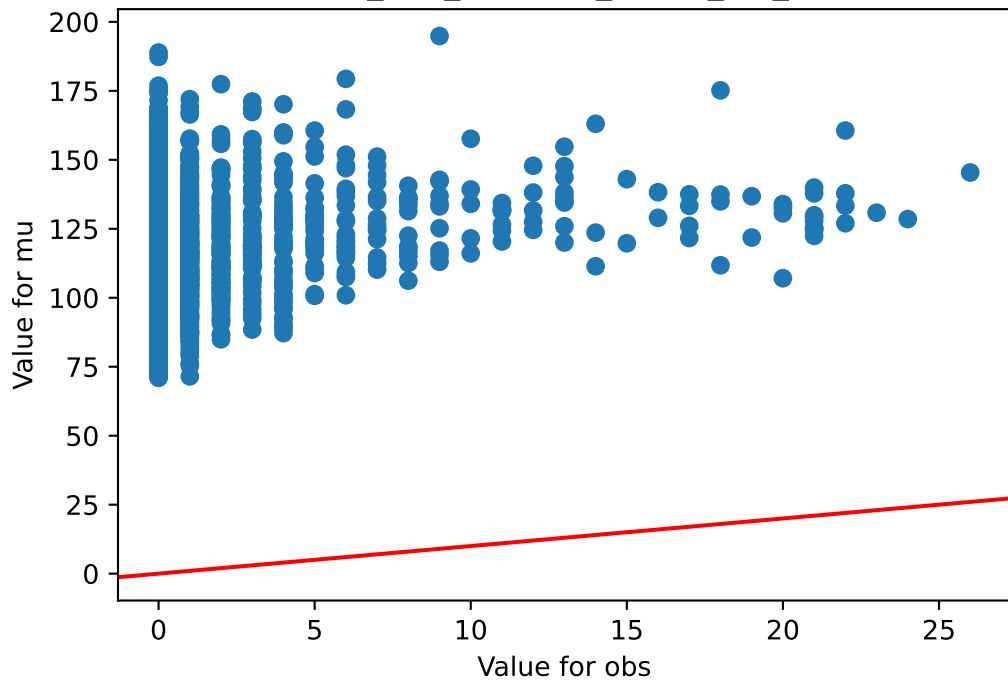
obs v/s mu Skin_Sun_Exposed_Lower_leg_73
