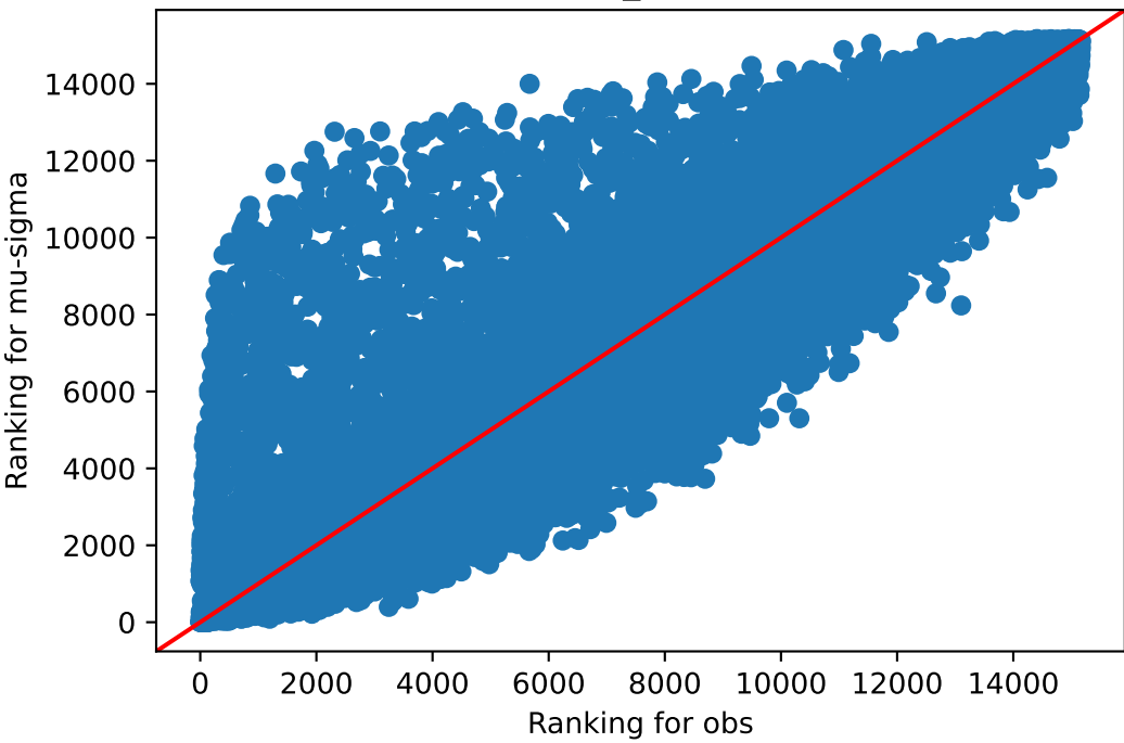
obs v/s mu-sigma Muscle_Skeletal
