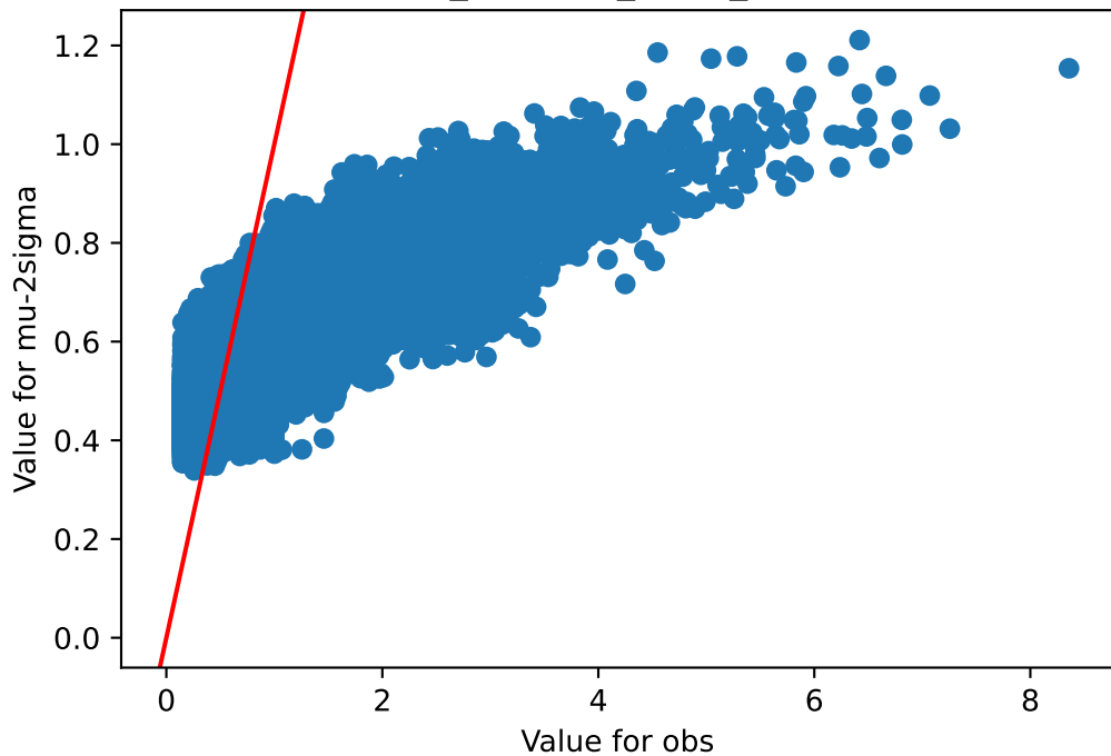
obs v/s mu-2sigma Brain_Caudate_basal_ganglia
