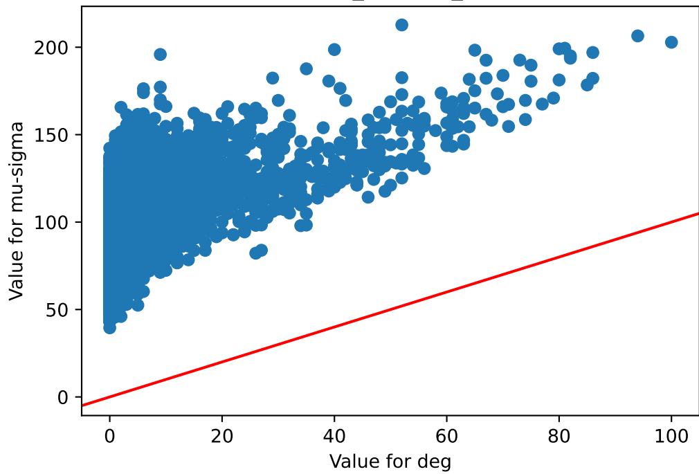
deg v/s mu-sigma Muscle_Skeletal_237
