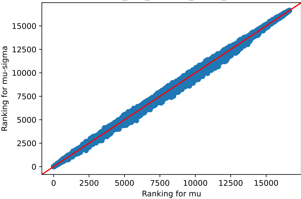
mu v/s mu-sigma Skin_Sun_Exposed_Lower_leg
