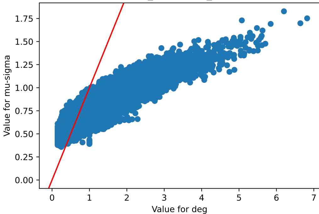
deg v/s mu-sigma Brain_Substantia_nigra
