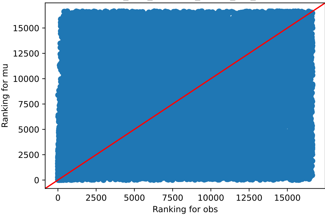
obs v/s mu Skin_Sun_Exposed_Lower_leg_73
