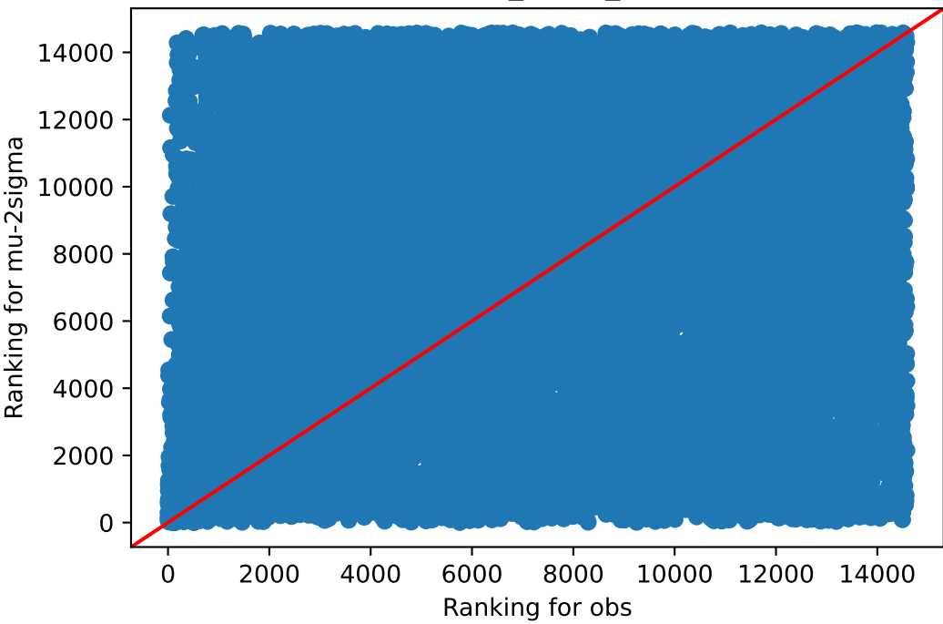
obs v/s mu-2sigma Whole_Blood_73
