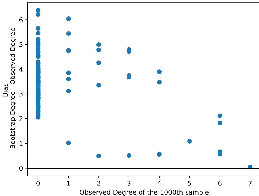
Bootstrap Bias
