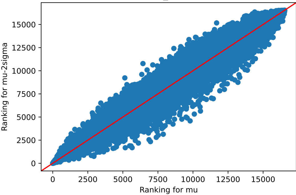
mu v/s mu-2sigma Brain_Cortex
