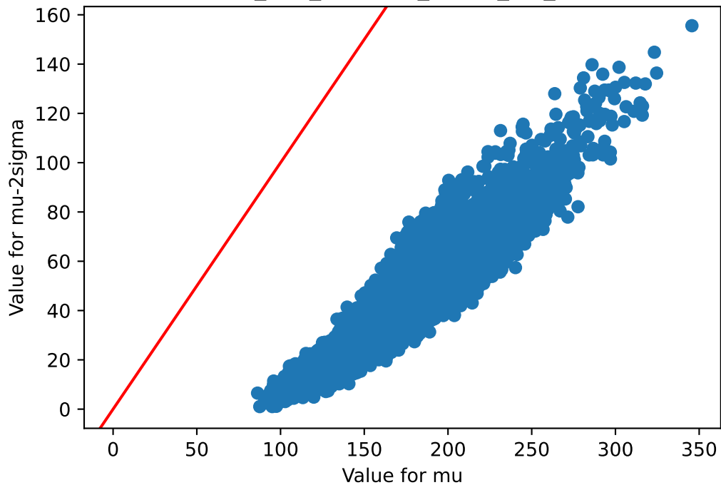
mu v/s mu-2sigma Skin_Sun_Exposed_Lower_leg_237
