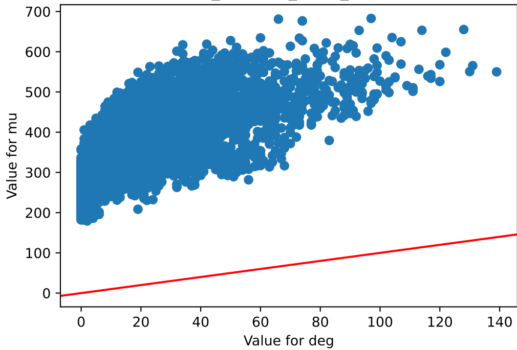
deg v/s mu Brain_Caudate_basal_ganglia
