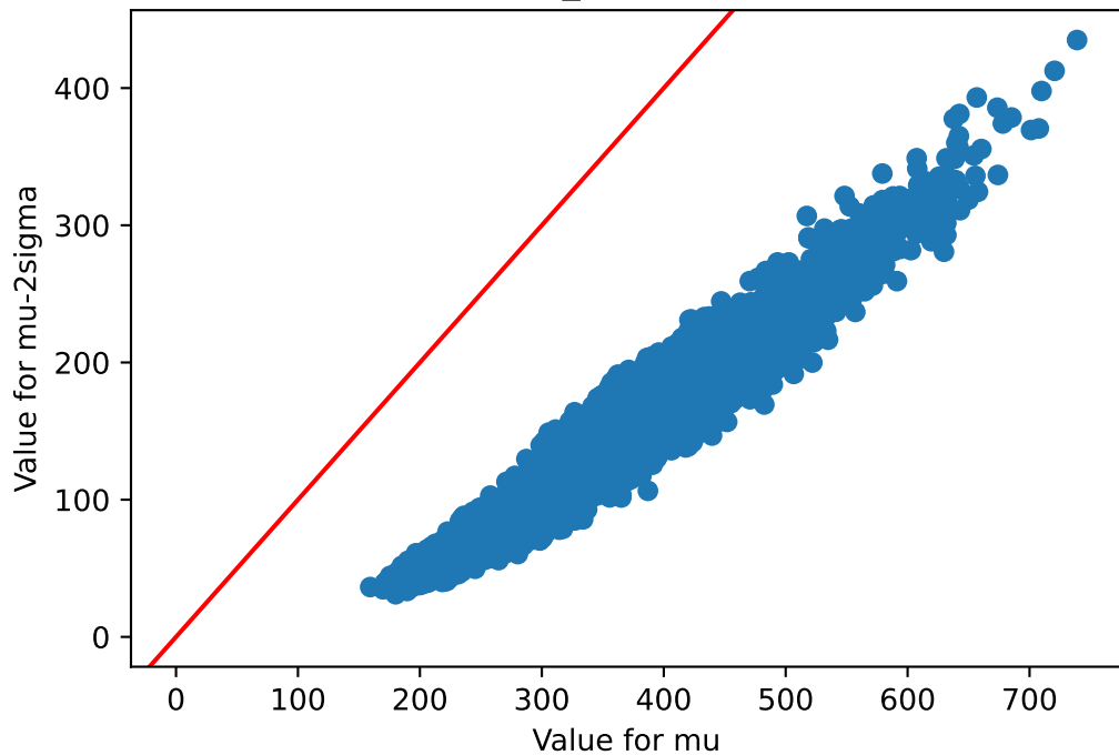
mu v/s mu-2sigma Brain_Cerebellum
