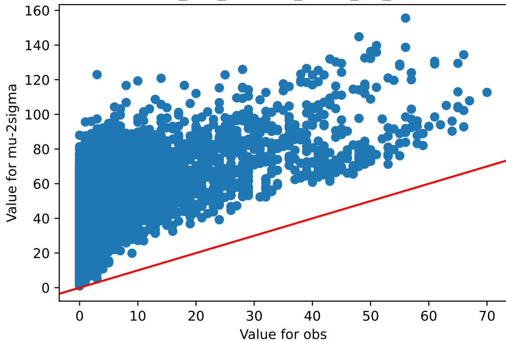
obs v/s \mu-2\sigma Skin_Sun_Exposed_Lower_leg_237
