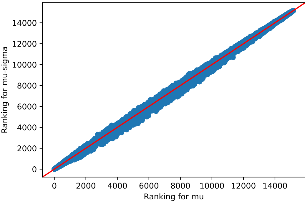
mu v/s mu-sigma Muscle_Skeletal
