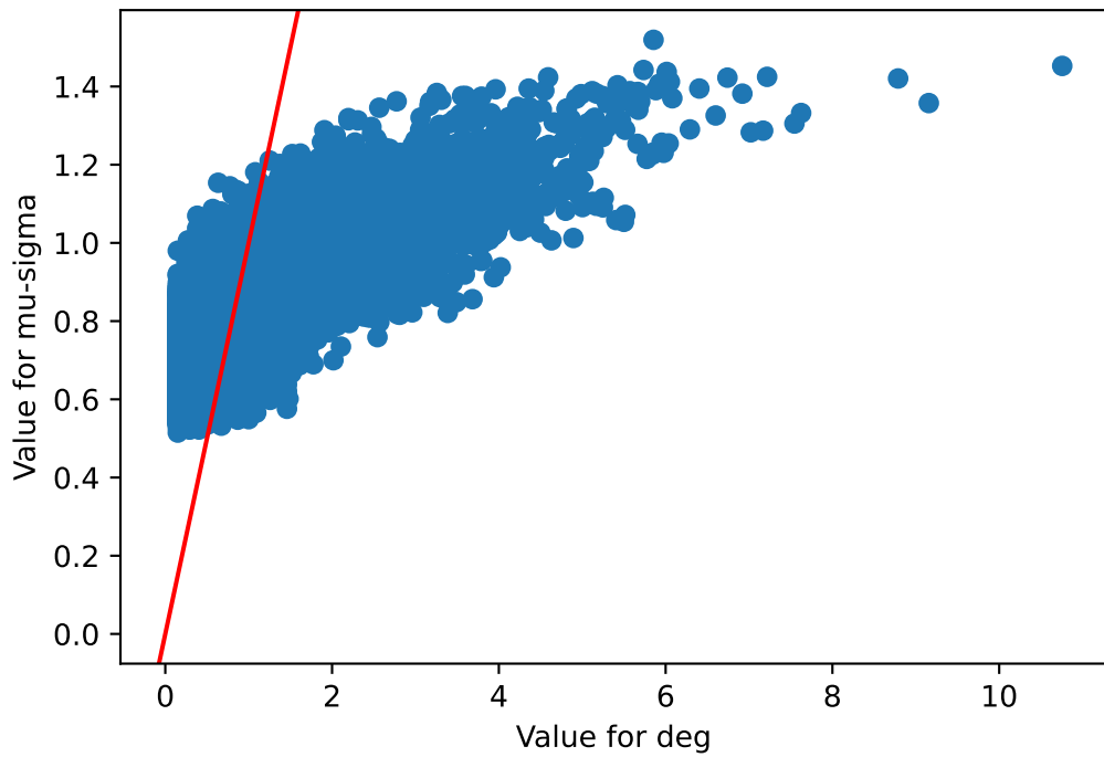
deg v/s mu-sigma Pancreas
