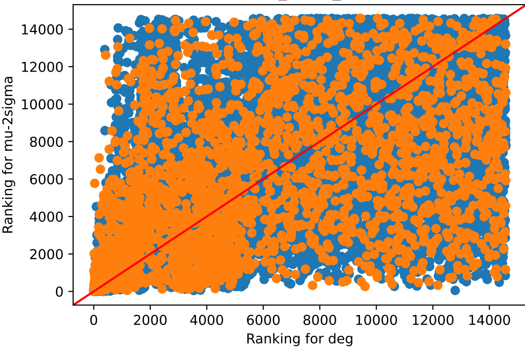
deg v/s mu-2sigma Whole_Blood_237
