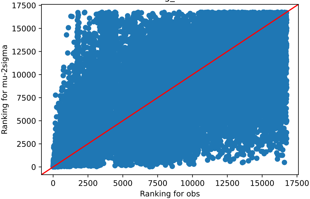
obs v/s mu-2sigma Lung_237
