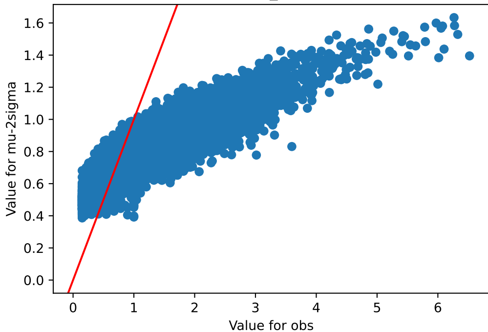
obs v/s mu-2sigma Whole_Blood
