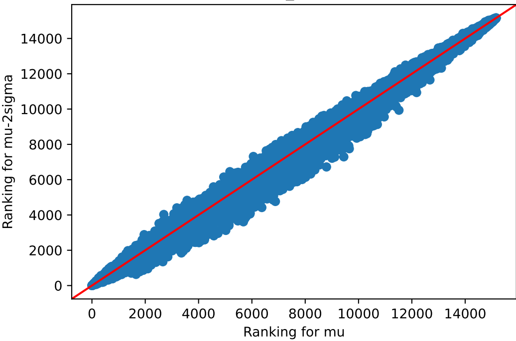
mu v/s mu-2sigma Muscle_Skeletal
