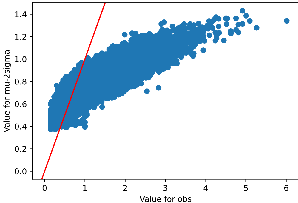
obs v/s mu-2sigma Thyroid
