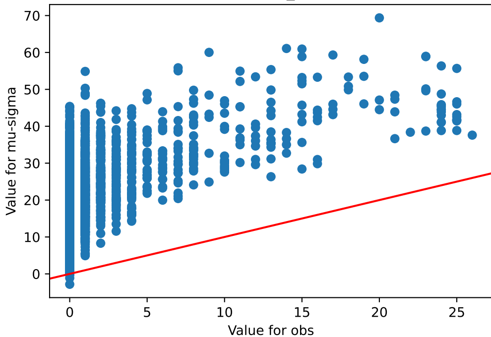
obs v/s mu-sigma Thyroid_73
