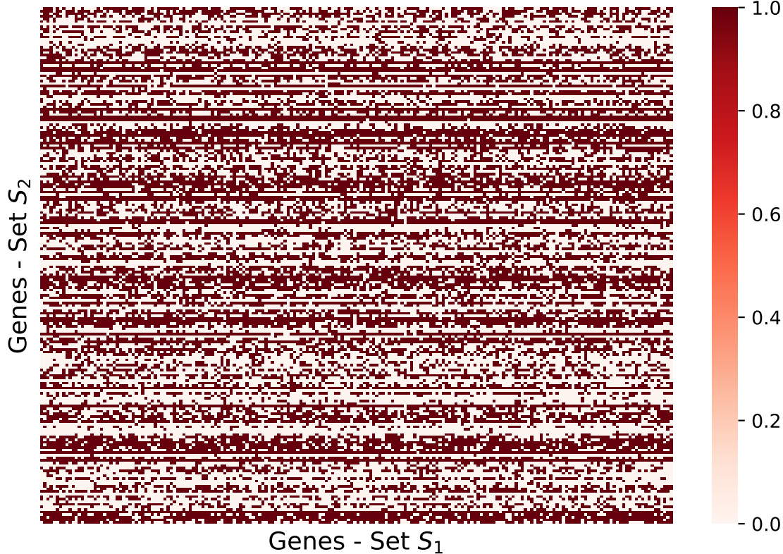
Adjacency Matrix s = 1000000
