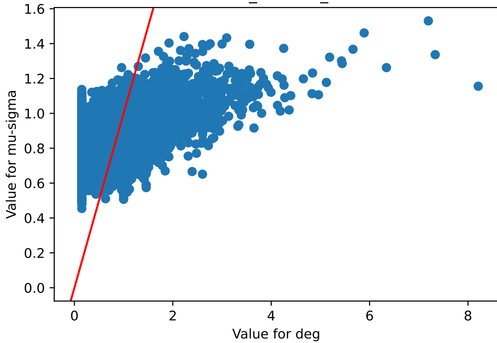
deg v/s mu-sigma Muscle_Skeletal_237
