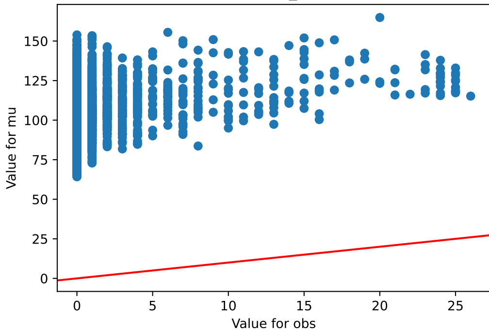
obs v/s mu Thyroid_73
