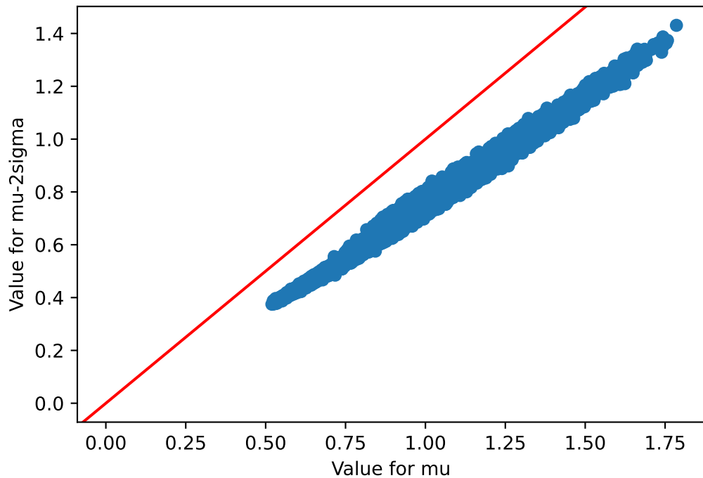
mu v/s mu-2sigma Thyroid
