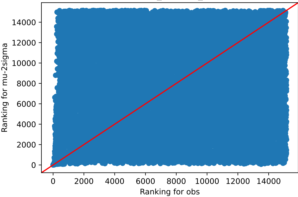
obs v/s mu-2sigma Muscle_Skeletal_73
