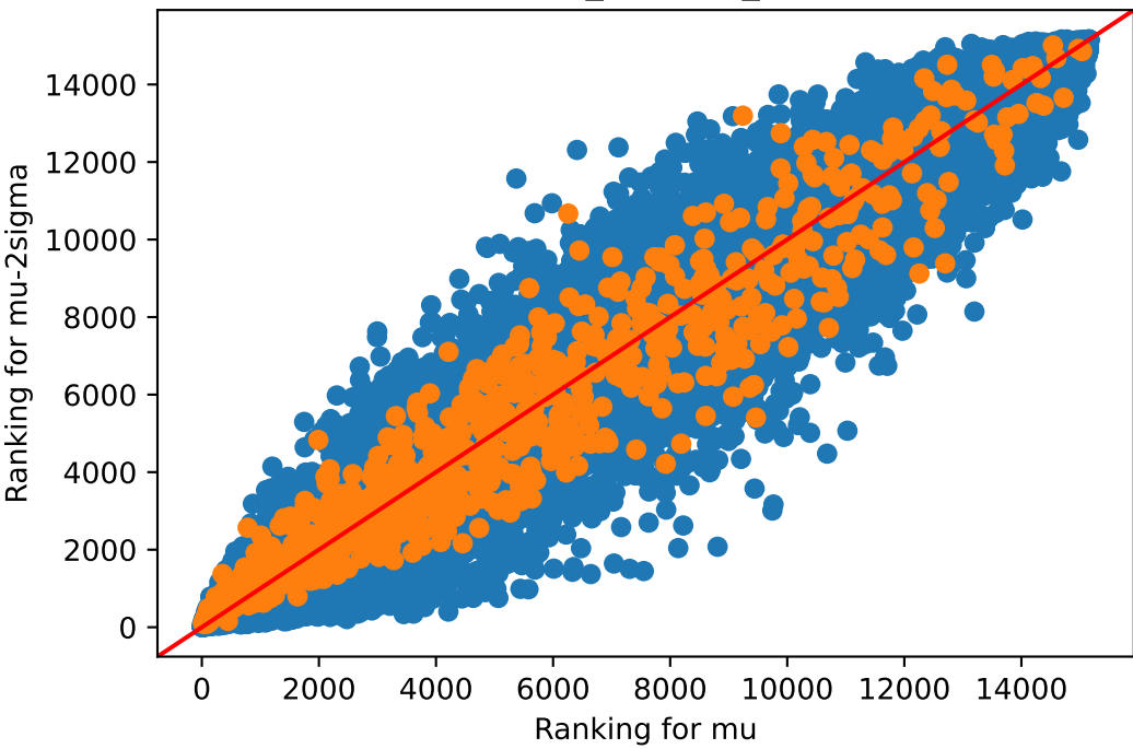
mu v/s mu-2sigma Muscle_Skeletal_237
