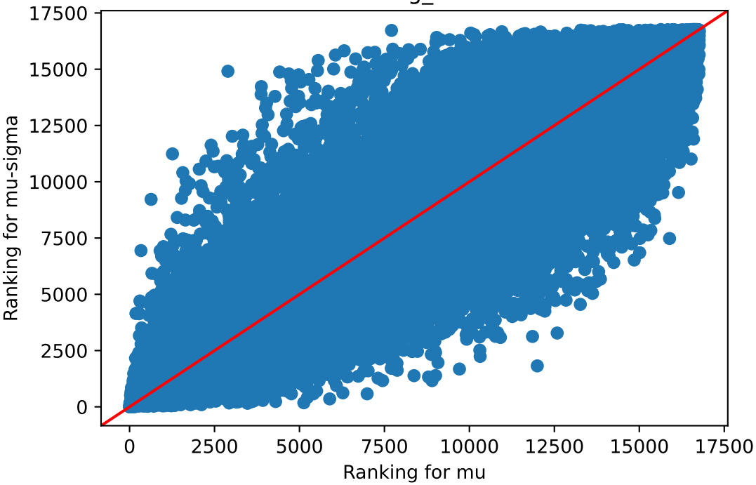
mu v/s mu-sigma Lung_73
