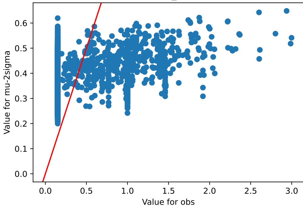
obs v/s mu-2sigma Lung_73
