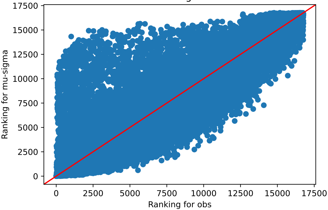
obs v/s mu-sigma Lung
