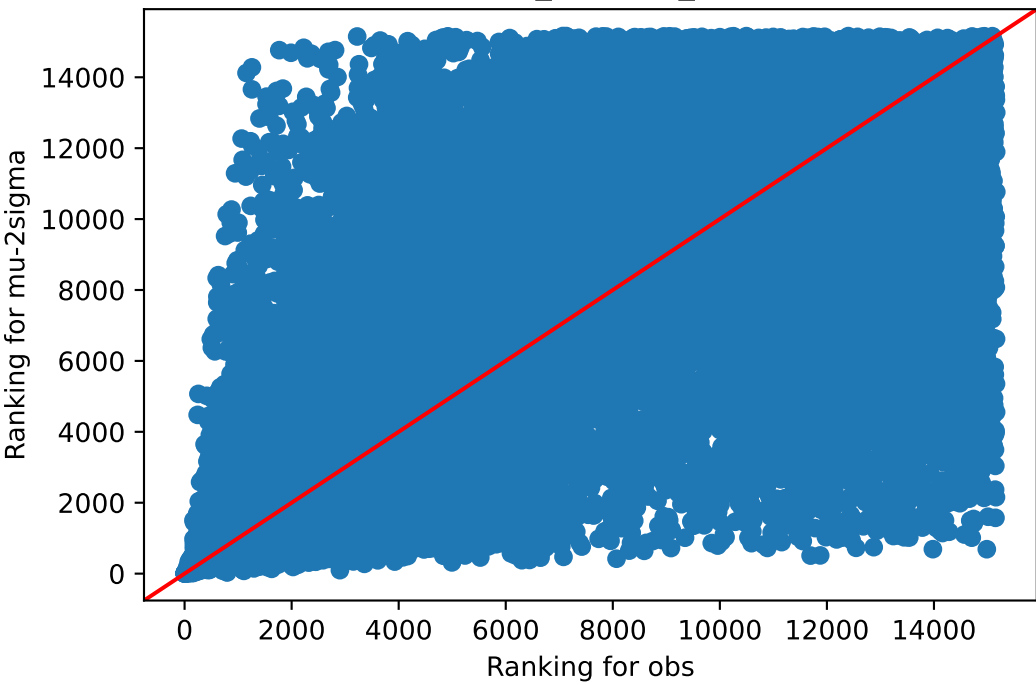
obs v/s mu-2sigma Muscle_Skeletal_237
