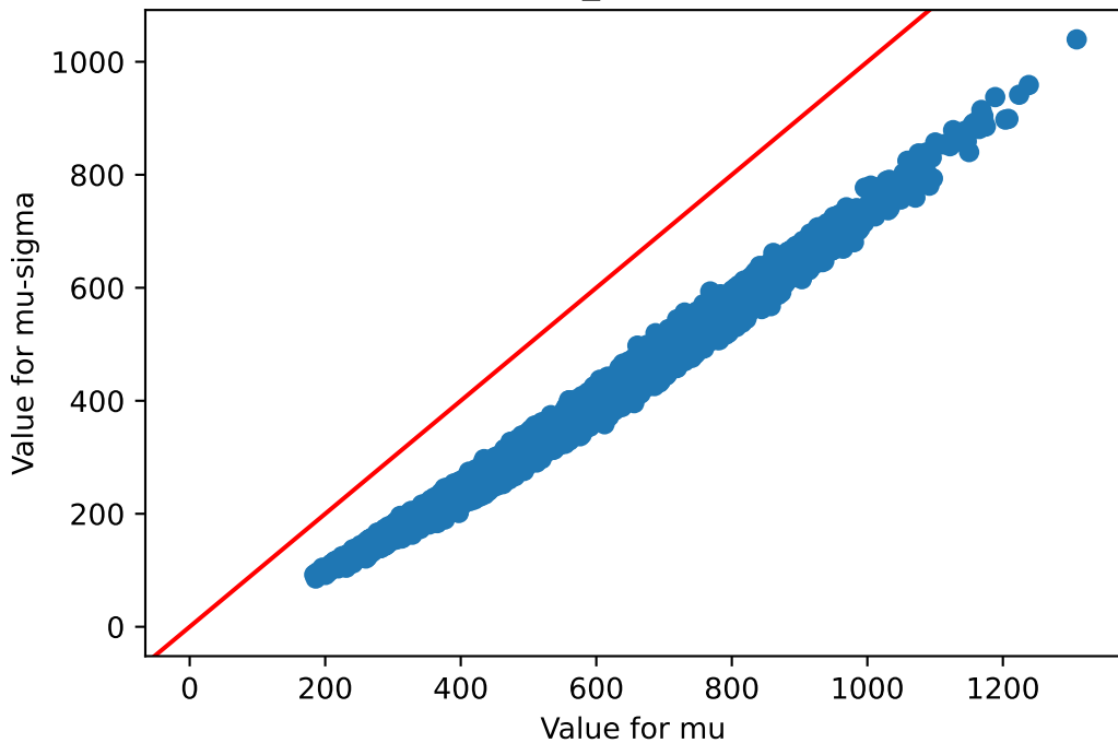
mu v/s mu-sigma Brain_Amygdala
