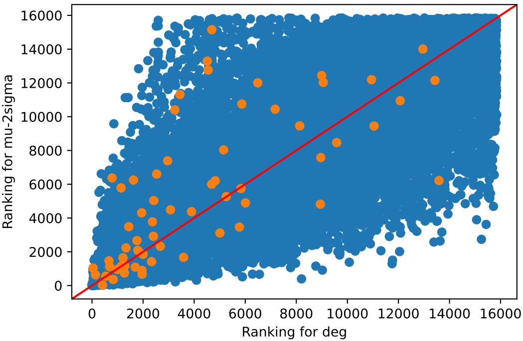
deg v/s \mu -2sigma Pancreas
