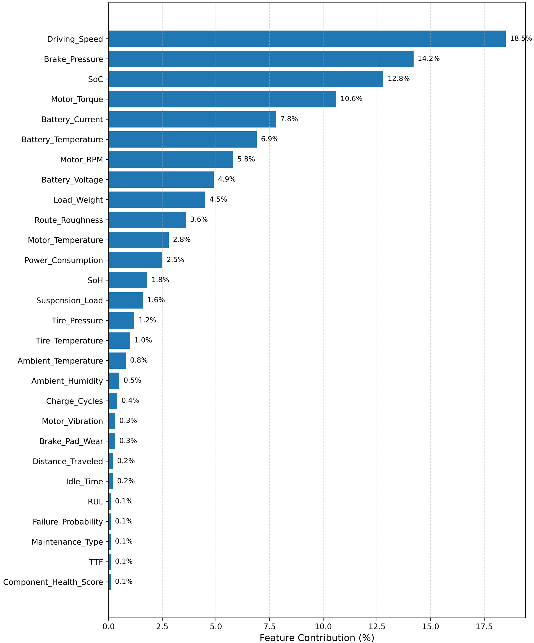
Feature Importance Analysis for Regenerative Braking Efficiency Prediction
