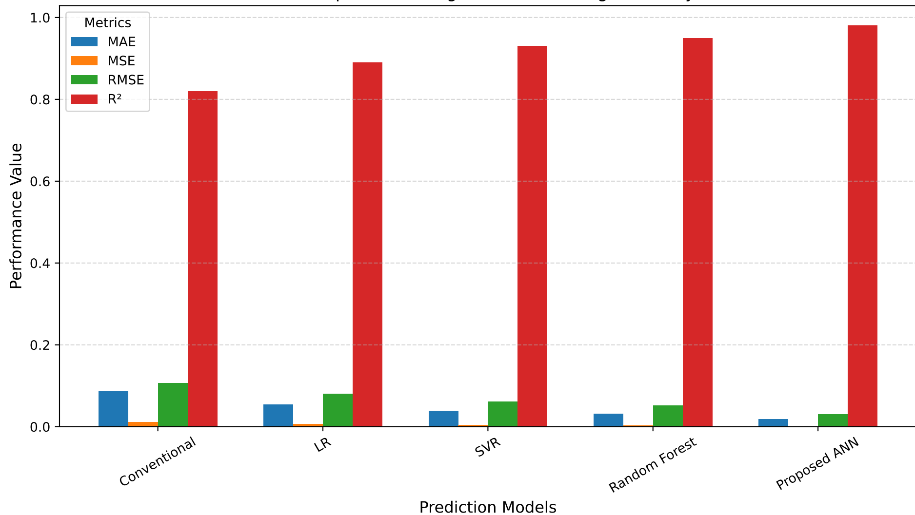
Performance Metric Comparison of Regenerative Braking Efficiency Prediction Models
