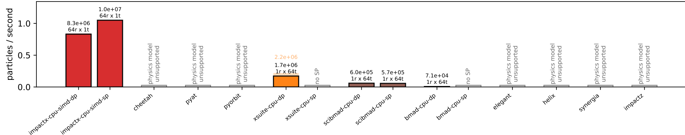
HTU beamline (spin depolarization) · CPU (n = 1,000,000 particles, FP32/FP64) — ref: impactx
