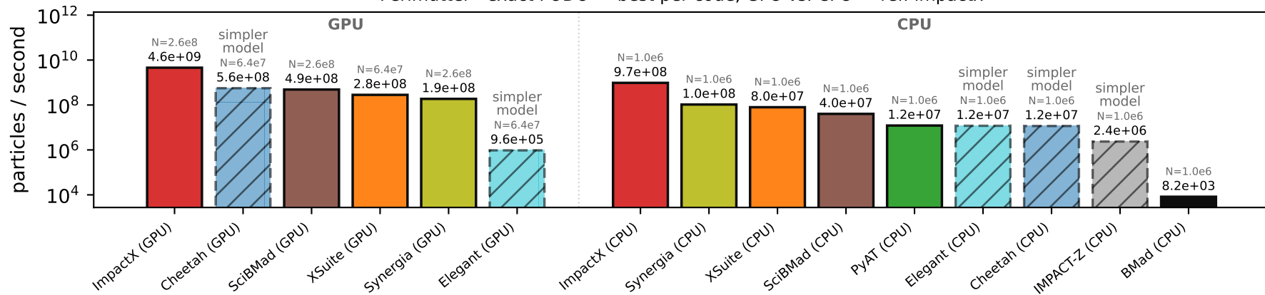
Perlmutter · exact FODO — best per code, GPU vs. CPU — ref: impactx
