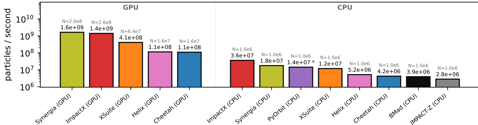
Perlmutter · 3D space charge — best per code, GPU vs. CPU — ref: impactx
