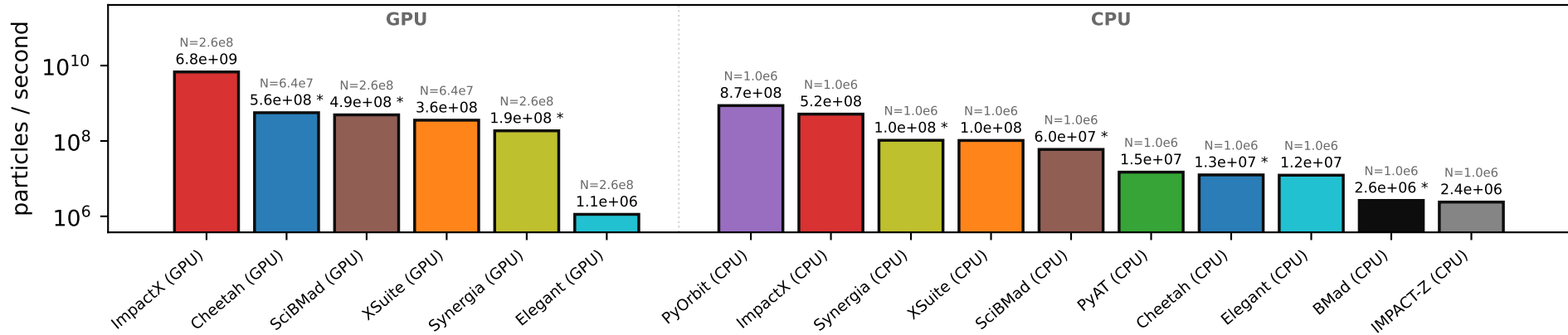
Perlmutter · chromatic FODO — best per code, GPU vs. CPU — ref: impactx
