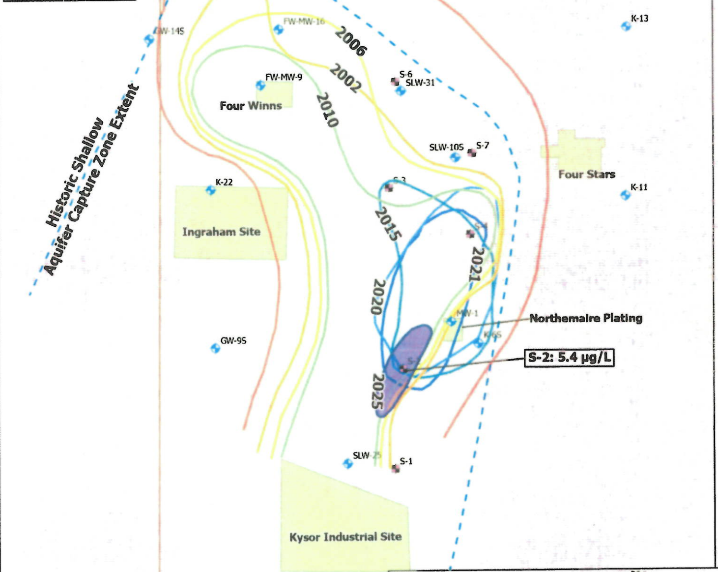
KYSOR SITE CADILLAC, WEXFORD COUNTY, MICHIGAN INTERIM SAMPLING EVENT 2025 FIGURE 4: EXTENT OF TRICHLOROETHENE EXCEEDING THE PAL IN THE SHALLOW AQUIFER FROM 1998-2025
