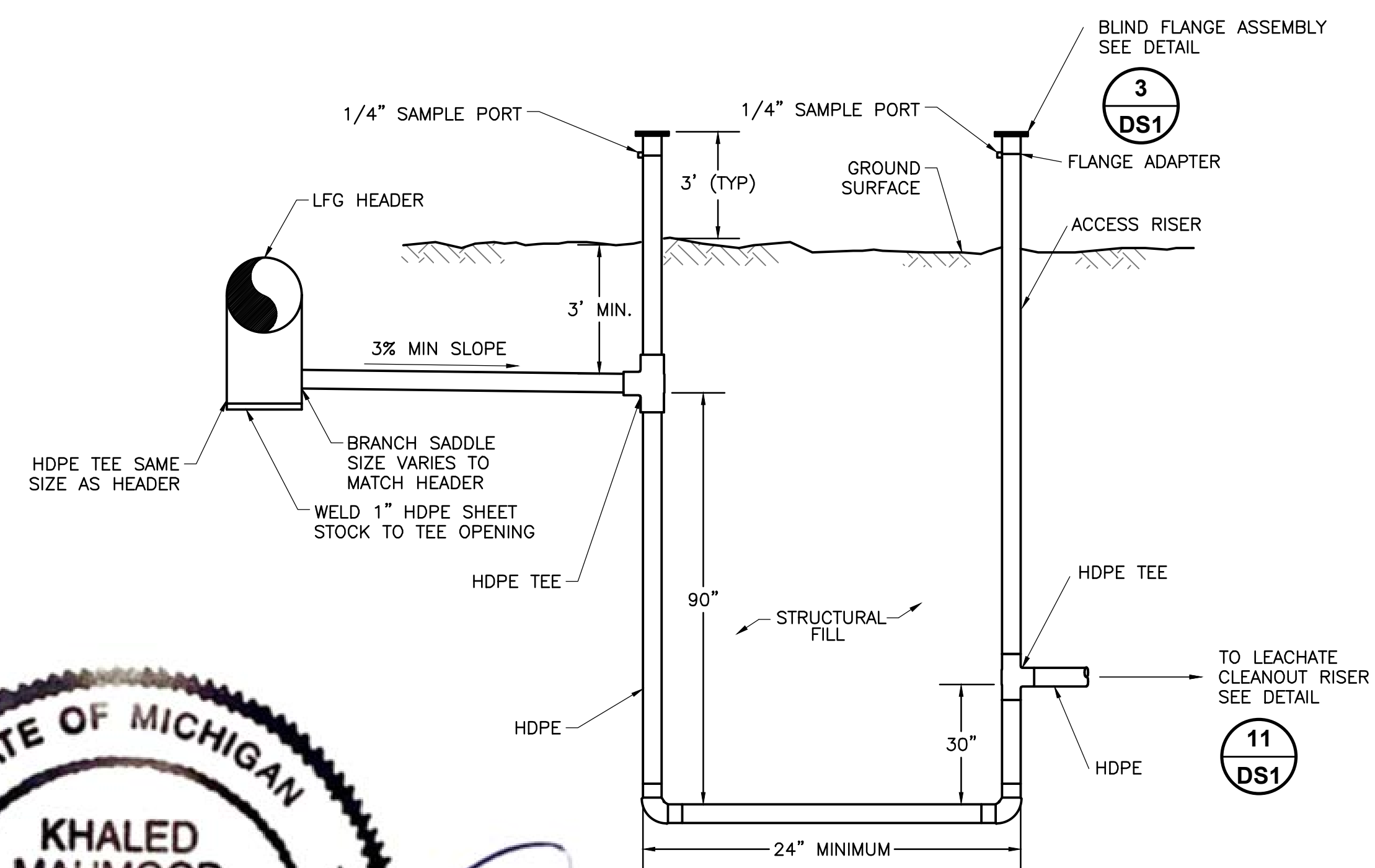
CONDENSATE DRIPLEG
