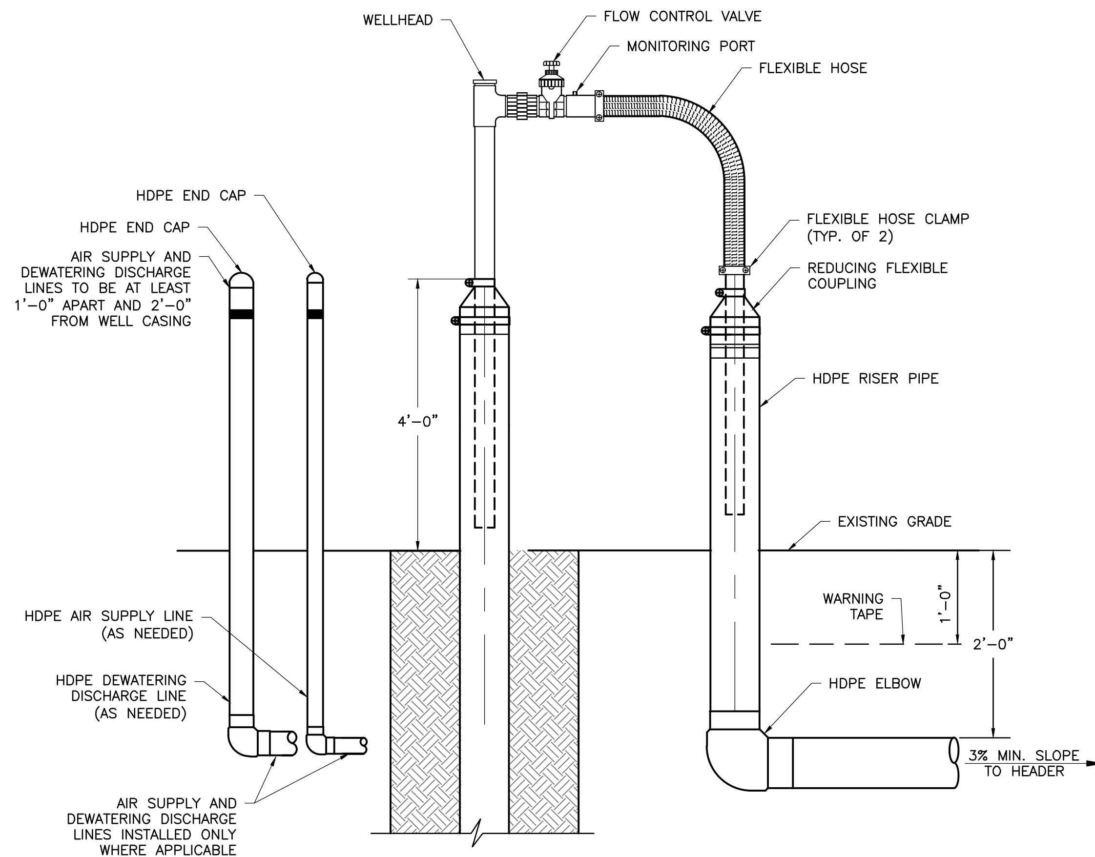
WELLHEAD DETAIL 8 SCALE: NOT TO SCALE DS1
