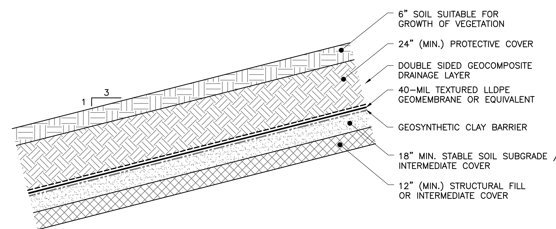
TYPICAL FINAL COVER
