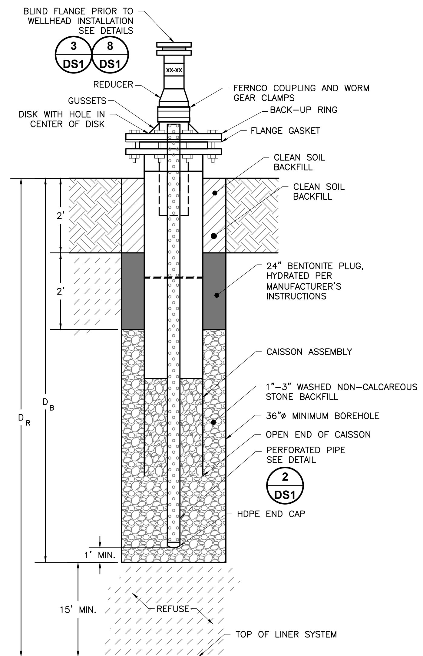
LFG EXTRACTION WELL WITH CAISSON
