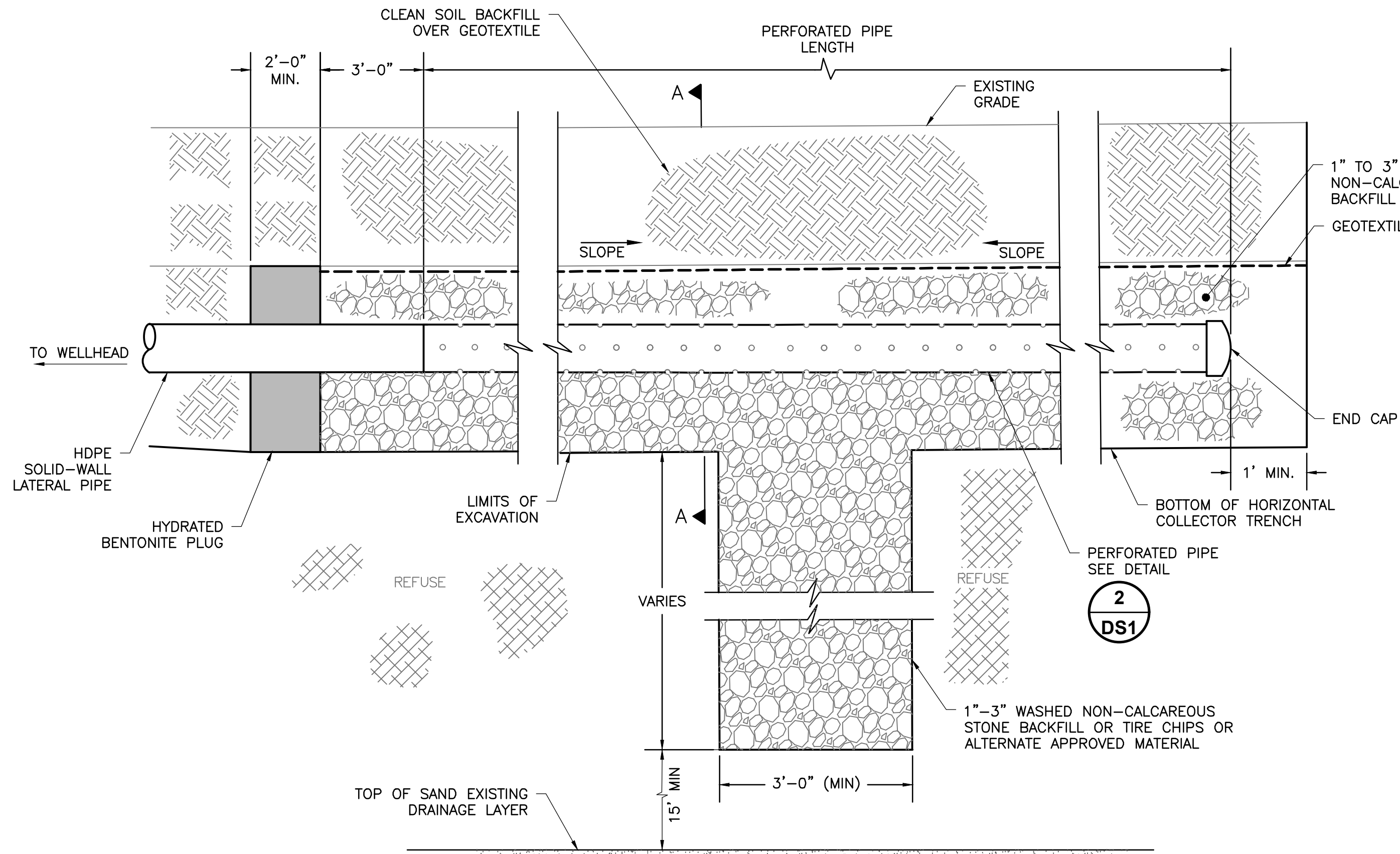
INTERIM HORIZONTAL COLLECTOR
