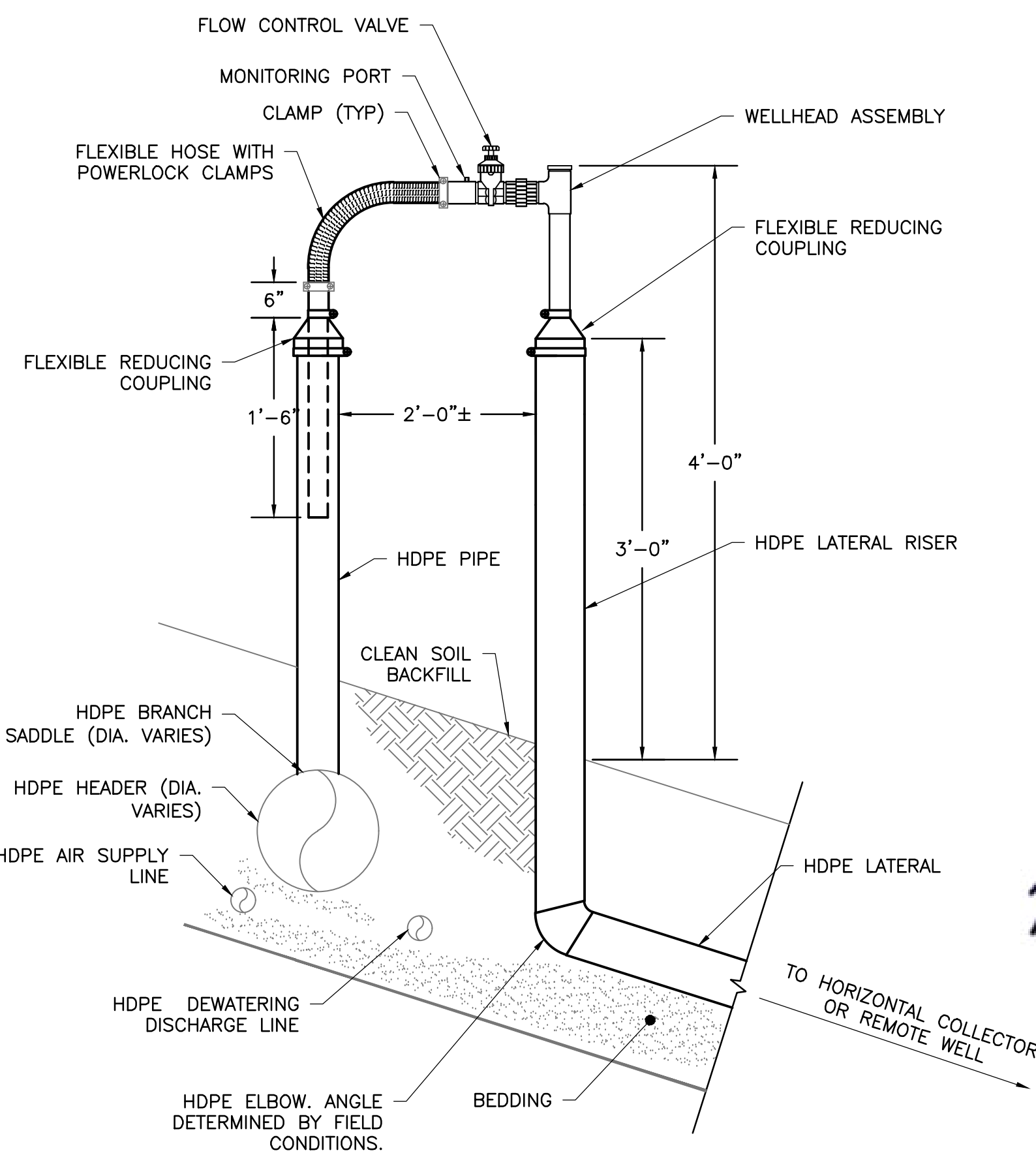
REMOTE WELLHEAD
