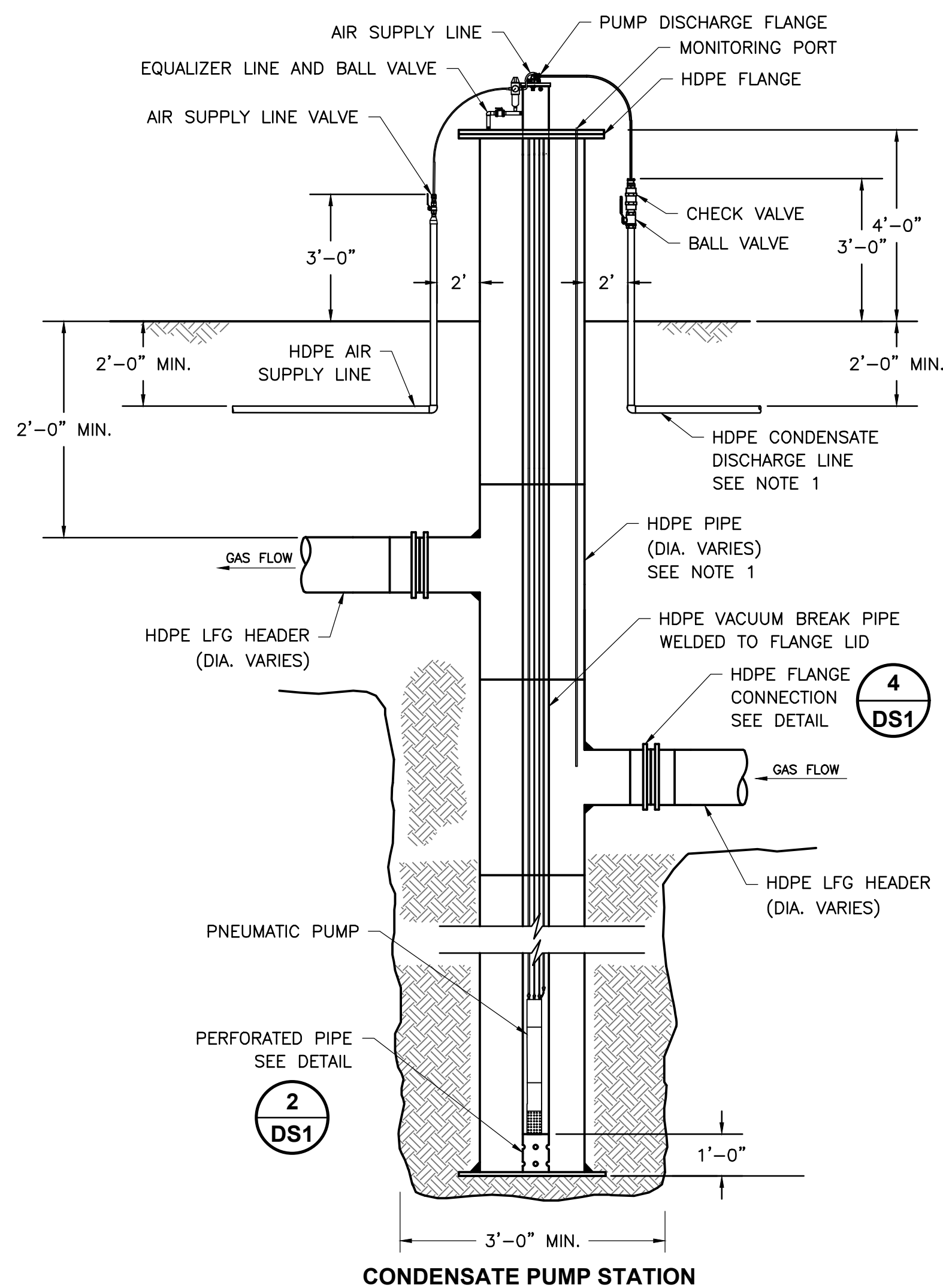
CONDENSATE PUMP STATION
