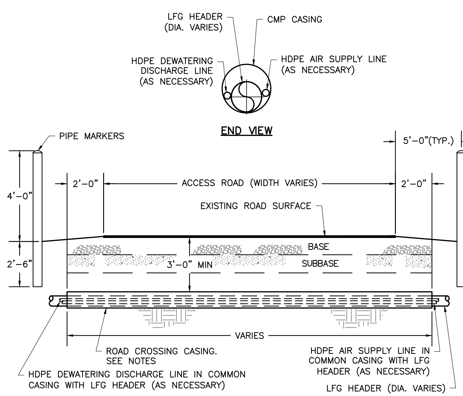
TRENCHED ROAD CROSSING
