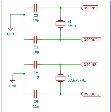
Oscillators
