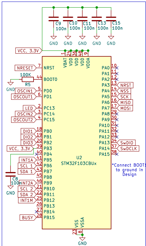
Microcontroller
