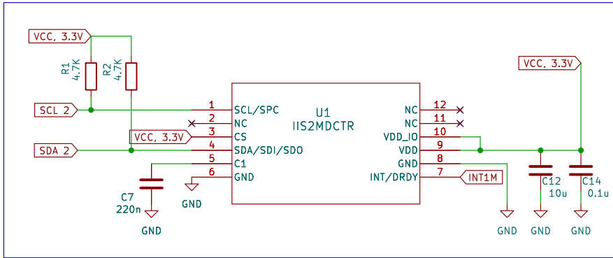
Magnetometer
