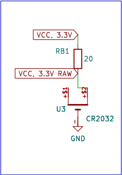
Power Supply
