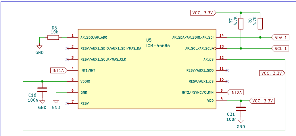
Accelerometer
