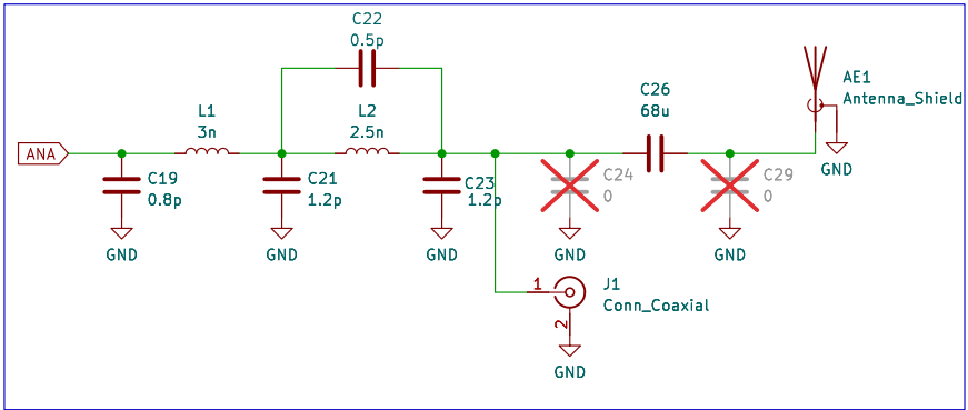
Antenna Frontend
