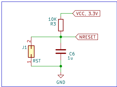
Reset Mechanism
