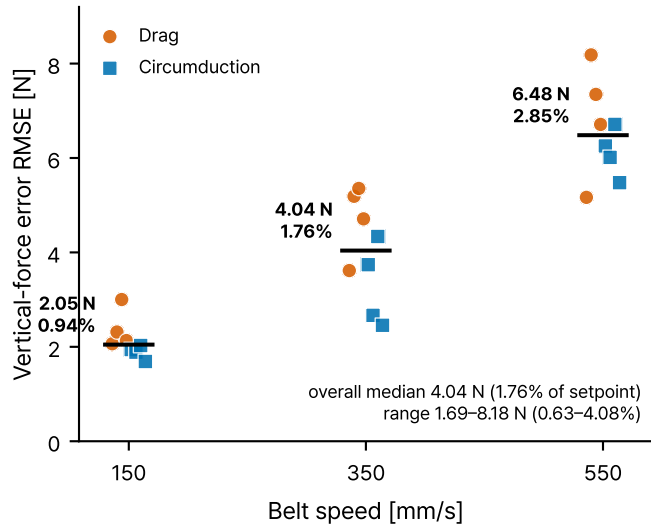
(B) Vertical support tracking, ILC enabled all 24 trials after the 24-s warm-up
