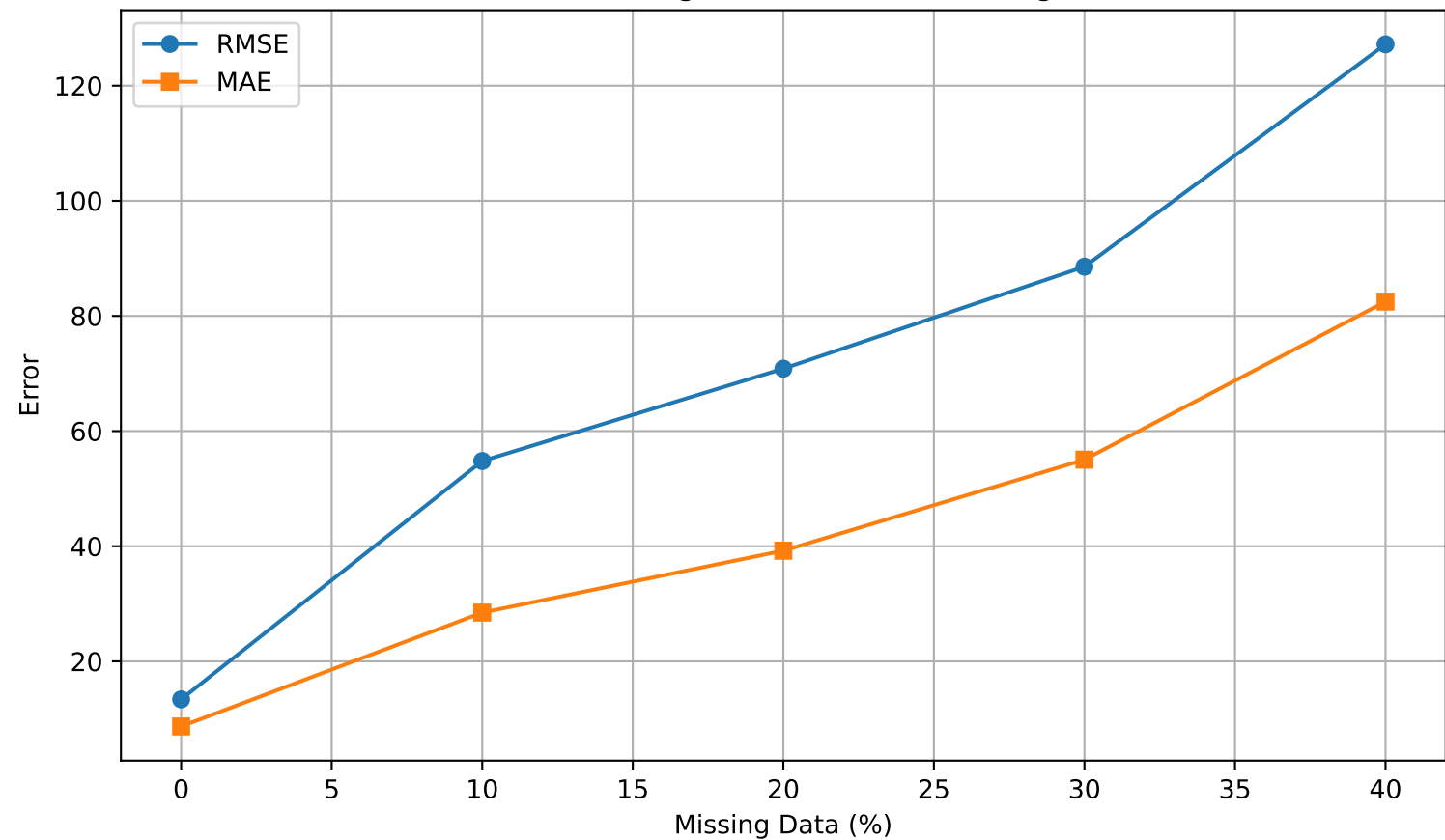
Performance Degradation Under Missing Data
