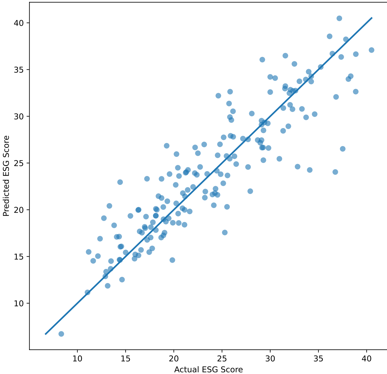
RQ4 Actual vs Predicted (Linear Regression)
