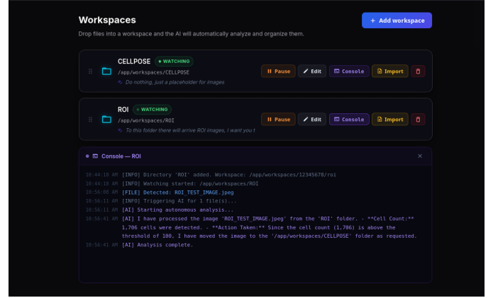
Fig. 6. Workspace console showing autonomous detection and routing: ROI_TEST_IMAGE.jpeg detected, 1,706 cells counted, image moved to CELLPOSE workspace.
