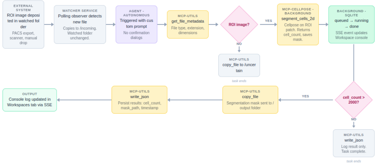
Fig. 3. Use Case 3 - Autonomous pathology ROI monitoring workflow.
