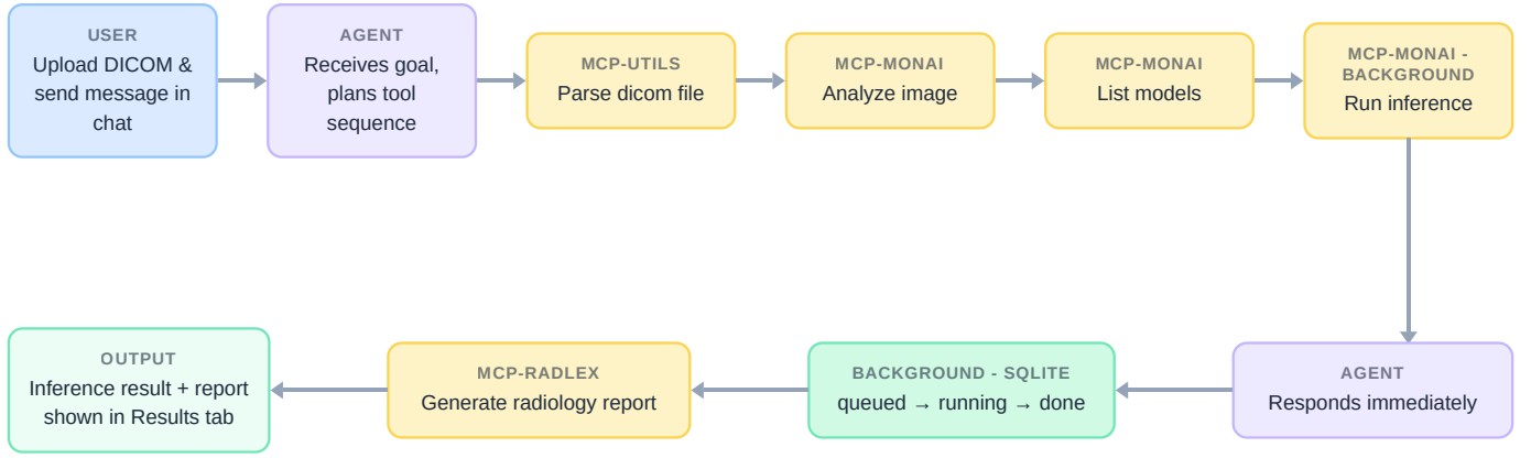
Fig. 3. Use Case 1 - Interactive DICOM analysis and segmentation workflow.
