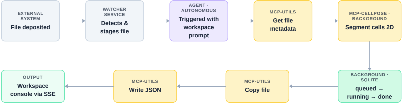
Fig. 4. Use Case 3 - Autonomous pathology ROI monitoring workflow.
