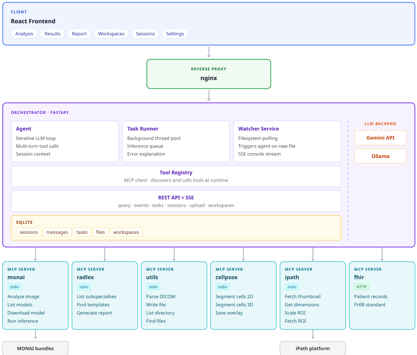
Fig. 1. MedGov-AI system architecture.
